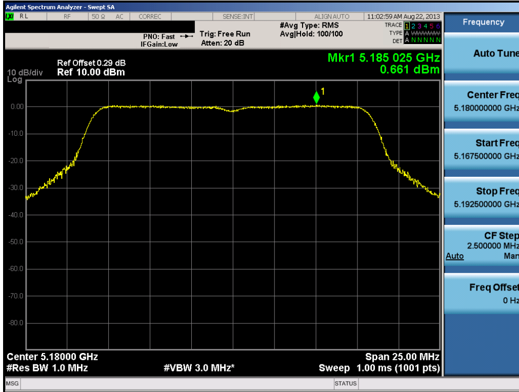
Plot 6-28. Peak Power Spectral Density Plot (802.11a (UNII Band 1) – Ch. 36)
