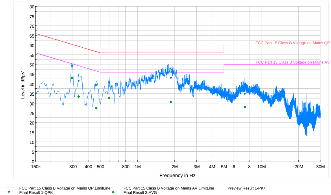
Plot 6-70. Line Conducted Plot with 802.11a UNII Band 1 (L1)
