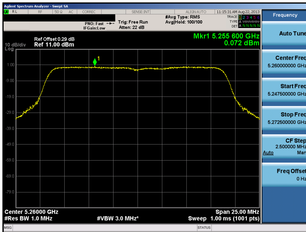
Plot 6-39. Peak Power Spectral Density Plot (20MHz BW 802.11n (UNII Band 2) – Ch. 52)
