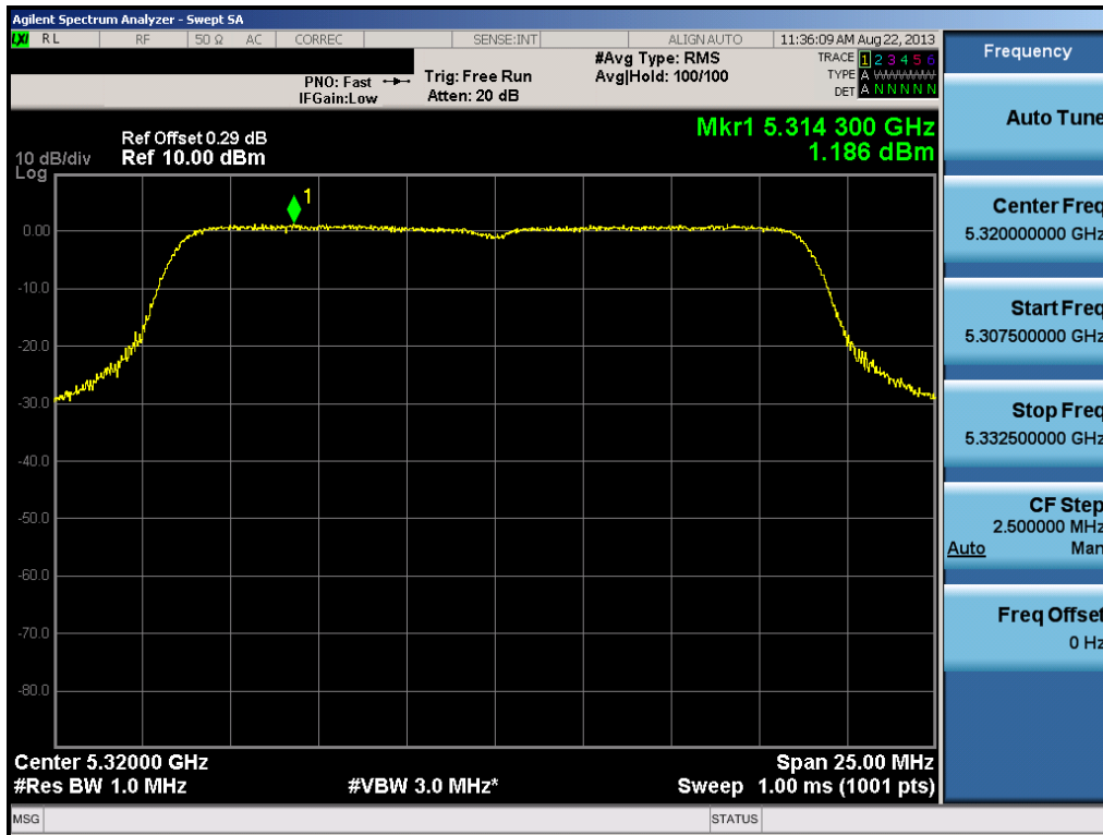
Plot 6-41. Peak Power Spectral Density Plot (20MHz BW 802.11n (UNII Band 2) – Ch. 64)
