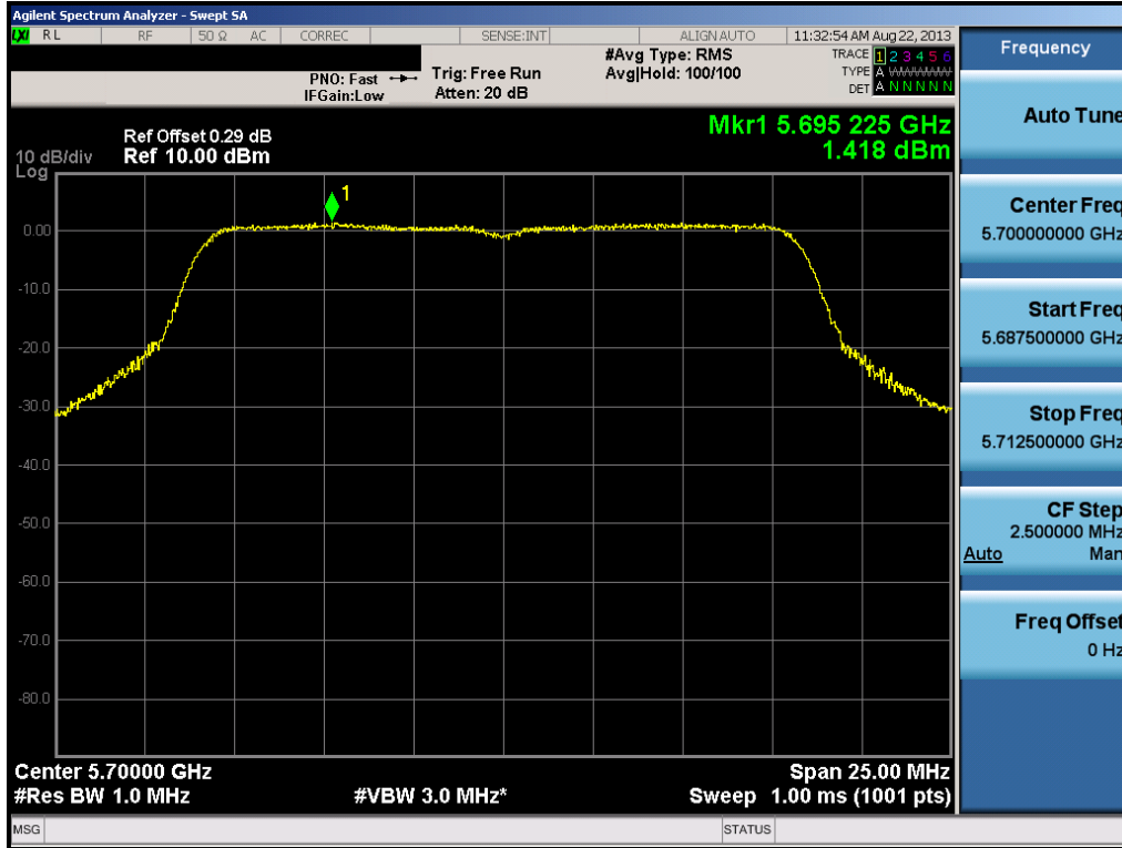
Plot 6-46. Peak Power Spectral Density Plot (802.11a (UNII Band 3) – Ch. 140)
