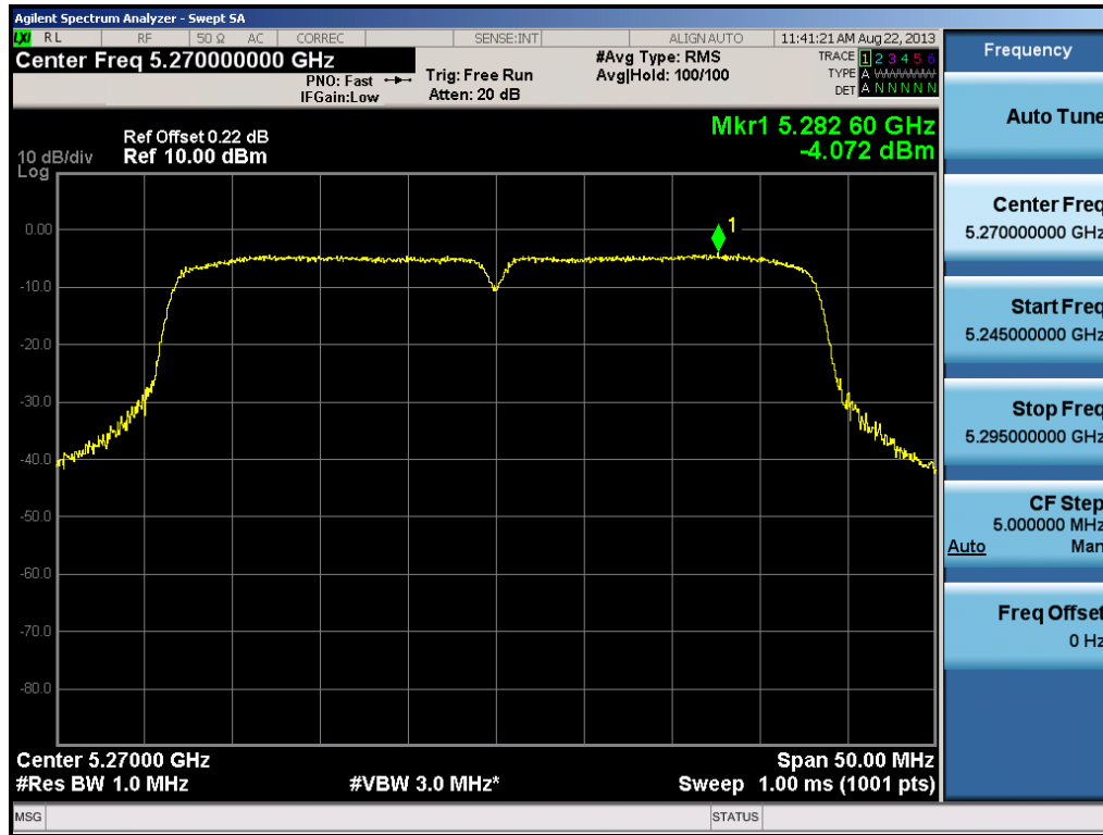
Plot 6-42. Peak Power Spectral Density Plot (40MHz BW 802.11n (UNII Band 2) – Ch. 54)
