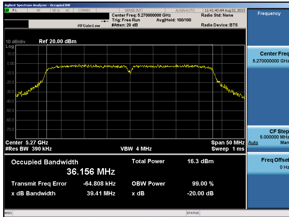
Plot 6-27. 20dB Bandwidth Plot (40MHz BW 802.11n (UNII Band 2) – Ch. 54)
