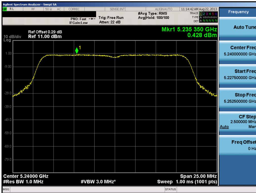
Plot 6-33. Peak Power Spectral Density Plot (20MHz BW 802.11n (UNII Band 1) – Ch. 48)
