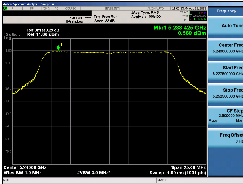
Plot 6-30. Peak Power Spectral Density Plot (802.11a (UNII Band 1) – Ch. 48)
