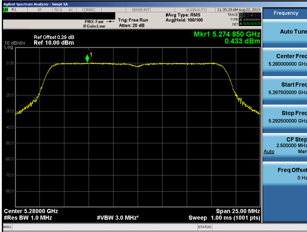
Plot 6-40. Peak Power Spectral Density Plot (20MHz BW 802.11n (UNII Band 2) – Ch. 56)
