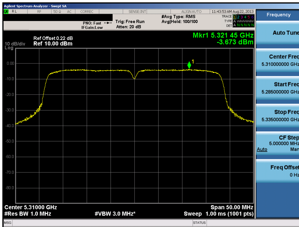
Plot 6-43. Peak Power Spectral Density Plot (40MHz BW 802.11n (UNII Band 2) – Ch. 62)
