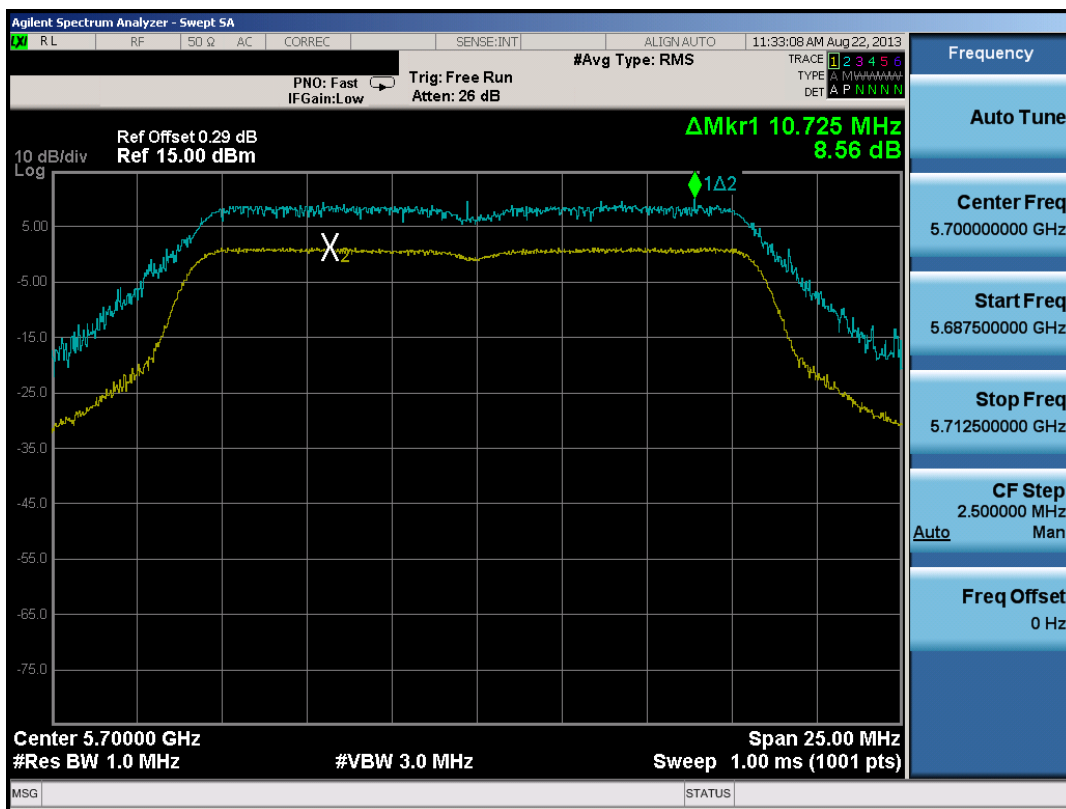
Plot 6-53. Peak Excursion Ratio Plot (802.11a)
