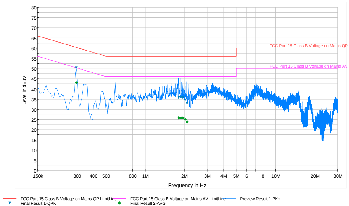
Plot 6-75. Line Conducted Plot with 802.11a UNII Band 3 (N)
