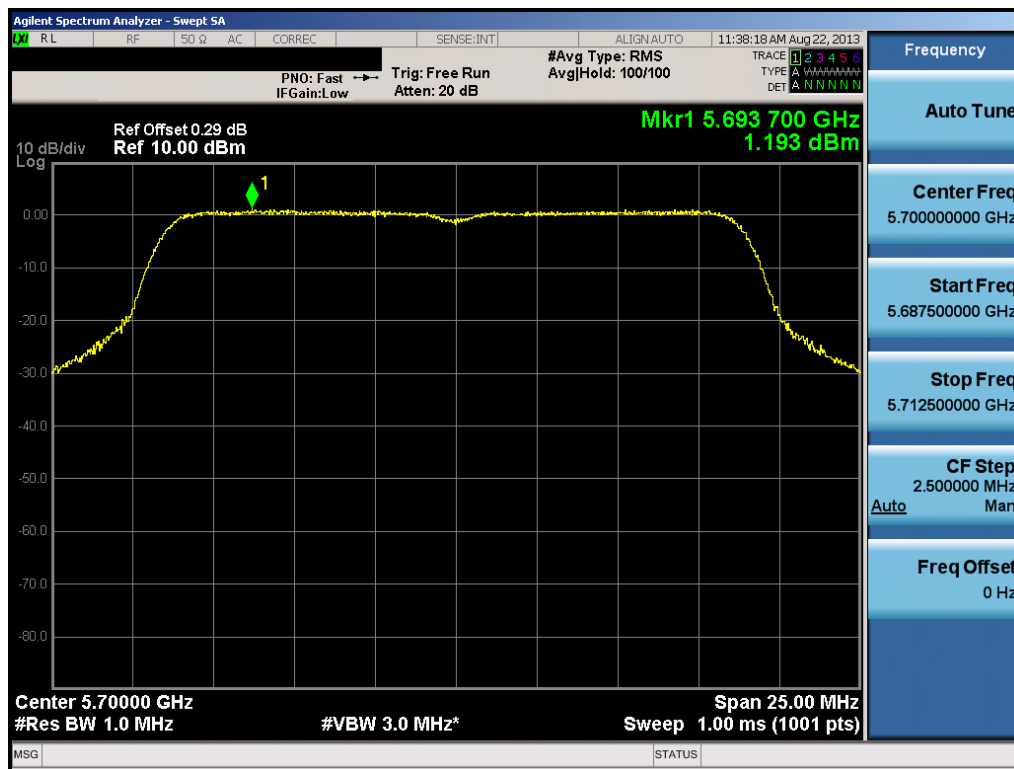
Plot 6-49. Peak Power Spectral Density Plot (20MHz BW 802.11n (UNII Band 3) – Ch. 140)
