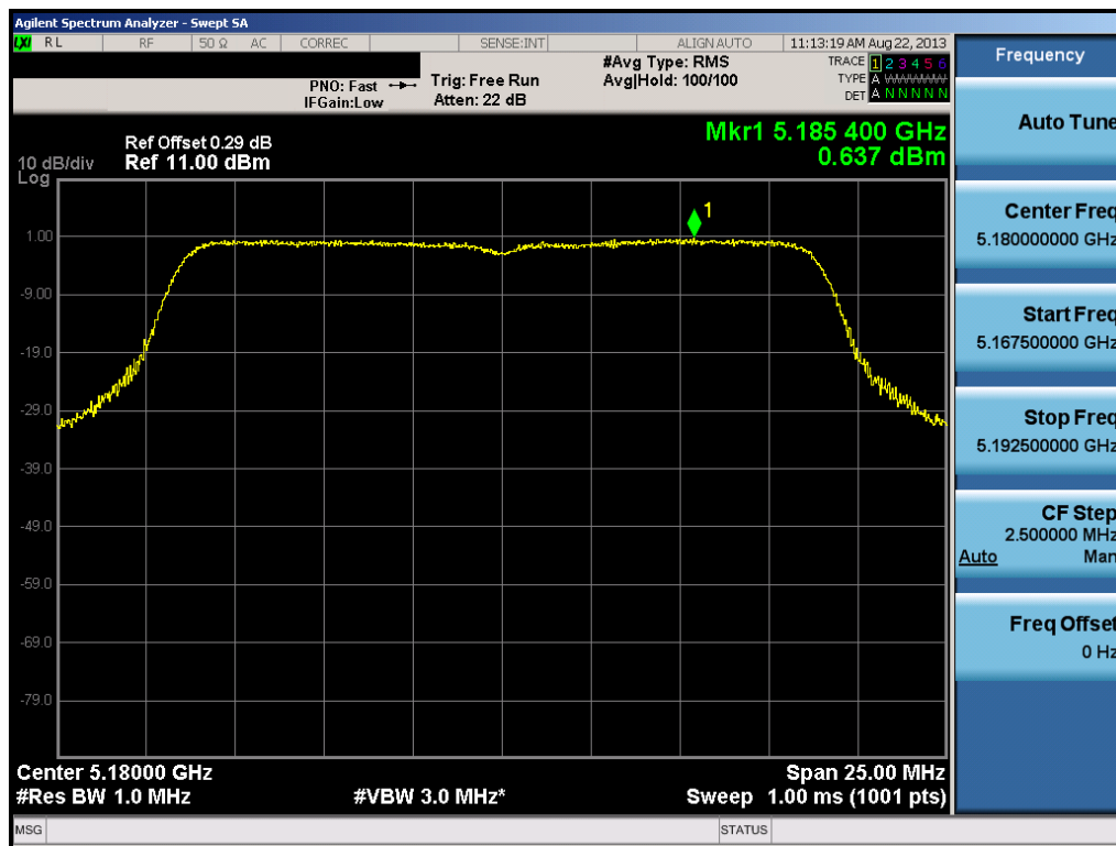
Plot 6-31. Peak Power Spectral Density Plot (20MHz BW 802.11n (UNII Band 1) – Ch. 36)
