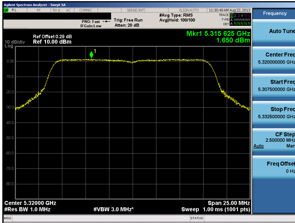
Plot 6-38. Peak Power Spectral Density Plot (802.11a (UNII Band 2) – Ch. 64)
