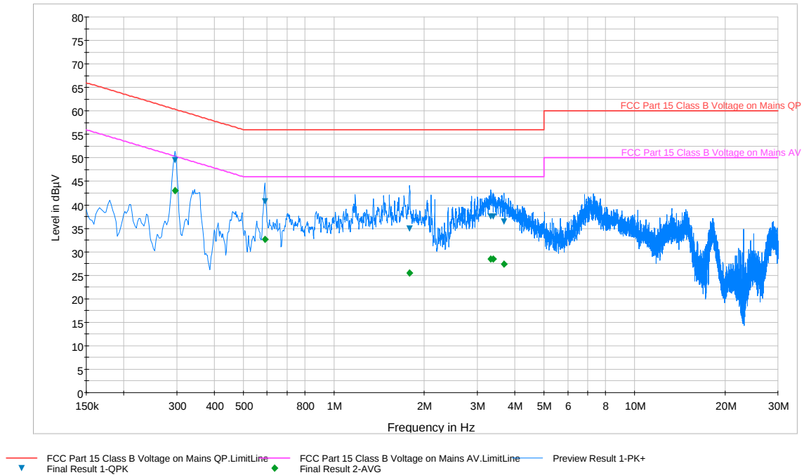
Plot 6-71. Line Conducted Plot with 802.11a UNII Band 1 (N)
