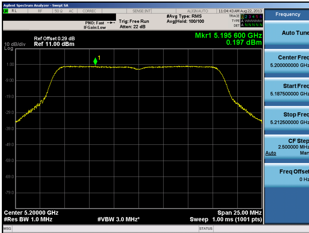
Plot 6-29. Peak Power Spectral Density Plot (802.11a (UNII Band 1) – Ch. 40)
