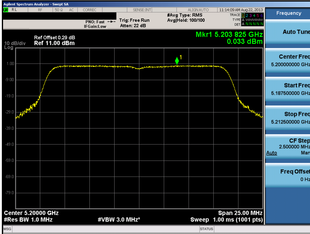
Plot 6-32. Peak Power Spectral Density Plot (20MHz BW 802.11n (UNII Band 1) – Ch. 40)
