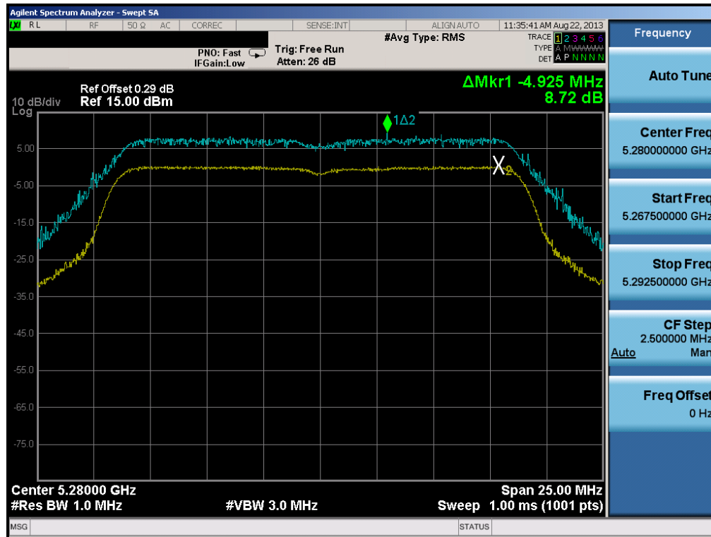
Plot 6-54. Peak Excursion Ratio Plot (20MHz BW 802.11n)
