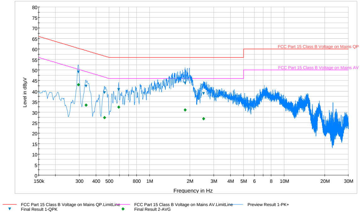
Plot 6-72. Line Conducted Plot with 802.11a UNII Band 2 (L1)
