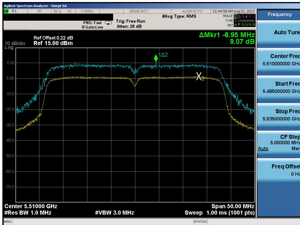
Plot 6-55. Peak Excursion Ratio Plot (40MHz BW 802.11n)
