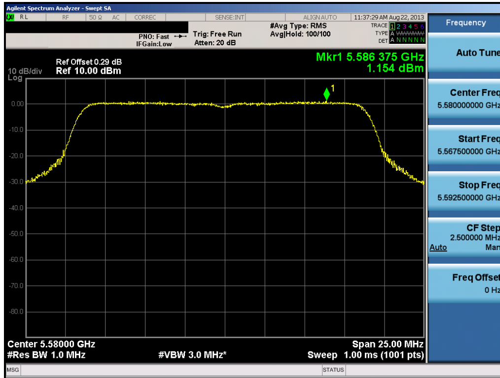
Plot 6-48. Peak Power Spectral Density Plot (20MHz BW 802.11n (UNII Band 3) – Ch. 116)
