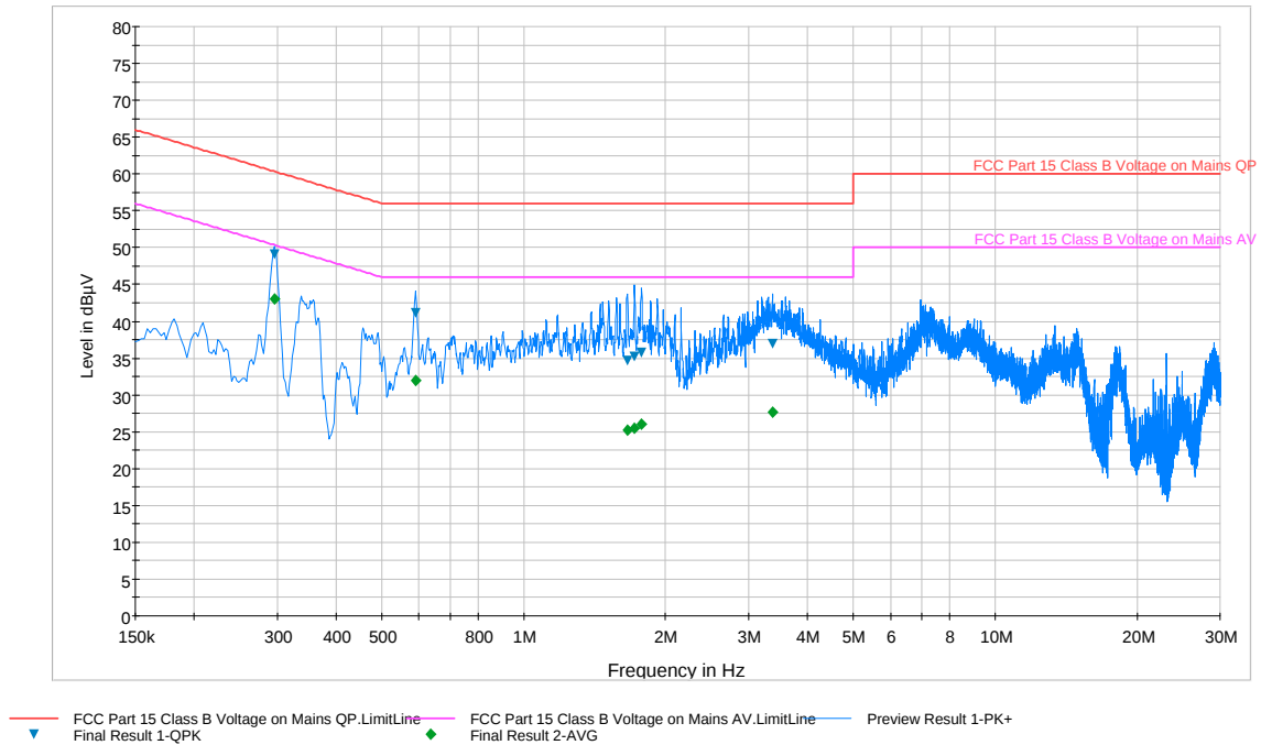
Plot 6-73. Line Conducted Plot with 802.11a UNII Band 2 (N)
