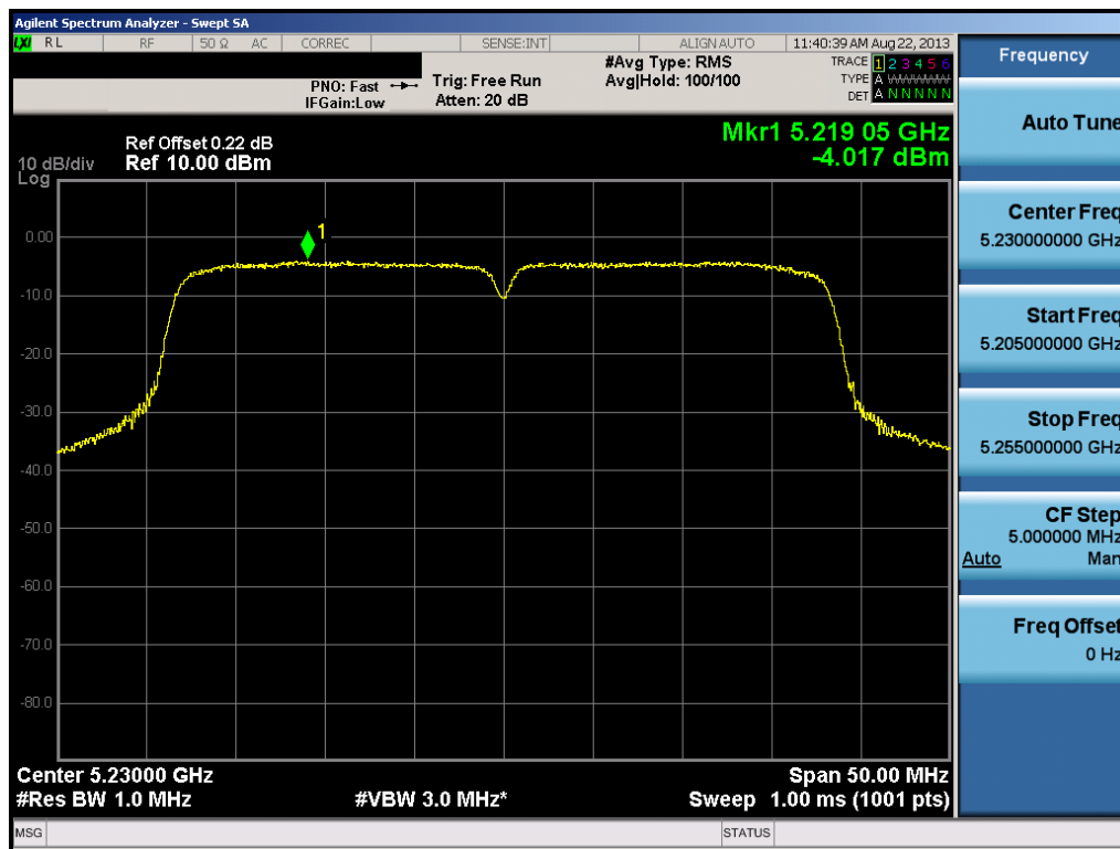
Plot 6-35. Peak Power Spectral Density Plot (40MHz BW 802.11n (UNII Band 1) – Ch. 46)
