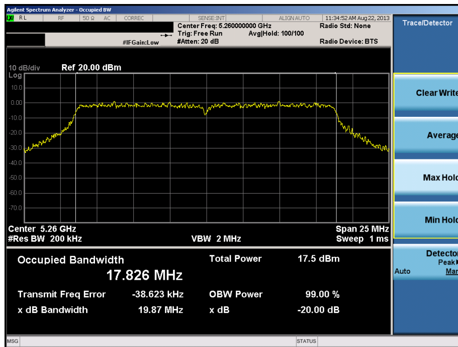
Plot 6-26. 20dB Bandwidth Plot (20MHz BW 802.11n (UNII Band 2) – Ch. 52)
