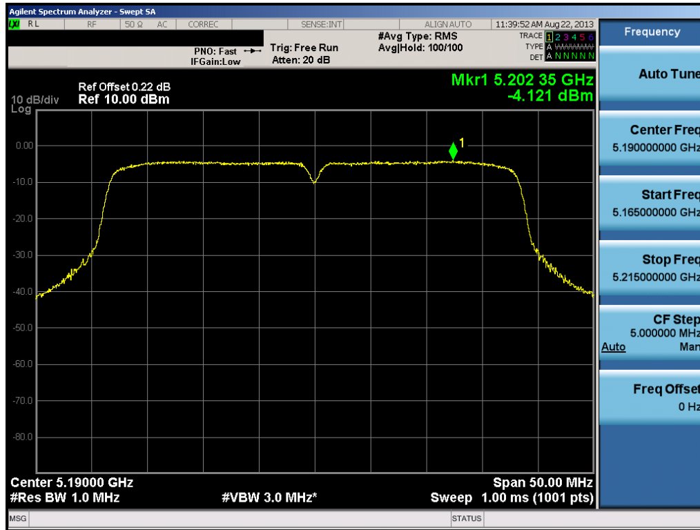
Plot 6-34. Peak Power Spectral Density Plot (40MHz BW 802.11n (UNII Band 1) – Ch. 38)
