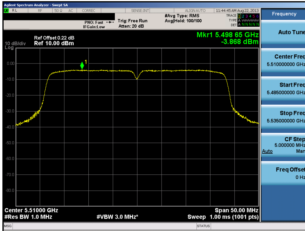
Plot 6-50. Peak Power Spectral Density Plot (40MHz BW 802.11n (UNII Band 3) – Ch. 102)
