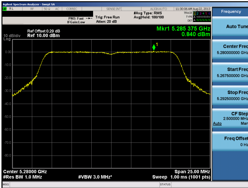
Plot 6-37. Peak Power Spectral Density Plot (802.11a (UNII Band 2) – Ch. 56)
