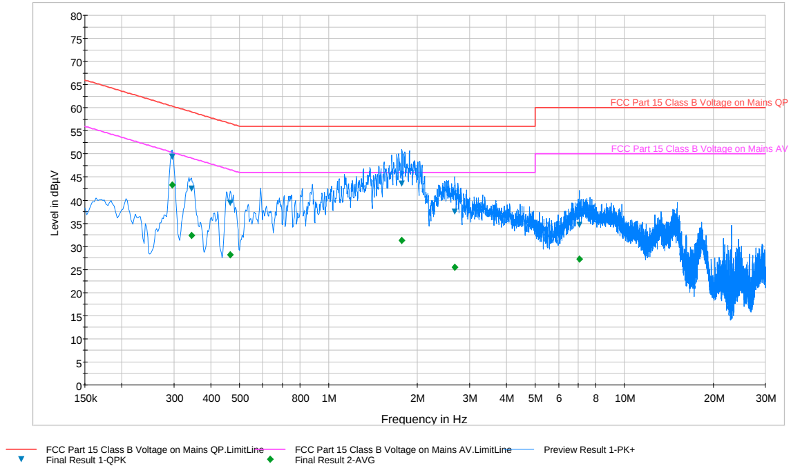
Plot 6-74. Line Conducted Plot with 802.11a UNII Band 3 (L1)
