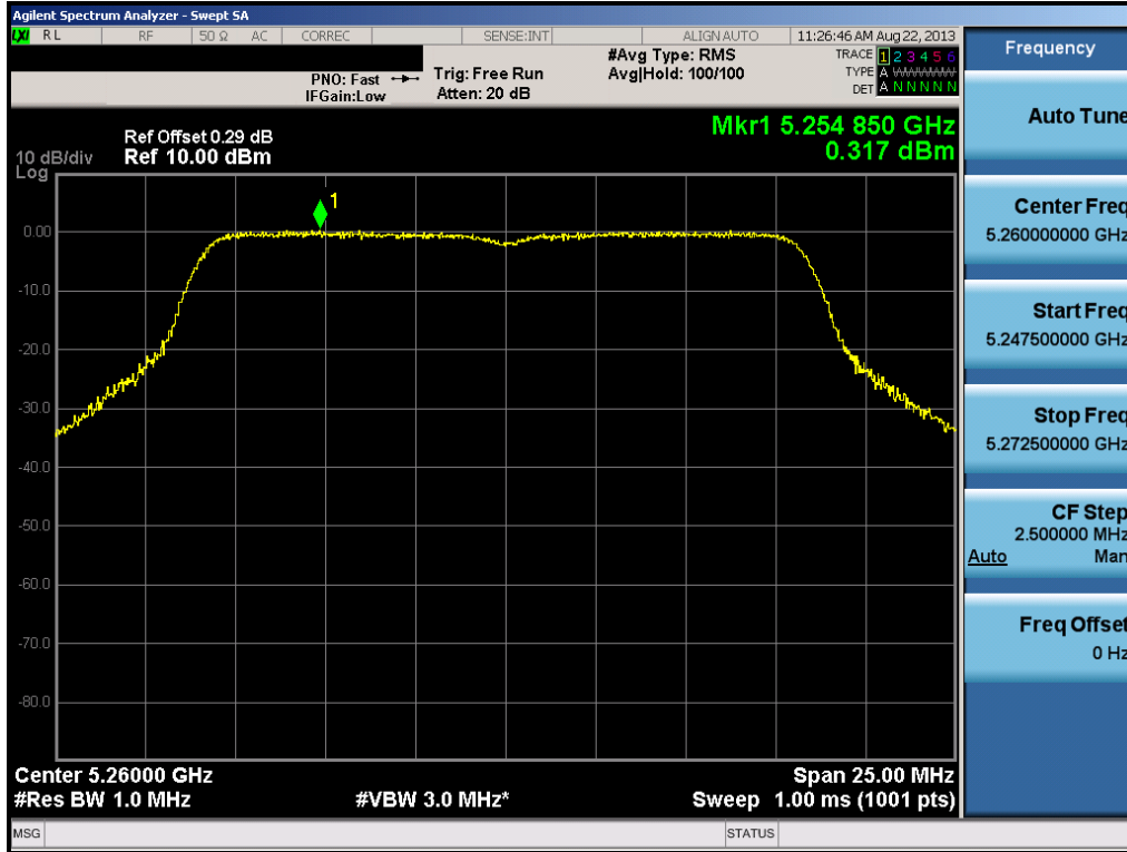
Plot 6-36. Peak Power Spectral Density Plot (802.11a (UNII Band 2) – Ch. 52)
