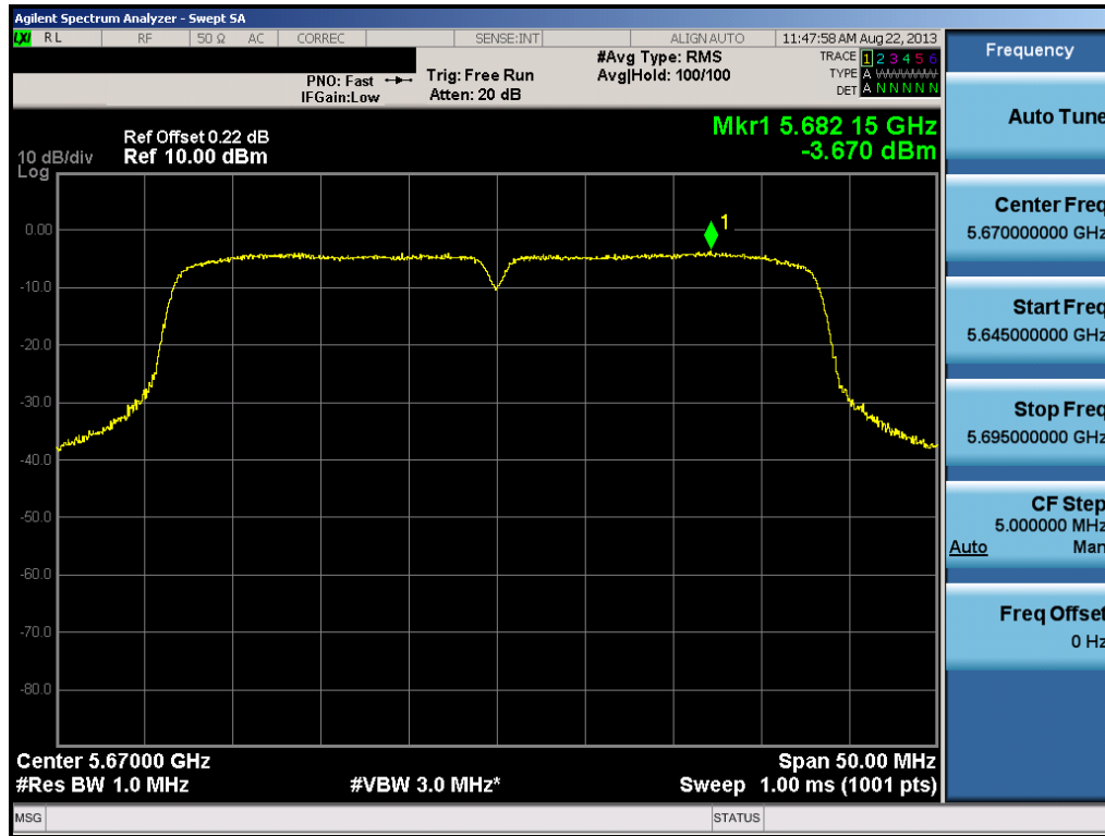
Plot 6-52. Peak Power Spectral Density Plot (40MHz BW 802.11n (UNII Band 3) – Ch. 134)
