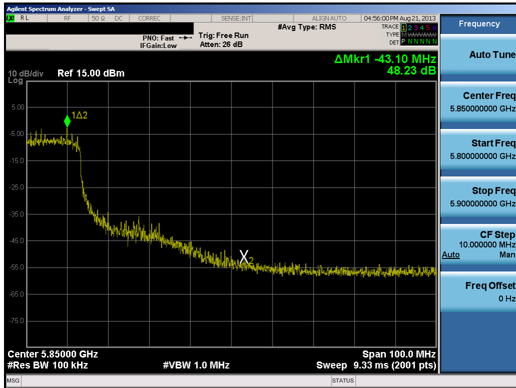
Plot 6-45. Band Edge Plot (40MHz BW 802.11n (5.8GHz) – Ch. 155)
