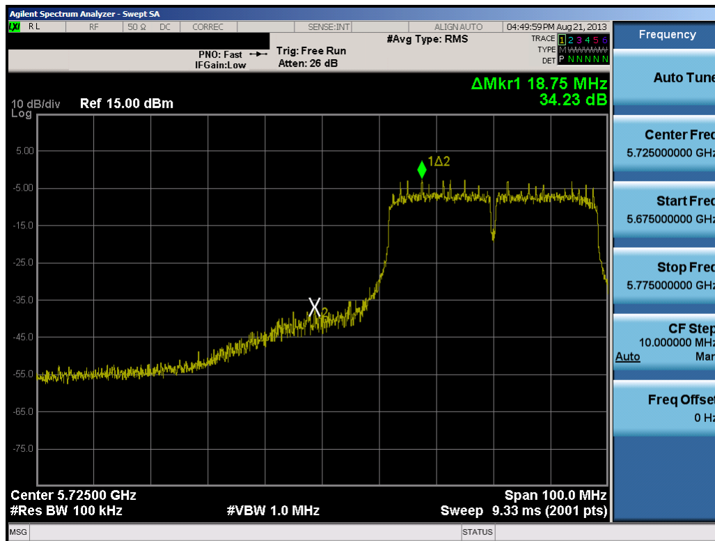
Plot 6-44. Band Edge Plot (40MHz BW 802.11n (5.8GHz) – Ch. 151)
