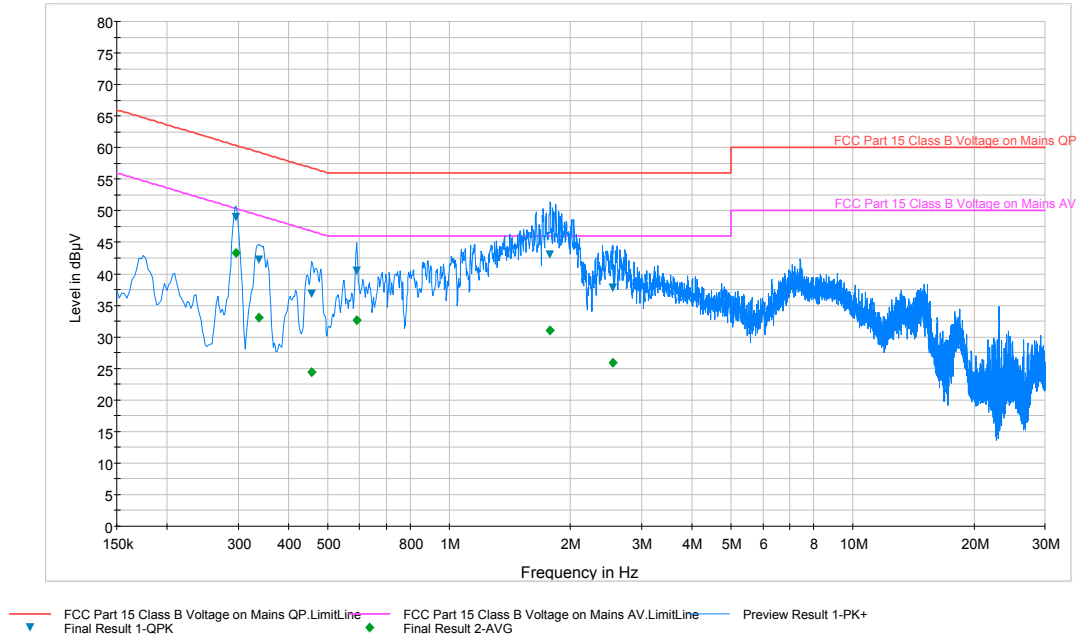
Plot 6-64. Line Conducted Plot with 802.11a (L1)
