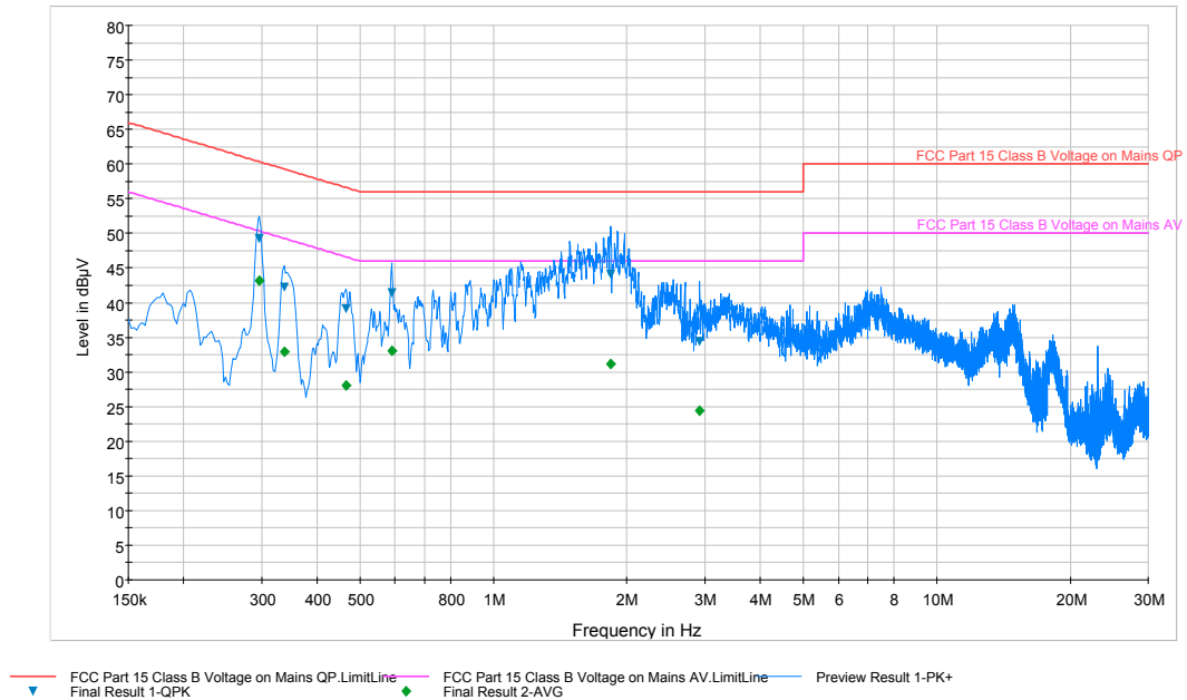
Plot 6-62. Line Conducted Plot with 802.11b (L1)
