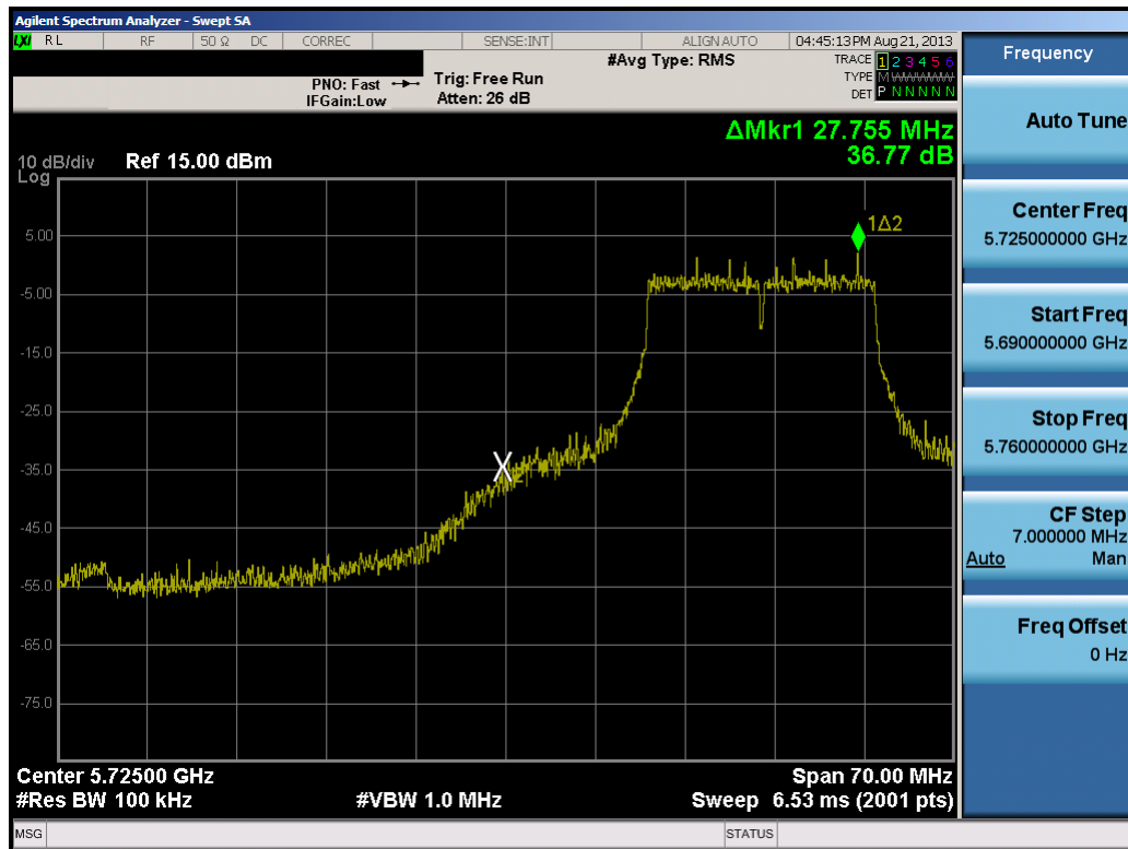
Plot 6-42. Band Edge Plot (20MHz BW 802.11n (5.8GHz) – Ch. 149)
