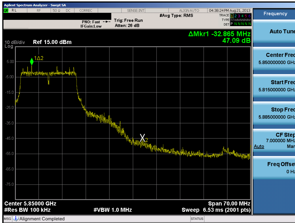
Plot 6-43. Band Edge Plot (20MHz BW 802.11n (5.8GHz) – Ch. 165)
