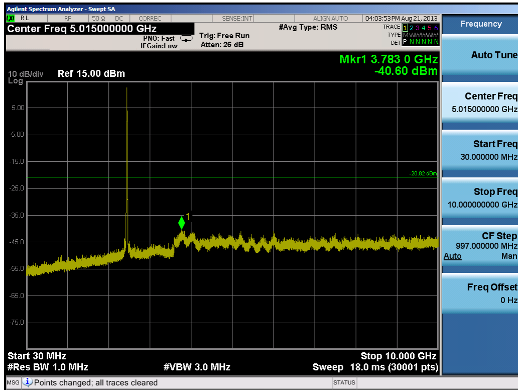
Plot 6-50. Conducted Spurious Plot (802.11b – Ch. 11)
