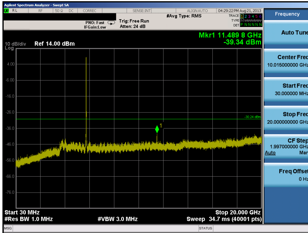
Plot 6-52. Conducted Spurious Plot (802.11a – Ch. 149)
