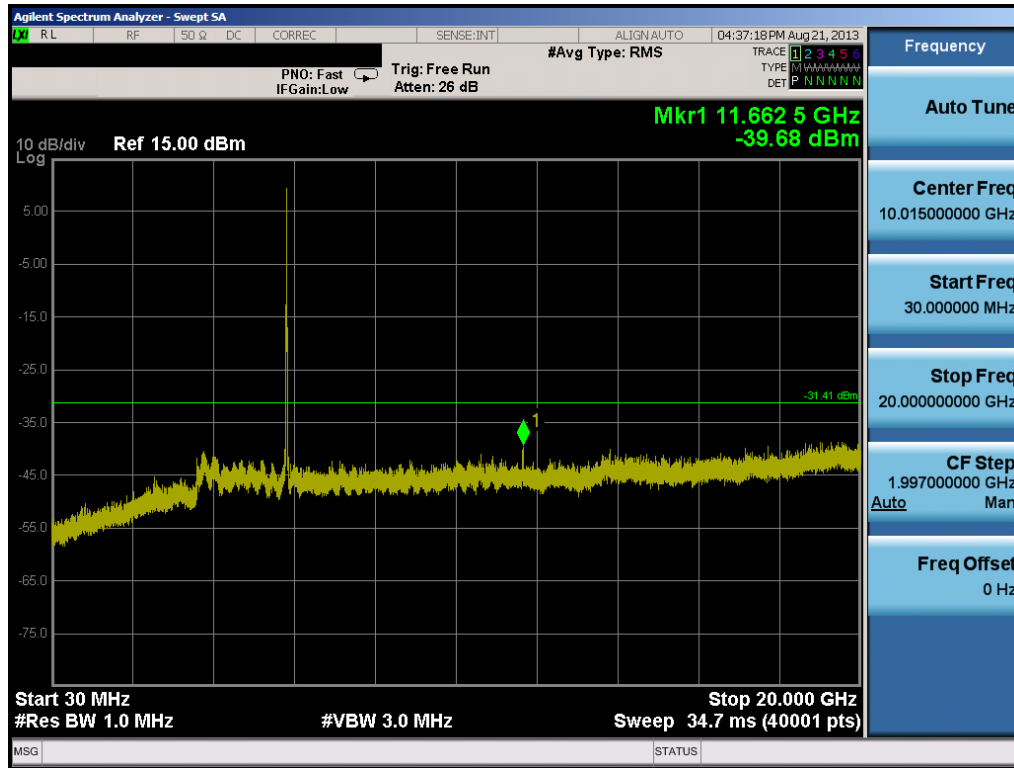
Plot 6-56. Conducted Spurious Plot (802.11a – Ch. 165)
