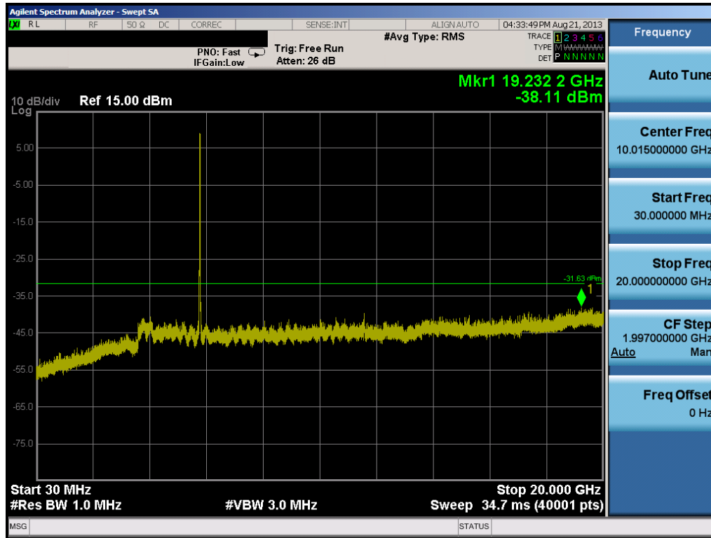
Plot 6-54. Conducted Spurious Plot (802.11a – Ch. 157)
