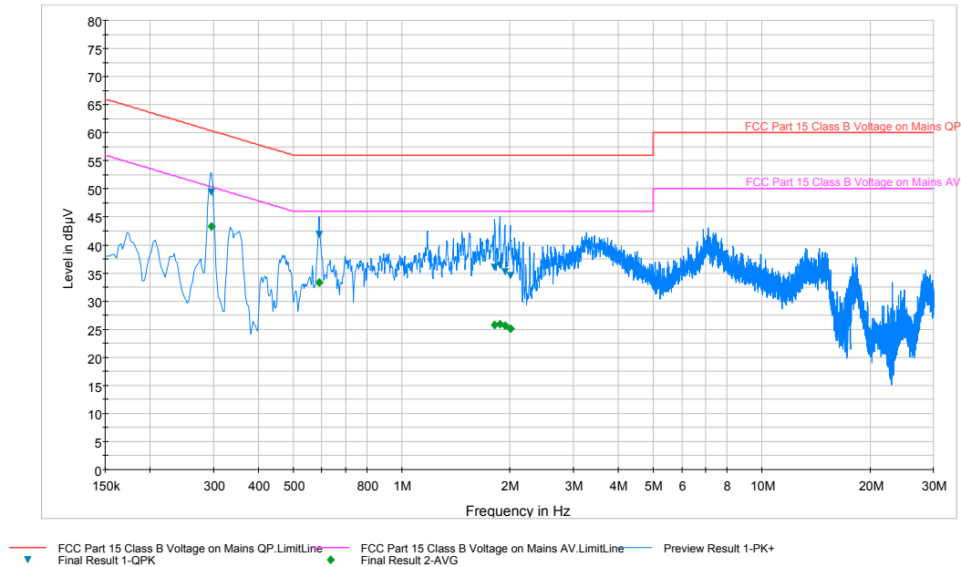
Plot 6-63. Line Conducted Plot with 802.11b (N)
