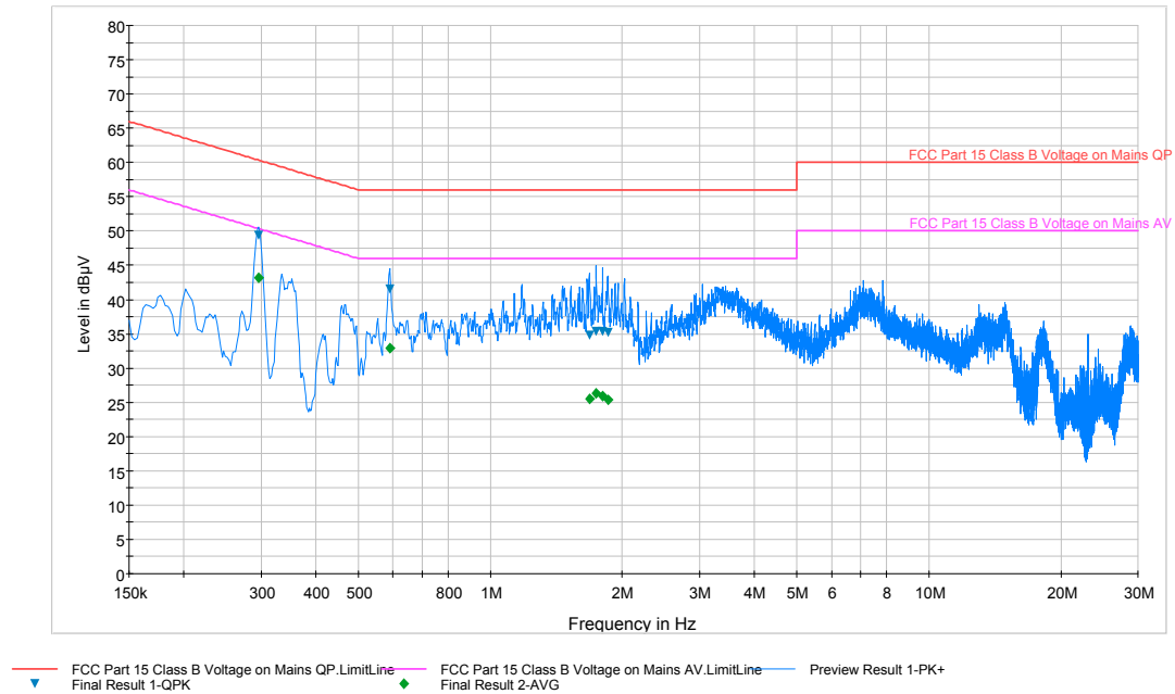
Plot 6-65. Line Conducted Plot with 802.11a (N)
