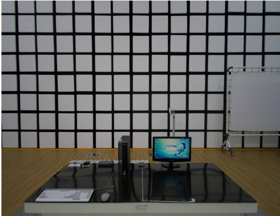
[ Radiated Disturbance for Below 1 GHz – Front ]
