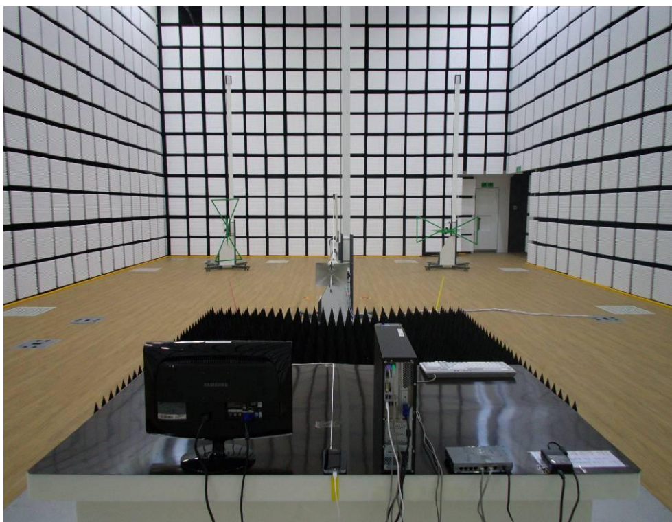
[ Radiated Disturbance for Above 1 GHz – Rear ]
