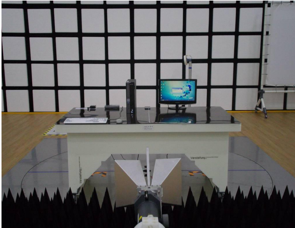
[ Radiated Disturbance for Above 1 GHz – Front ]
