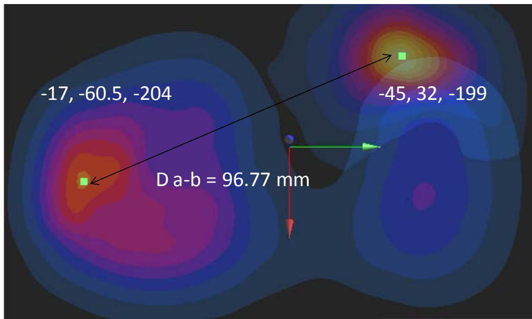
Figure 12-1 Peak SAR Locations of 5.8 GHz WLAN and UMTS 1900
