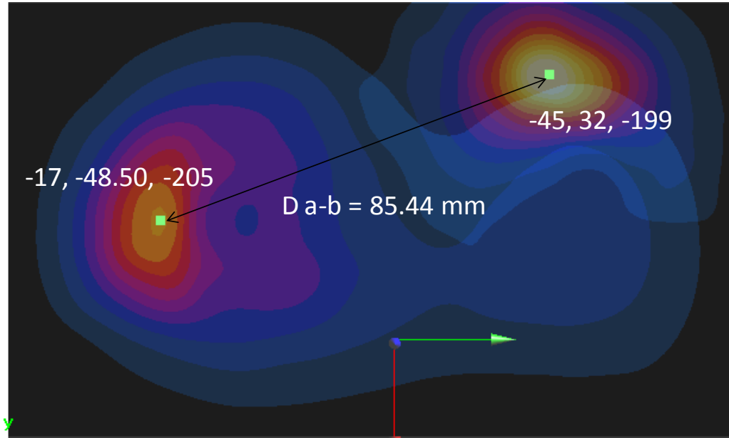
Figure 12-3 Peak SAR Locations of 5.8 GHz WLAN and LTE band 4
