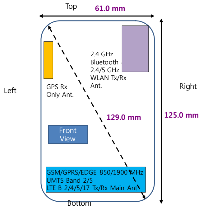
Figure 1-1 DUT Antenna Locations
