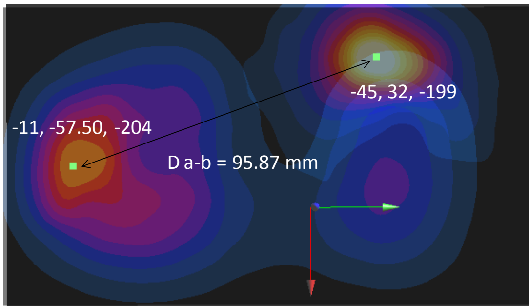
Figure 12-2 Peak SAR Locations of 5.8 GHz WLAN and LTE Band 2
