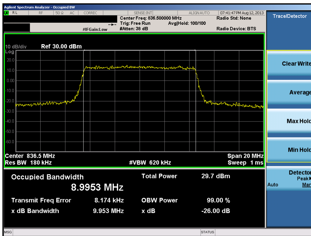
Plot 8-15. Occupied Bandwidth Plot (10.0MHz QPSK – RB Size 50)
