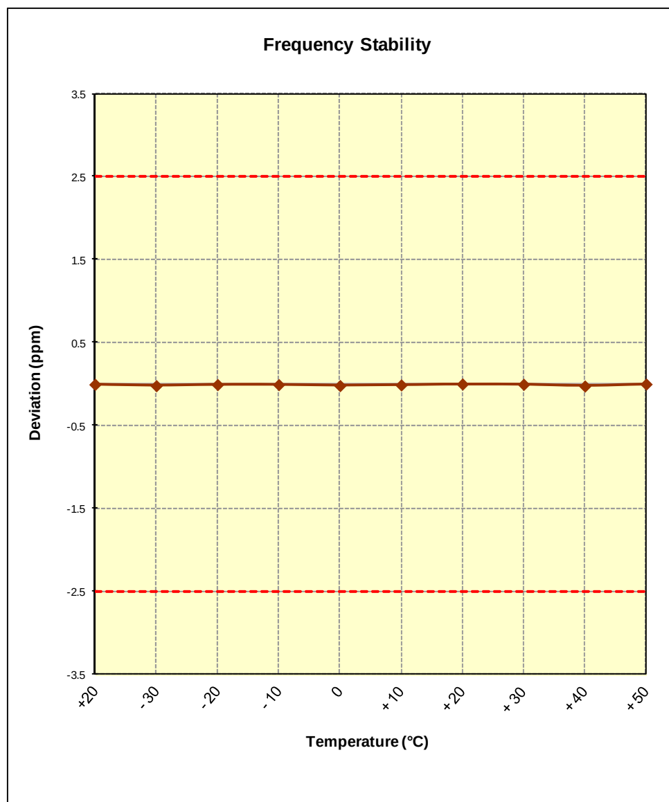
Figure 6-1. Frequency Stability Graph (Band 17)
