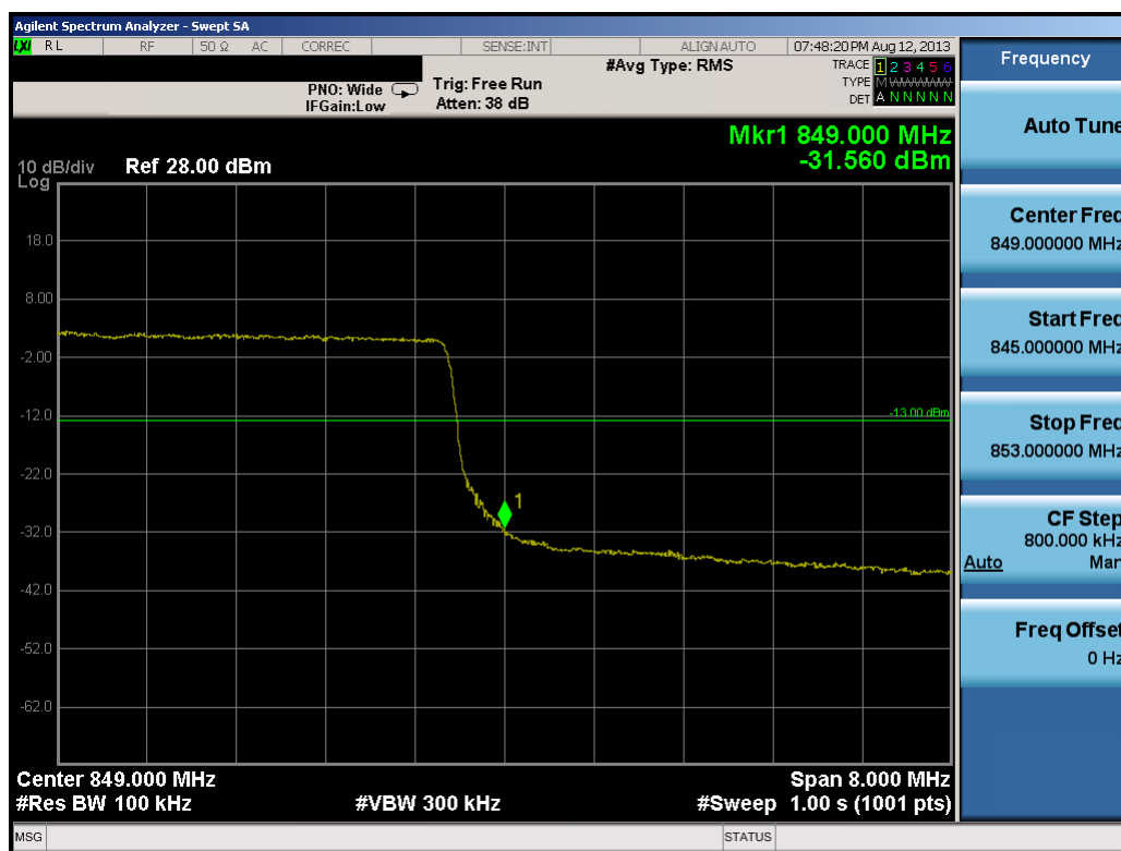
Plot 8-23. Upper Band Edge Plot (10.0MHz QPSK – RB Size 50)
