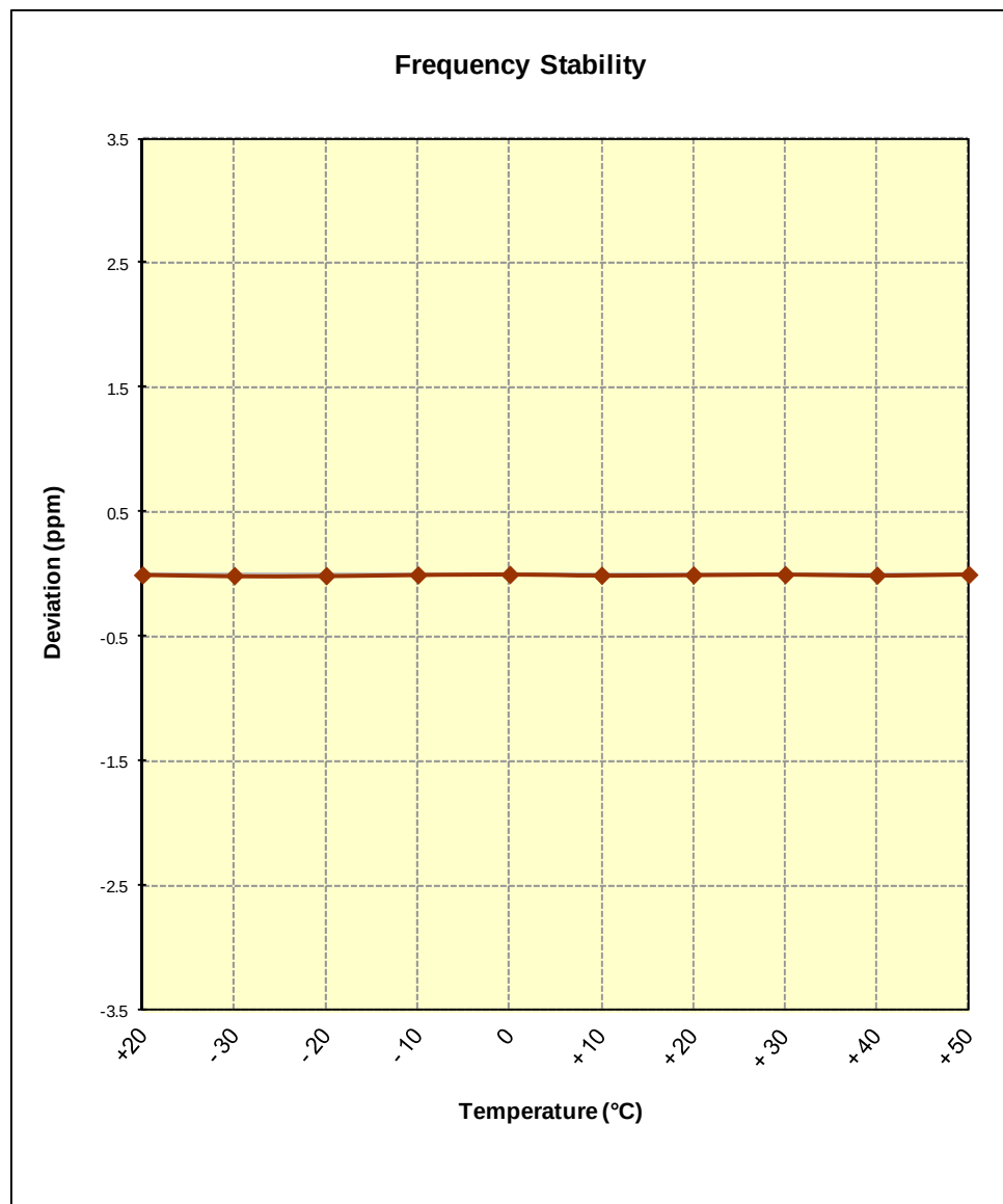
Figure 6-3. Frequency Stability Graph (Band 4)
