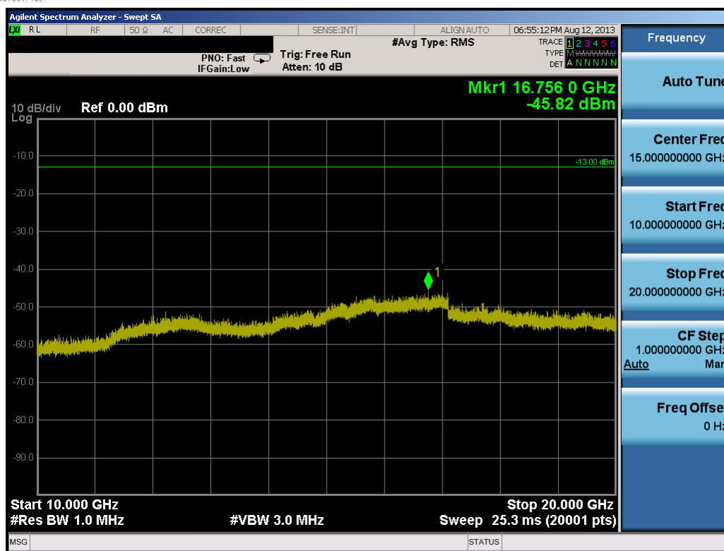
Plot 9-24. Conducted Spurious Plot (10.0MHz QPSK – RB Size 1, RB Offset 0 – High Channel)
