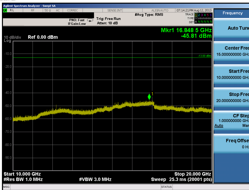
Plot 9-38. Conducted Spurious Plot (15.0MHz QPSK – RB Size 1, RB Offset 0 – High Channel)
