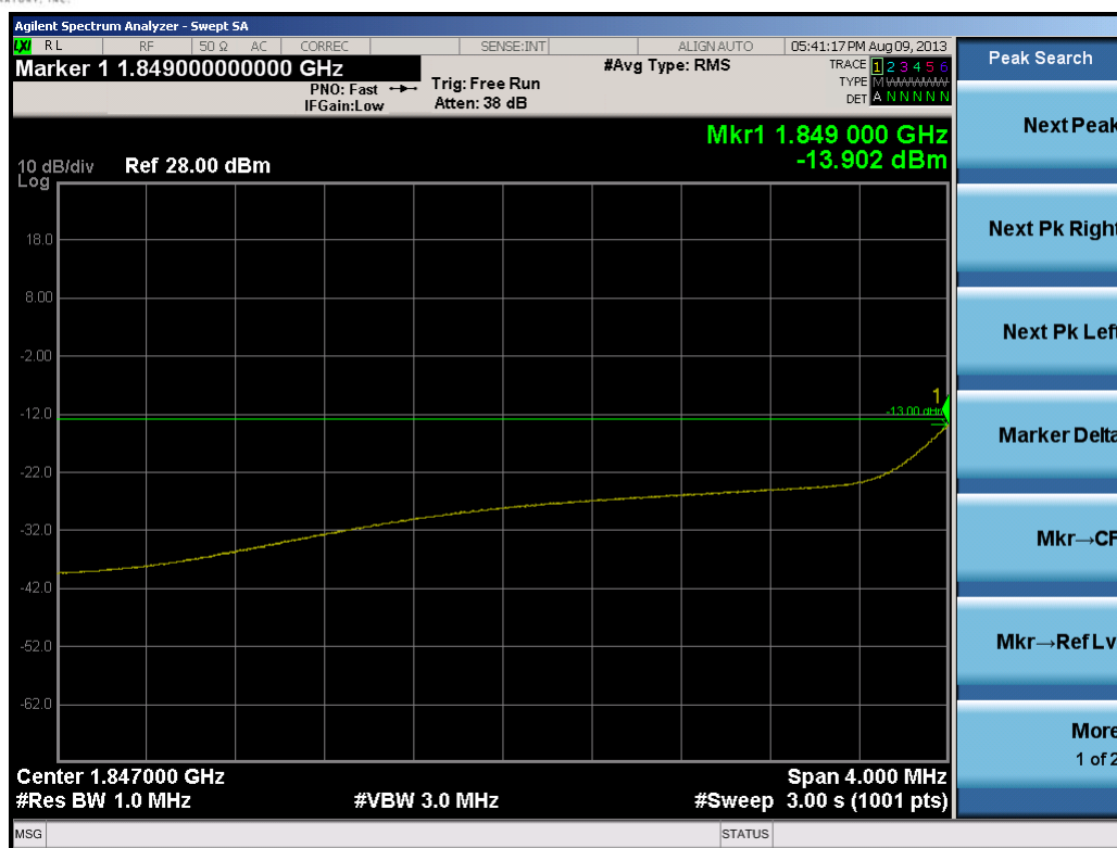
Plot 10-2. Lower Extended Band Edge Plot (5.0MHz QPSK – RB Size 25)
