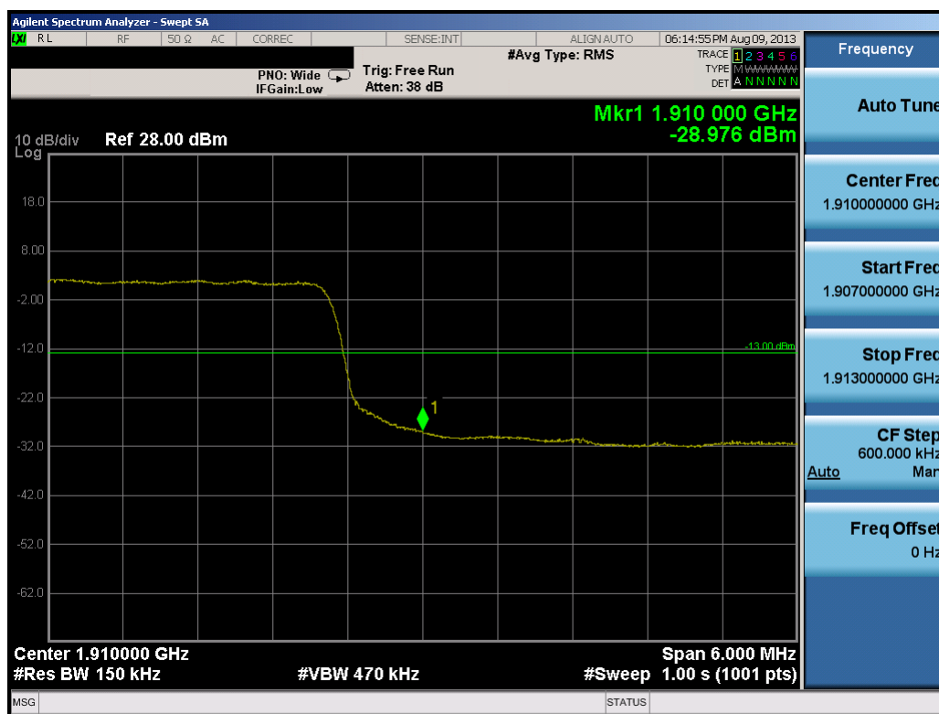
Plot 10-39. Upper Band Edge Plot (15.0MHz QPSK – RB Size 75)
