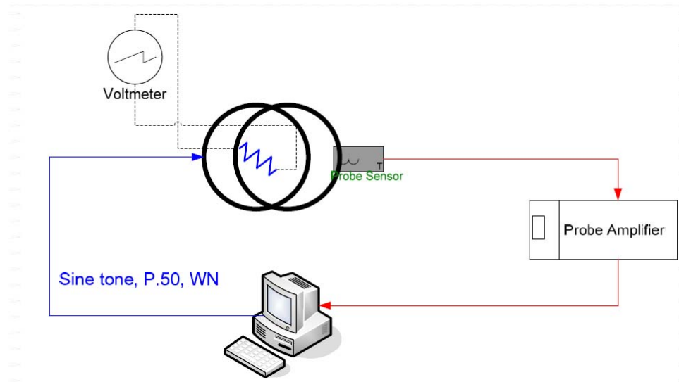
Figure 5-1 Validation Setup with Helmholtz Coil
