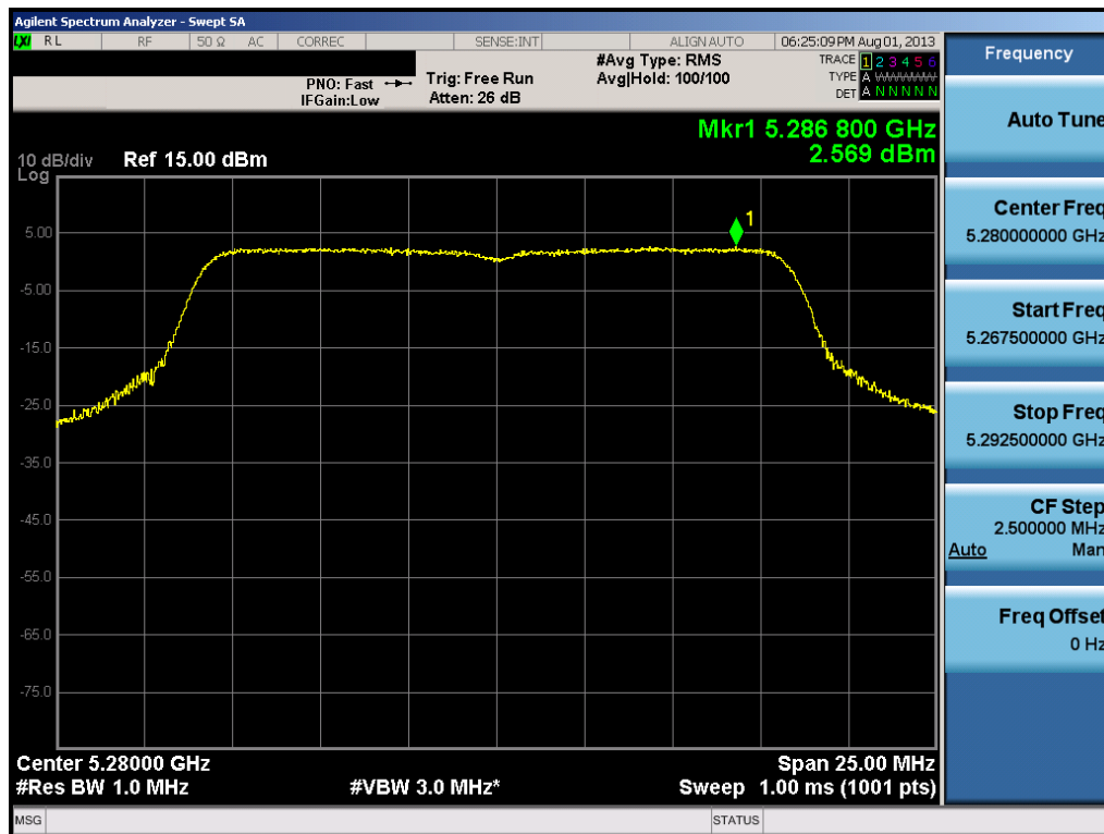
Plot 6-38. Peak Power Spectral Density Plot (802.11a (UNII Band 2) – Ch. 56)
