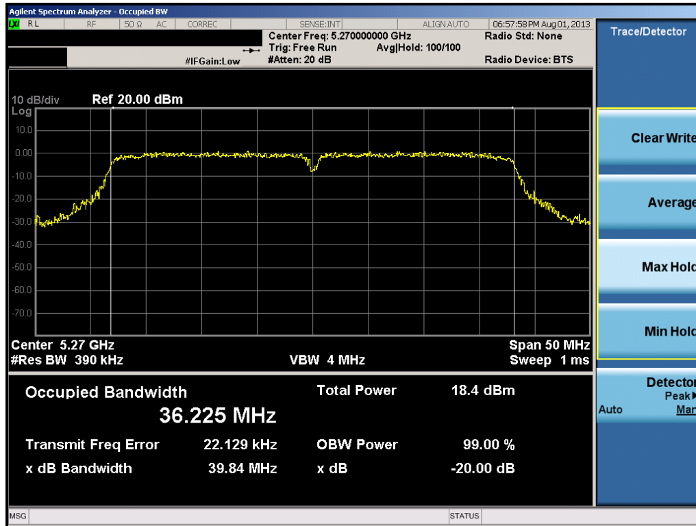
Plot 6-28. 20dB Bandwidth Plot (40MHz BW 802.11n (UNII Band 2) – Ch. 54)
