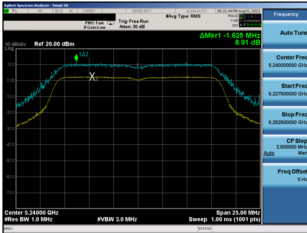
Plot 6-54. Peak Excursion Ratio Plot (802.11a)
