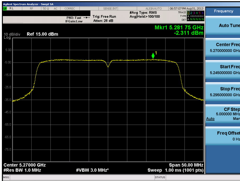
Plot 6-43. Peak Power Spectral Density Plot (40MHz BW 802.11n (UNII Band 2) – Ch. 54)
