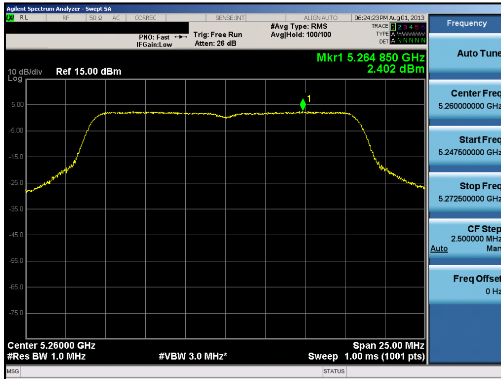
Plot 6-37. Peak Power Spectral Density Plot (802.11a (UNII Band 2) – Ch. 52)
