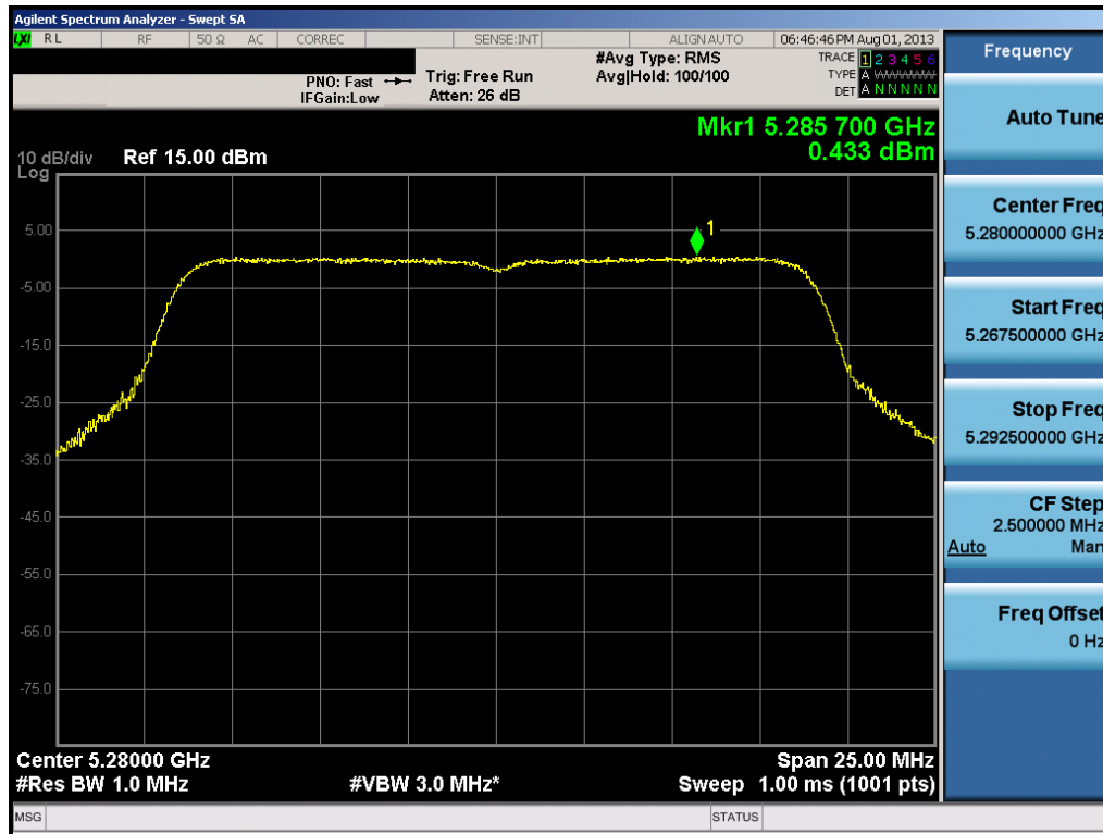
Plot 6-41. Peak Power Spectral Density Plot (20MHz BW 802.11n (UNII Band 2) – Ch. 56)
