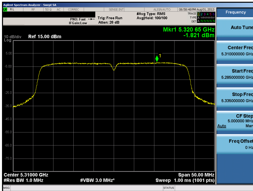
Plot 6-44. Peak Power Spectral Density Plot (40MHz BW 802.11n (UNII Band 2) – Ch. 62)
