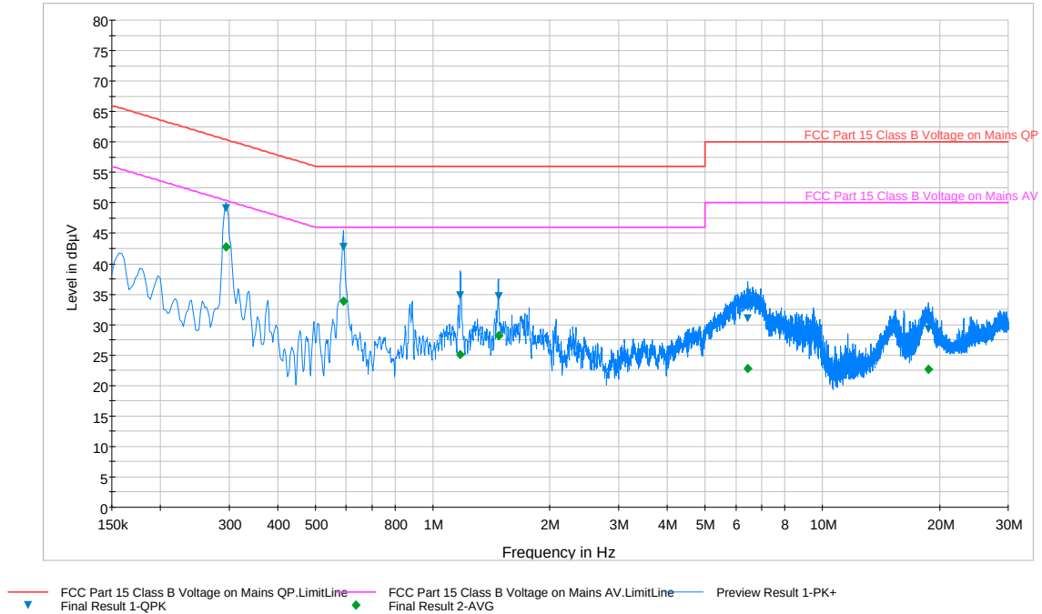
Plot 6-73. Line Conducted Plot with 802.11a UNII Band 2 (L1)
