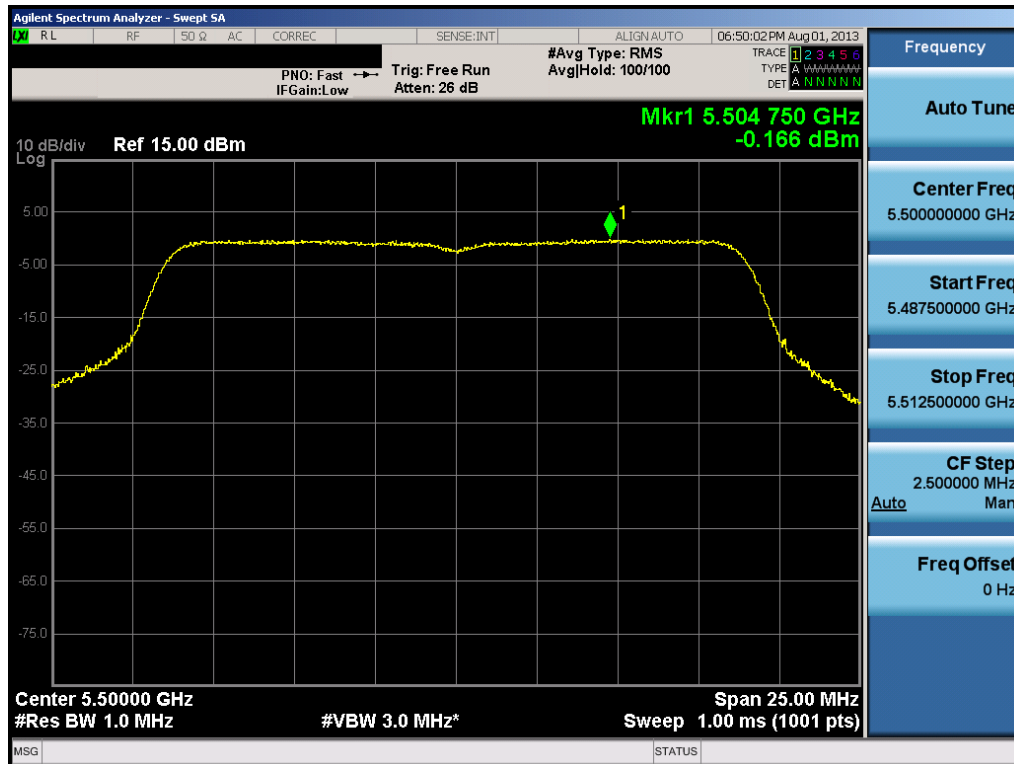
Plot 6-48. Peak Power Spectral Density Plot (20MHz BW 802.11n (UNII Band 3) – Ch. 100)
