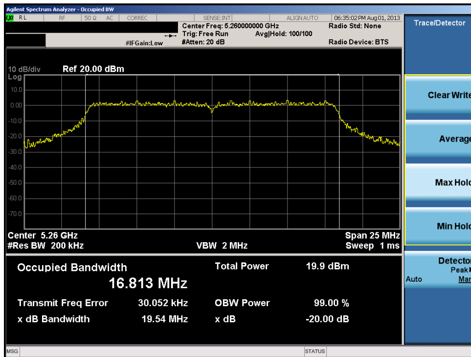
Plot 6-26. 20dB Bandwidth Plot (20MHz BW 802.11a (UNII Band 2) – Ch. 52)
