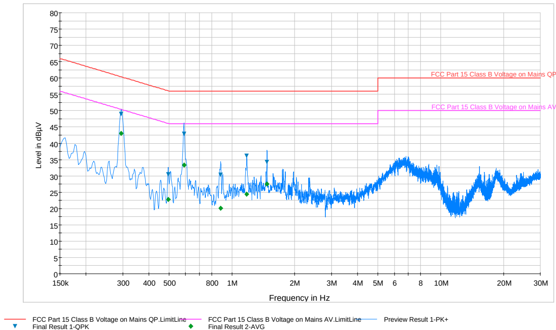
Plot 6-74. Line Conducted Plot with 802.11a UNII Band 2 (N)
