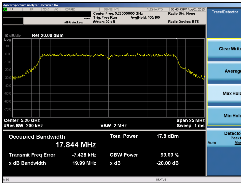
Plot 6-27. 20dB Bandwidth Plot (20MHz BW 802.11n (UNII Band 2) – Ch. 52)
