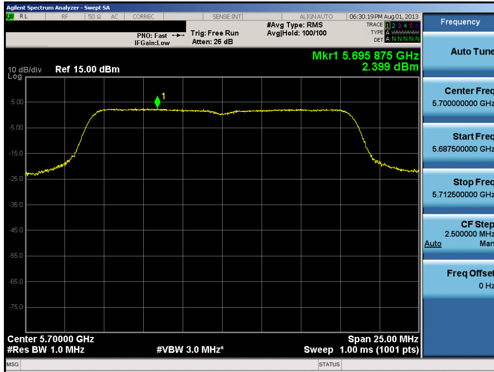
Plot 6-47. Peak Power Spectral Density Plot (802.11a (UNII Band 3) – Ch. 140)
