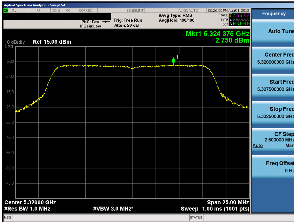
Plot 6-39. Peak Power Spectral Density Plot (802.11a (UNII Band 2) – Ch. 64)
