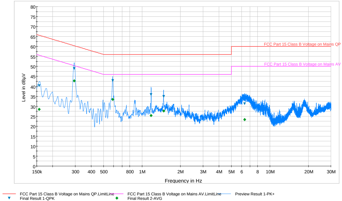
Plot 6-75. Line Conducted Plot with 802.11a UNII Band 3 (L1)
