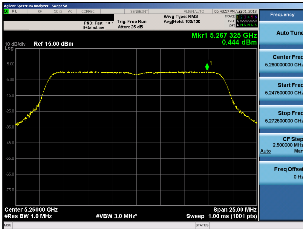
Plot 6-40. Peak Power Spectral Density Plot (20MHz BW 802.11n (UNII Band 2) – Ch. 52)
