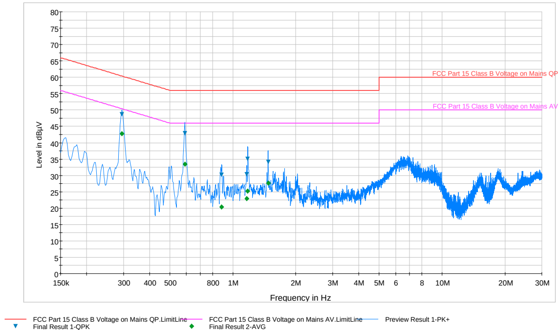
Plot 6-76. Line Conducted Plot with 802.11a UNII Band 3 (N)
