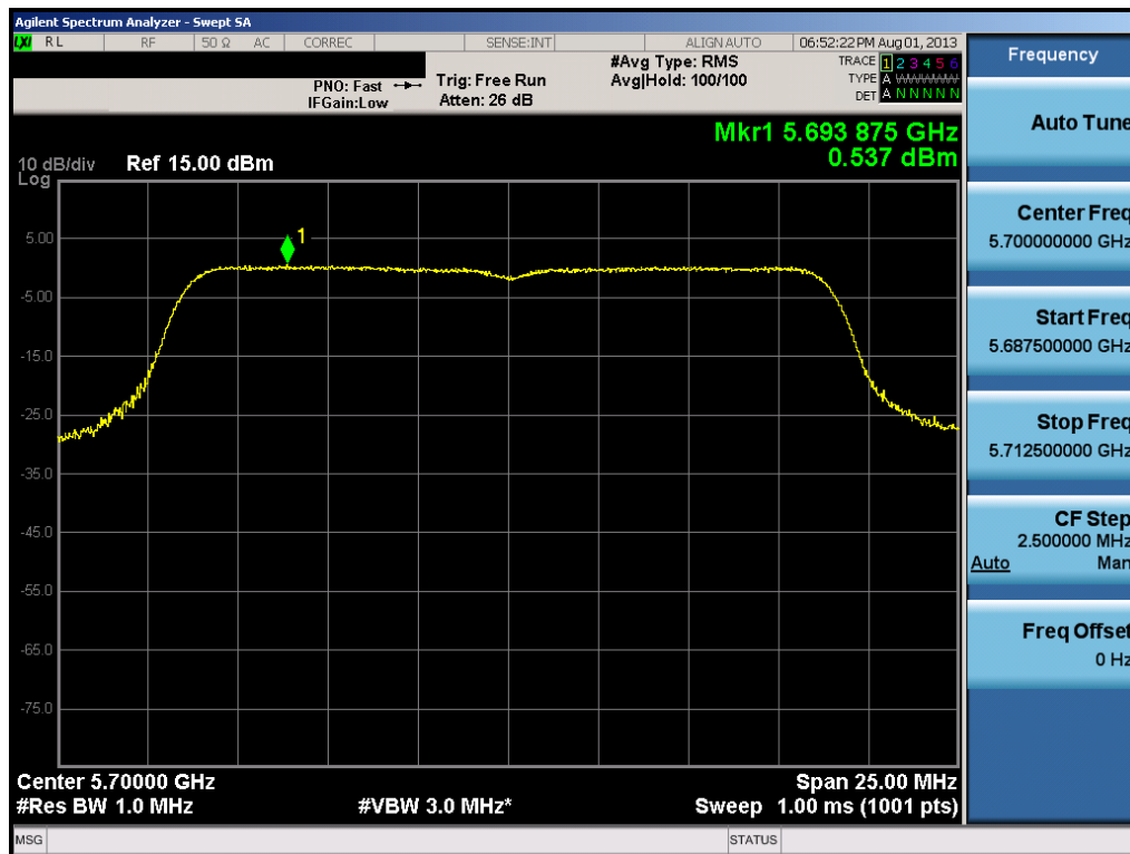
Plot 6-50. Peak Power Spectral Density Plot (20MHz BW 802.11n (UNII Band 3) – Ch. 140)
