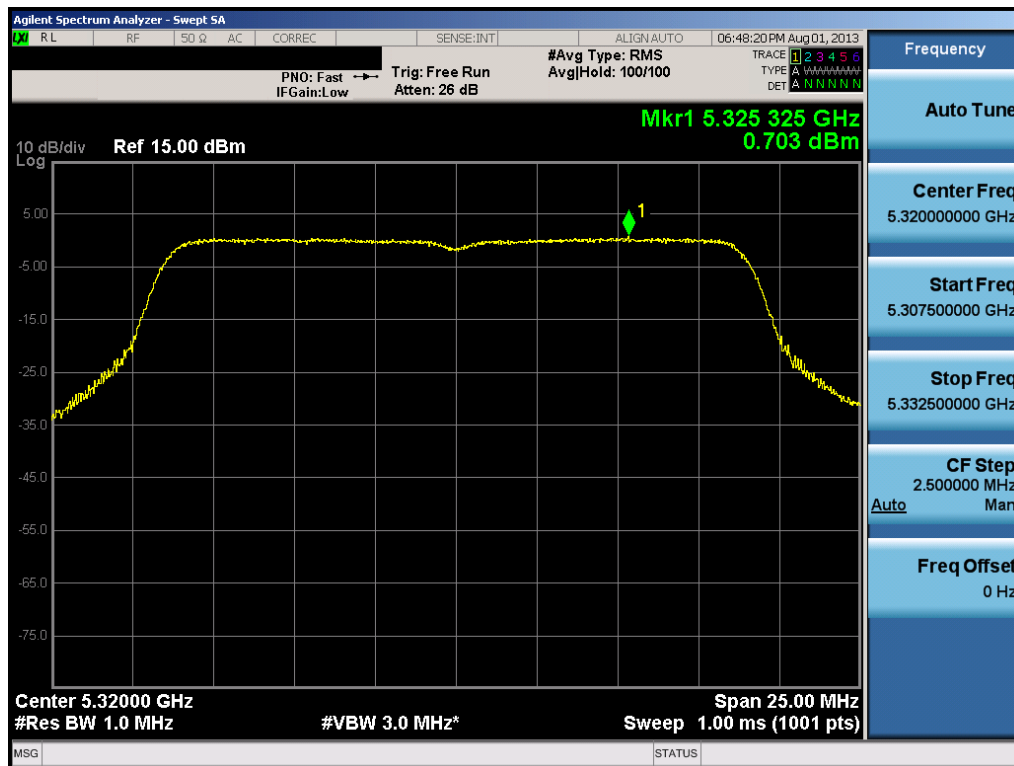
Plot 6-42. Peak Power Spectral Density Plot (20MHz BW 802.11n (UNII Band 2) – Ch. 64)
