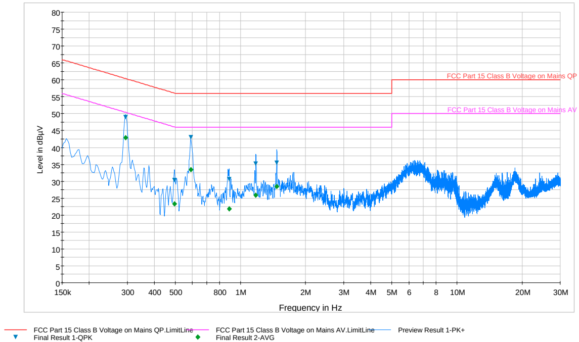
Plot 6-71. Line Conducted Plot with 802.11a UNII Band 1 (L1)
