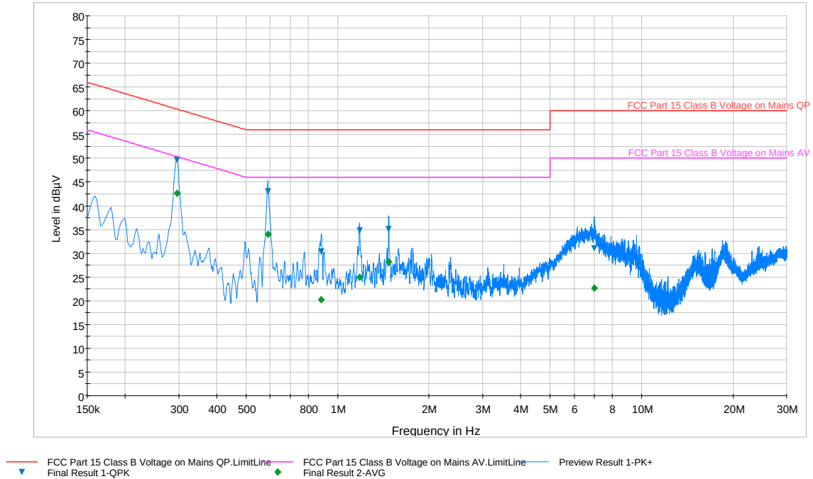
Plot 6-72. Line Conducted Plot with 802.11a UNII Band 1 (N)
