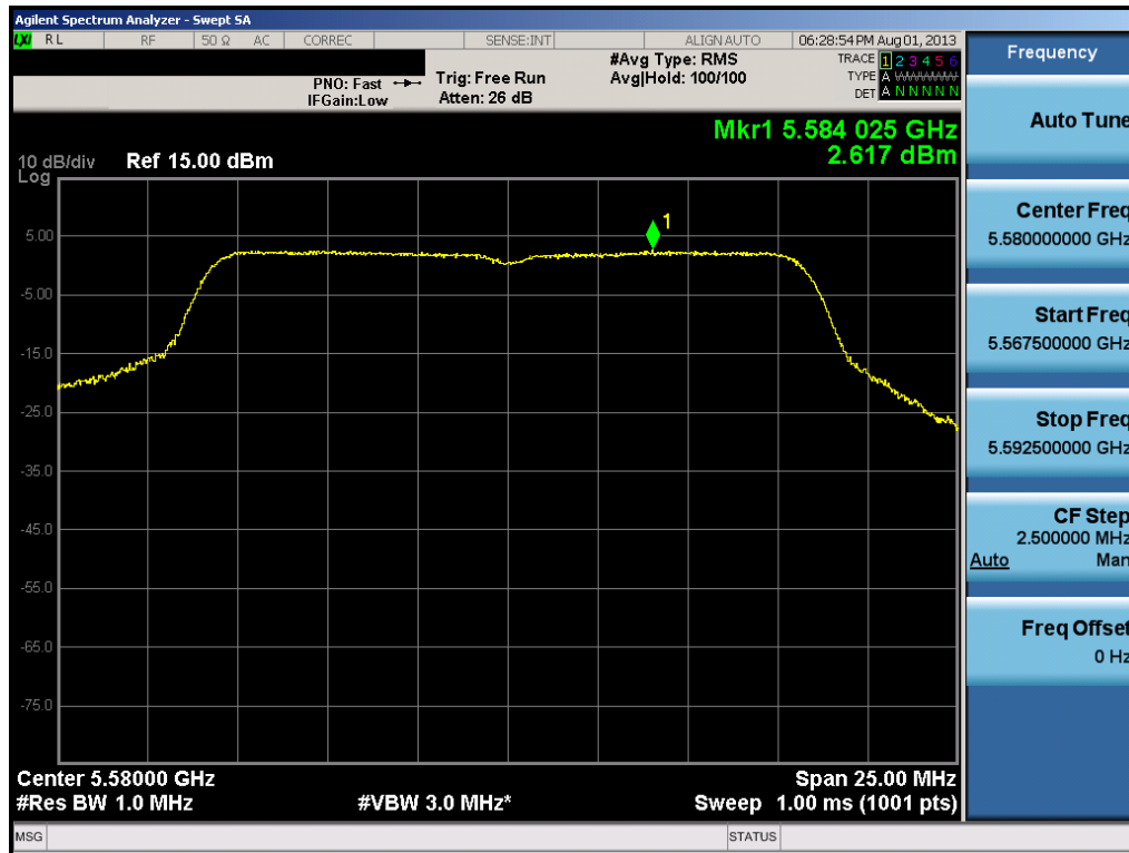
Plot 6-46. Peak Power Spectral Density Plot (802.11a (UNII Band 3) – Ch. 116)
