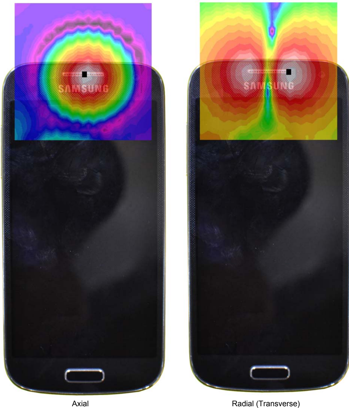
Figure 13-3 T-Coil Scan Overlay Magnetic Field Distributions
