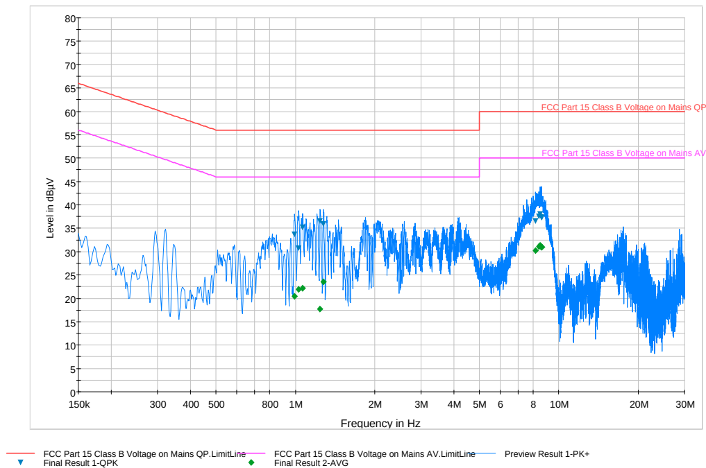
Plot 6-34. Line-Conducted Test Plot (N)
