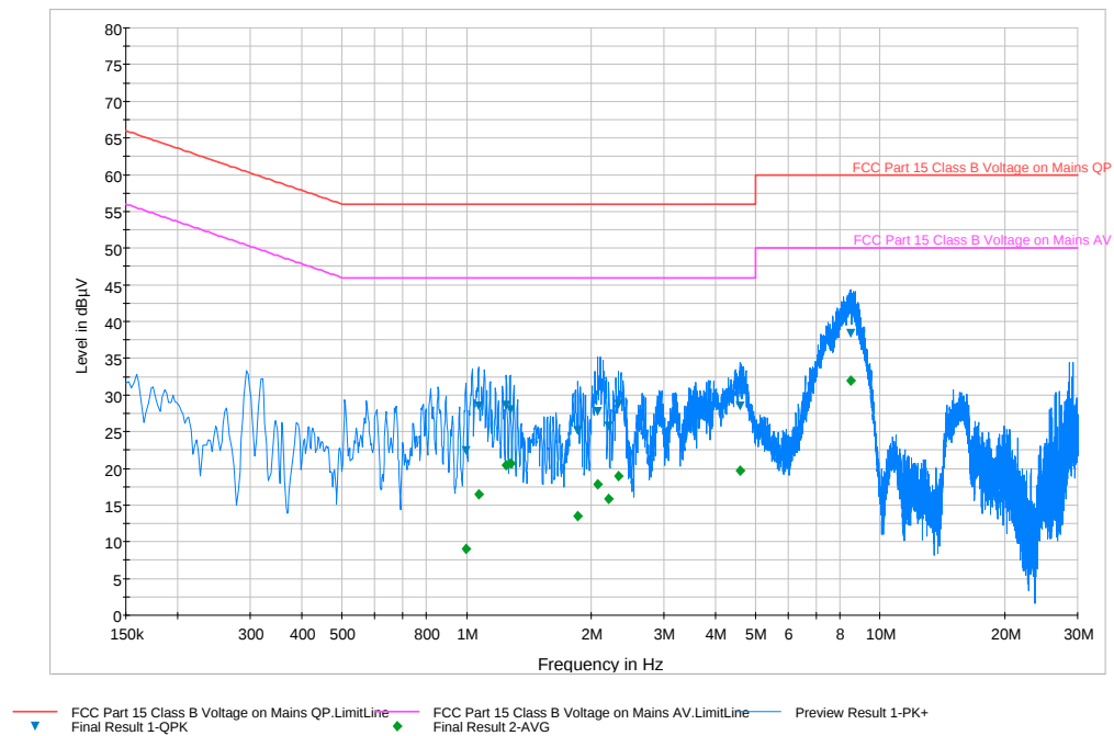
Plot 6-33. Line-Conducted Test Plot (L1)
