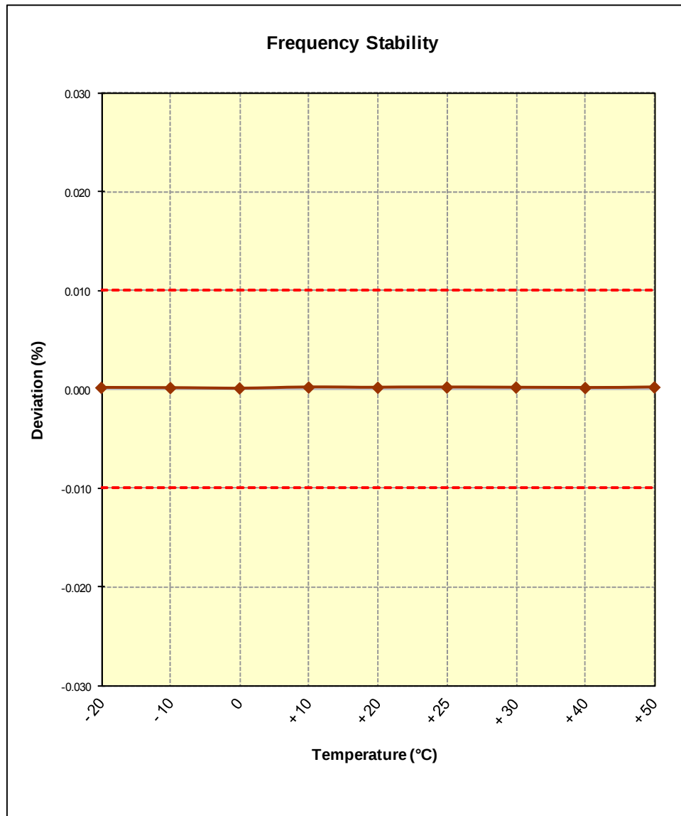
Figure 8-4. Frequency Stability Plot
