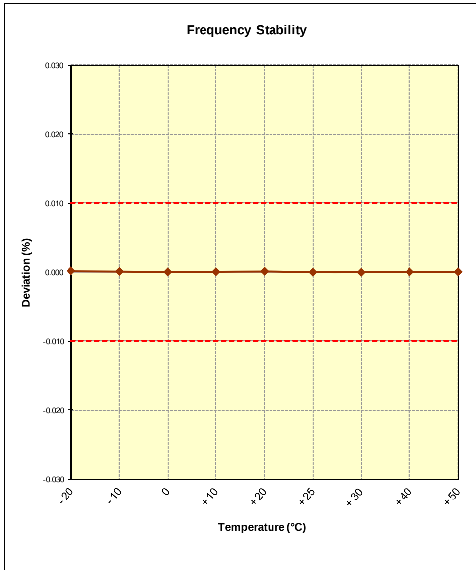
Figure 8-5. Frequency Stability Plot
