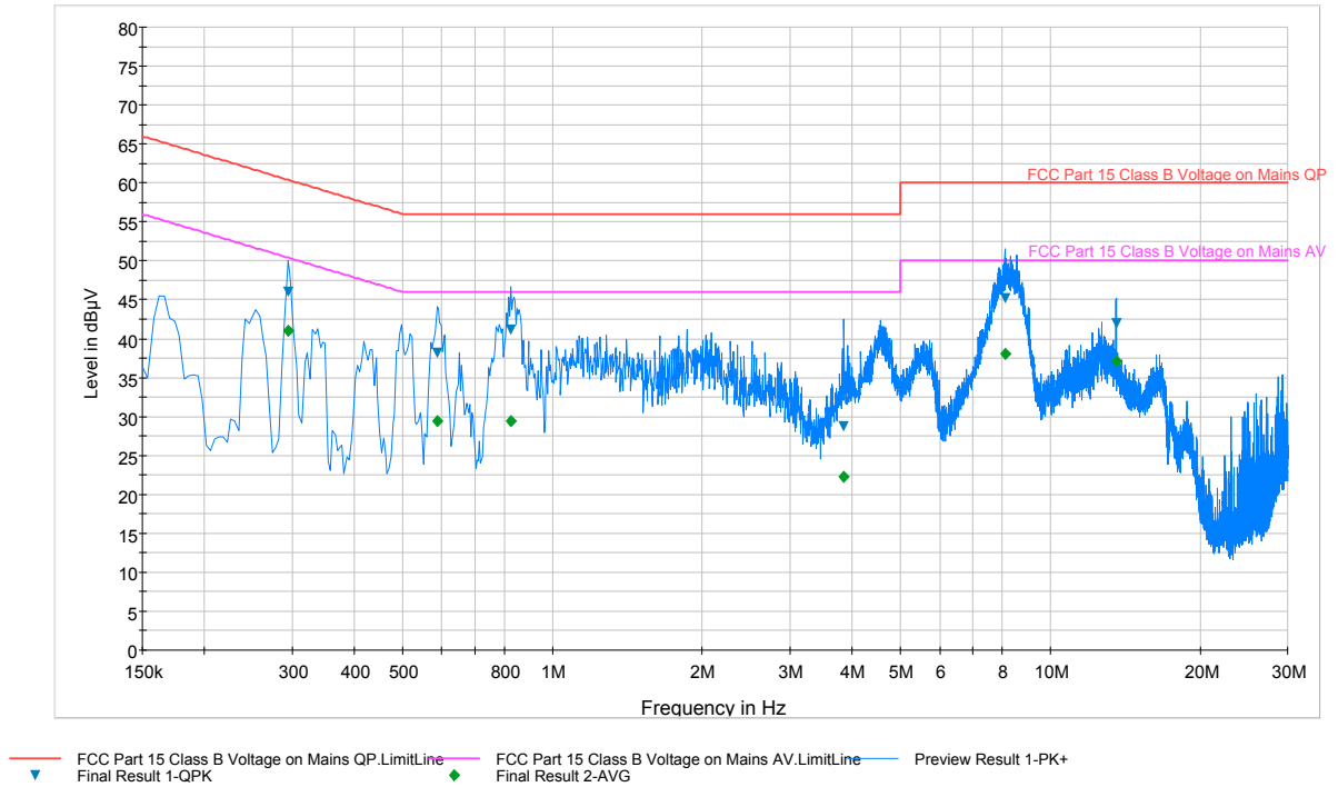
Plot 8-1. Line-Conducted Test Plot (L1)
