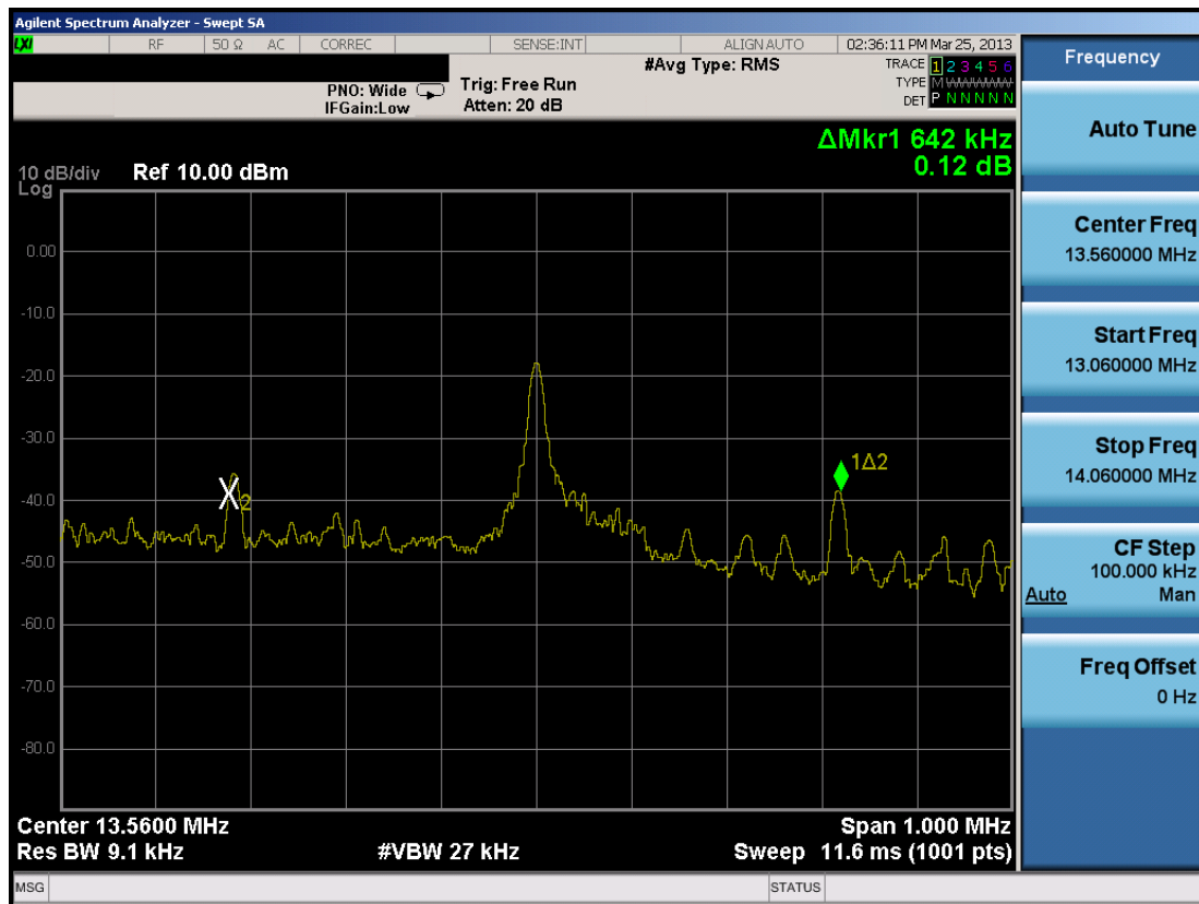
Figure 8-3. 20dB Bandwidth Plot (Wireless Charging Cover)
