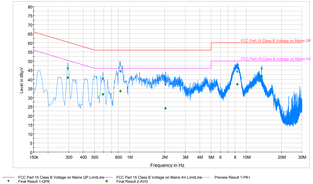
Plot 8-2. Line-Conducted Test Plot (N)
