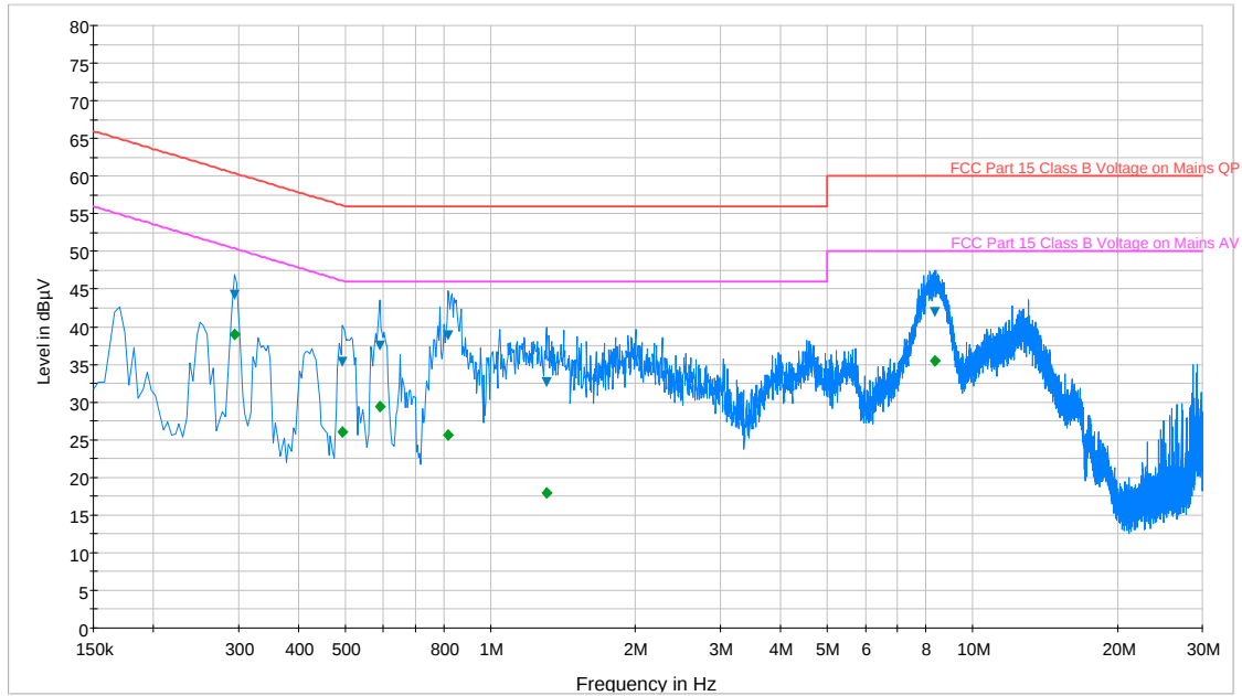
Plot 6-103. Line Conducted Plot with 802.11a UNII Band 2 (L1)
