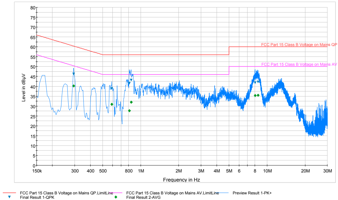
Plot 6-74. Line Conducted Plot with 802.11a (N)
