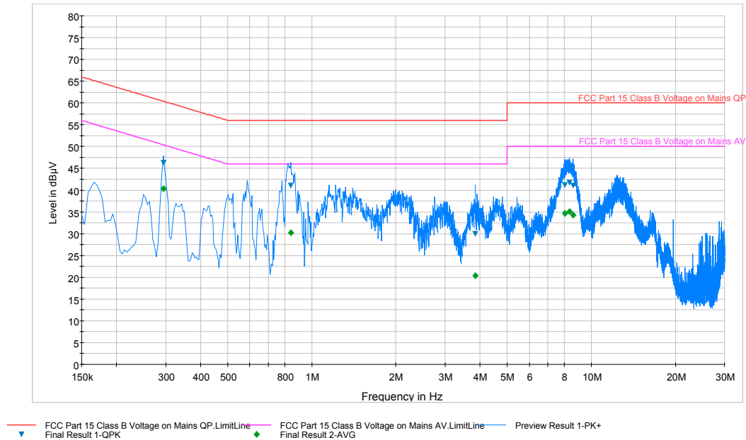
Plot 6-72. Line Conducted Plot with 802.11b (N)
