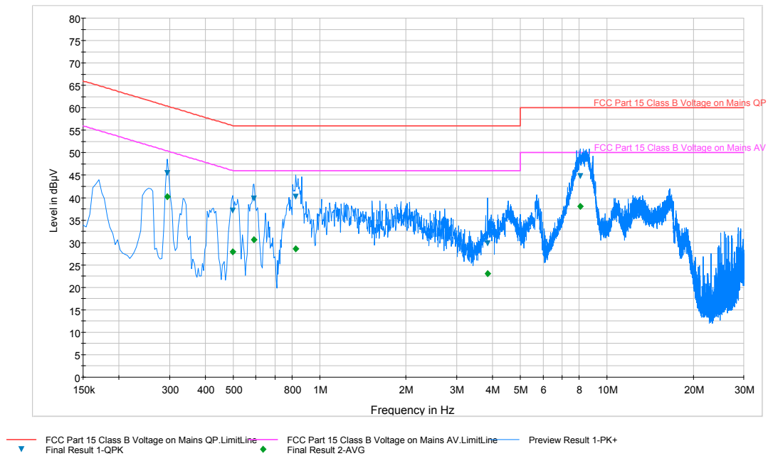
Plot 6-73. Line Conducted Plot with 802.11a (L1)
