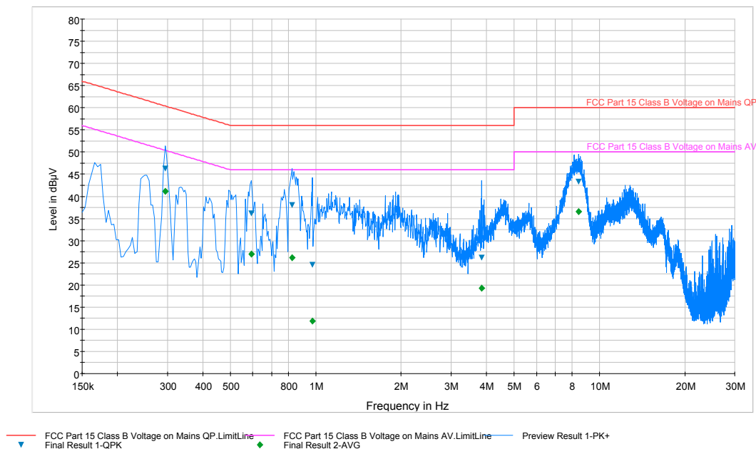
Plot 6-71. Line Conducted Plot with 802.11b (L1)
