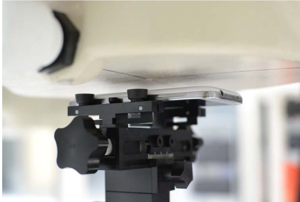
SAR Test Setup Photo 6 – Back side at 1.0 cm with Wireless Charging Cover
