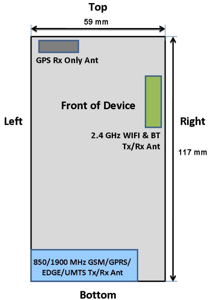
Figure 1-1 DUT Antenna Locations
