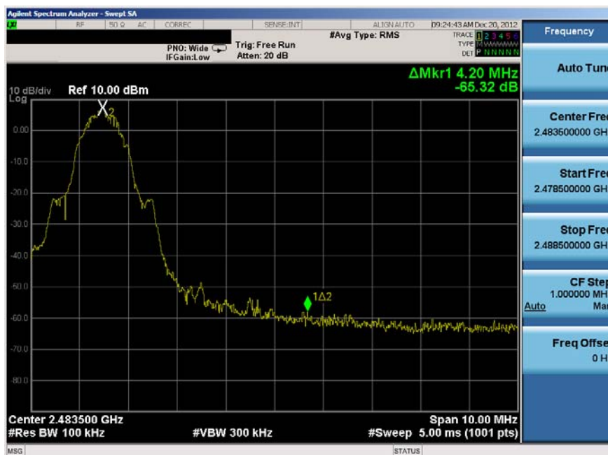
Plot 6-8. Band Edge Plot (Bluetooth (LE) – Ch. 39)
