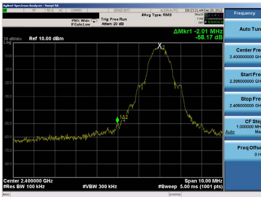
Plot 6-7. Band Edge Plot (Bluetooth (LE) – Ch. 0)
