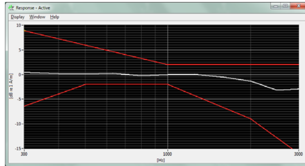
Figure 7-1 Axial Frequency Response
