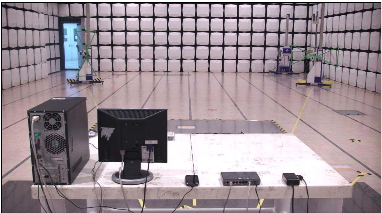
[ Radiated Disturbance for Below 1 GHz – Rear ]
