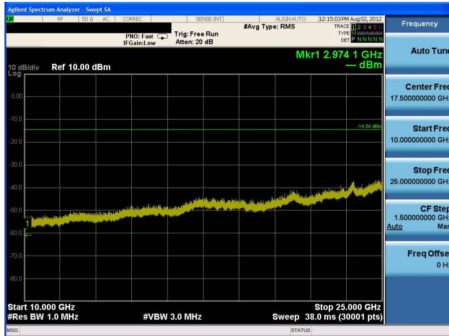
Plot 6-19. Conducted Spurious Plot (Bluetooth, 3Mbps – Ch. 0)
