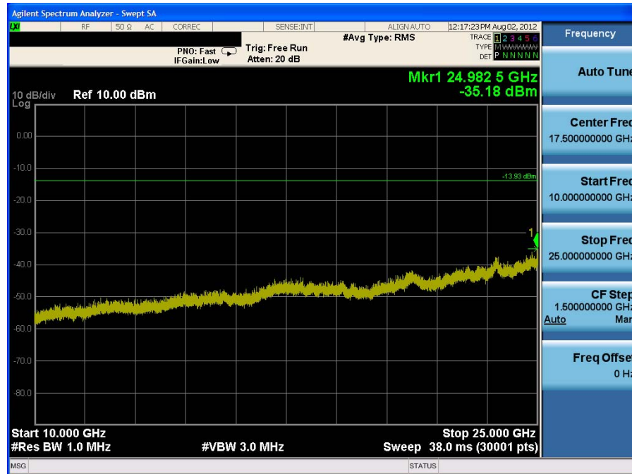
Plot 6-21. Conducted Spurious Plot (Bluetooth, 3Mbps – Ch. 39)
