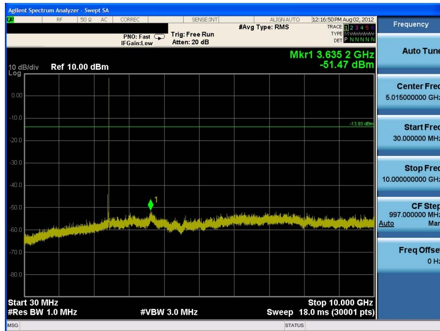
Plot 6-20. Conducted Spurious Plot (Bluetooth, 3Mbps – Ch. 39)
