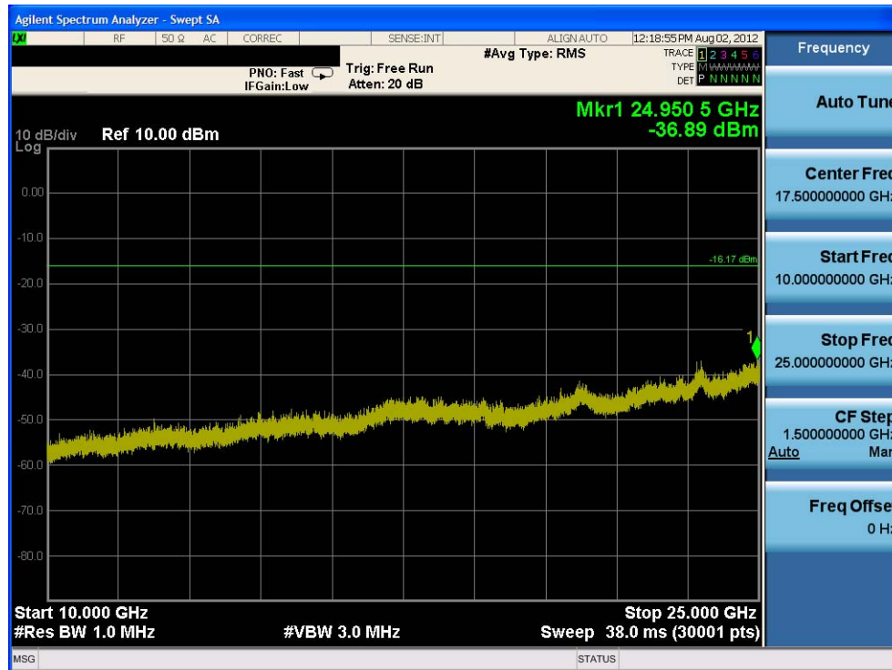
Plot 6-23. Conducted Spurious Plot (Bluetooth, 3Mbps – Ch. 78)
