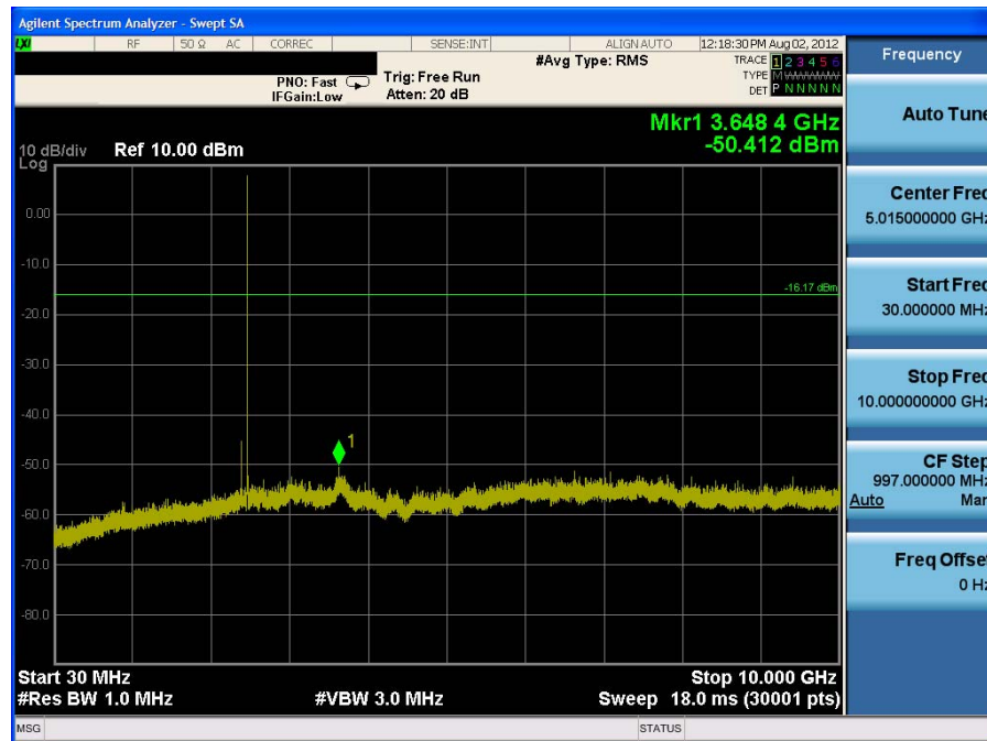
Plot 6-22. Conducted Spurious Plot (Bluetooth, 3Mbps – Ch. 78)
