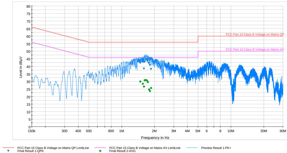
Plot 6-25. Line-Conducted Test Plot (N)
