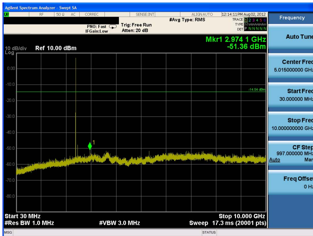
Plot 6-18. Conducted Spurious Plot (Bluetooth, 3Mbps – Ch. 0)
