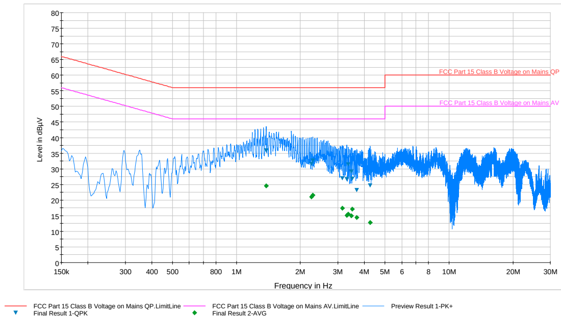
Plot 6-24. Line-Conducted Test Plot (L1)
