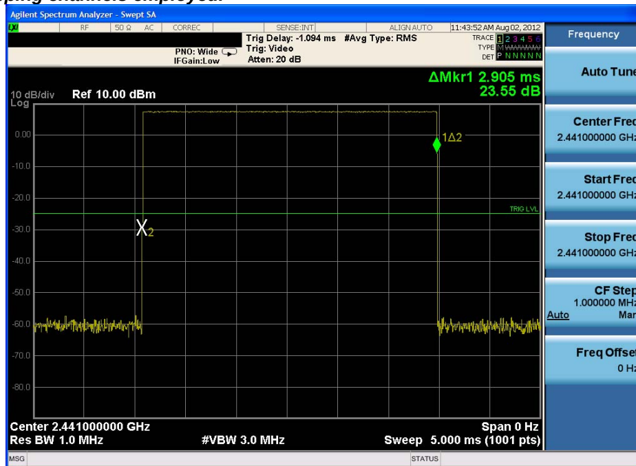
Plot 6-15. Time of Occupancy Plot (Bluetooth)
