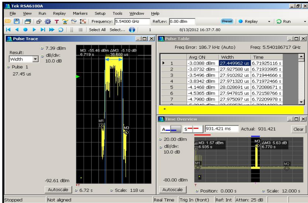
Figure 6-7. Pulse width analysis using Pulse Table and Pulse Trace Function
