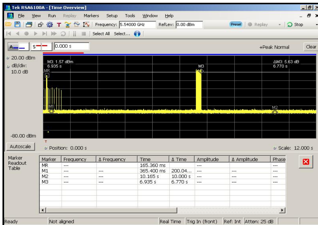
Figure 6-5. Channel Move Time (< 10sec)
