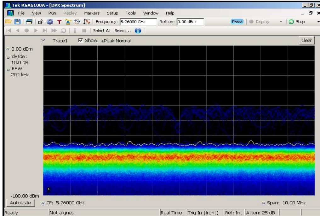
Figure 5-3. Real-Time Spectrum Display, No WLAN Traffic
