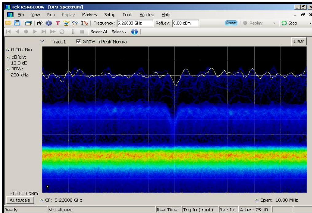
Figure 5-4. Real-Time Spectrum Display, WLAN Traffic (Streaming Video)
