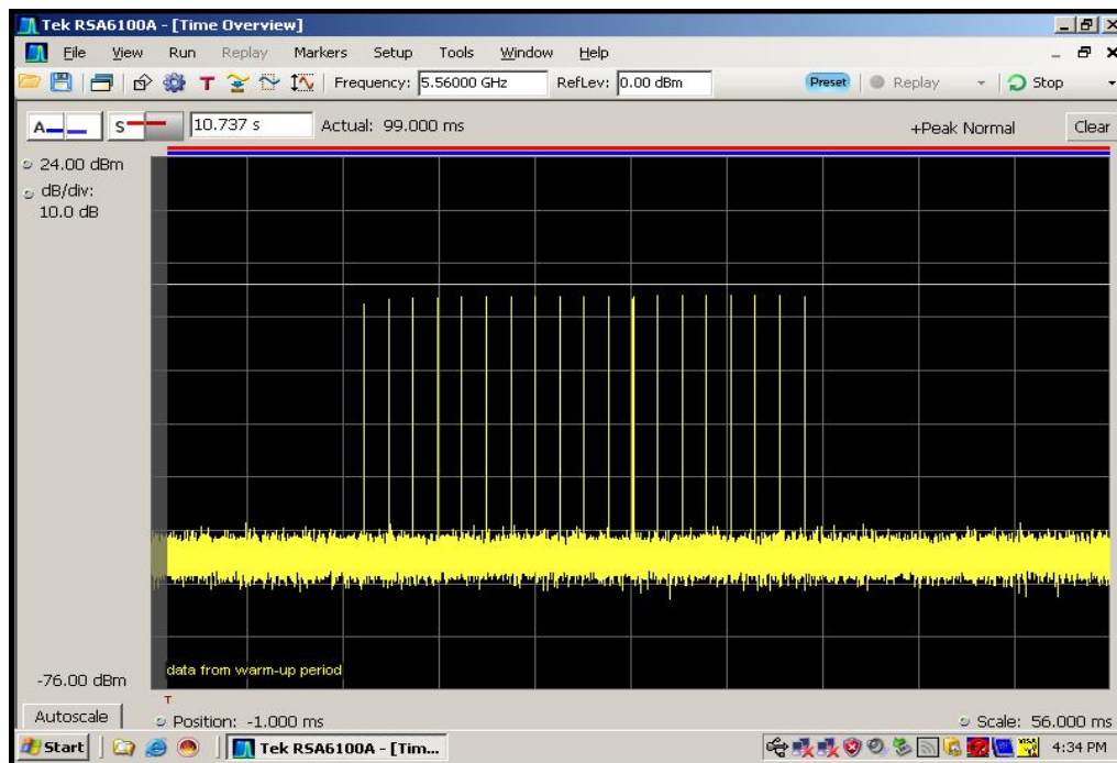
Figure 6-1. Type 1 Radar Pulse
