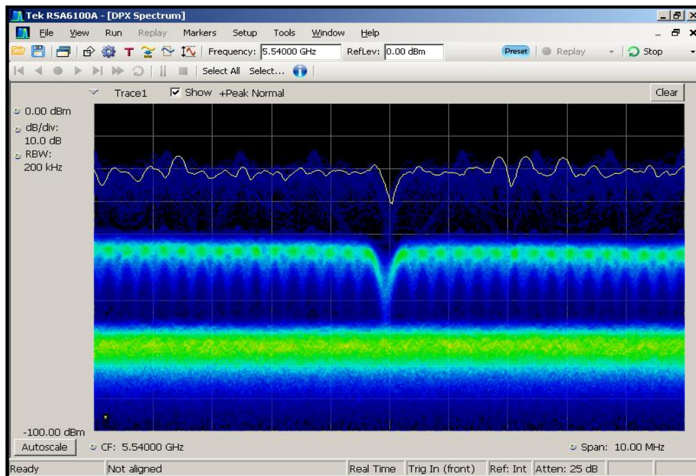
Figure 6-4. Real-Time Spectrum Display, WLAN Traffic (Streaming Video)
