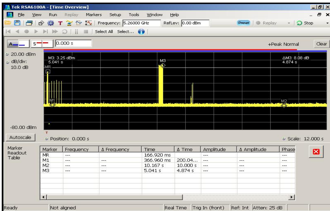
Figure 5-5. Channel Move Time (< 10sec)
