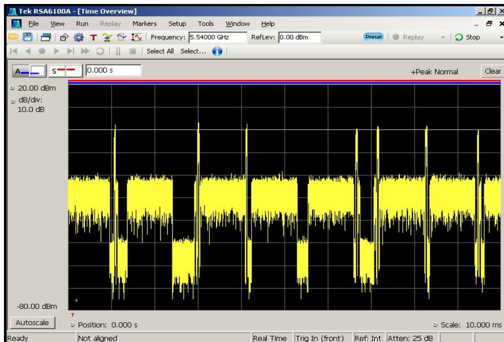
Figure 6-2. Time Display WLAN Channel Traffic (Streaming Video)
