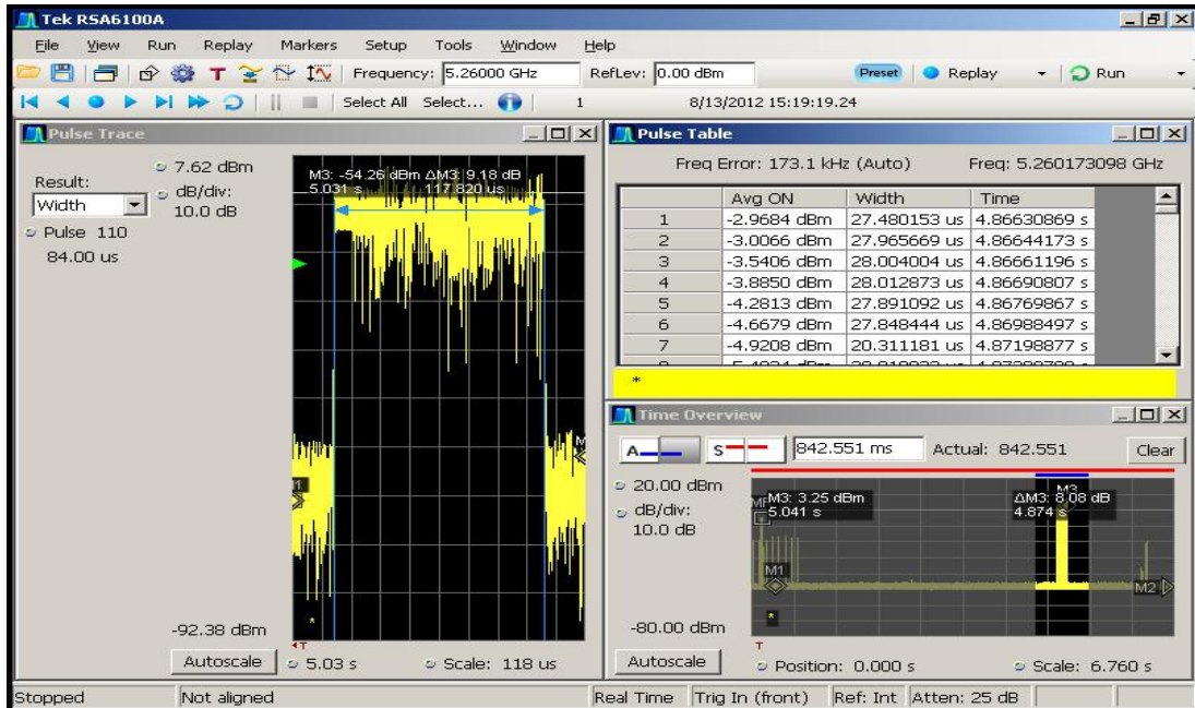
Figure 5-7. Pulse width analysis using Pulse Table and Pulse Trace Function
