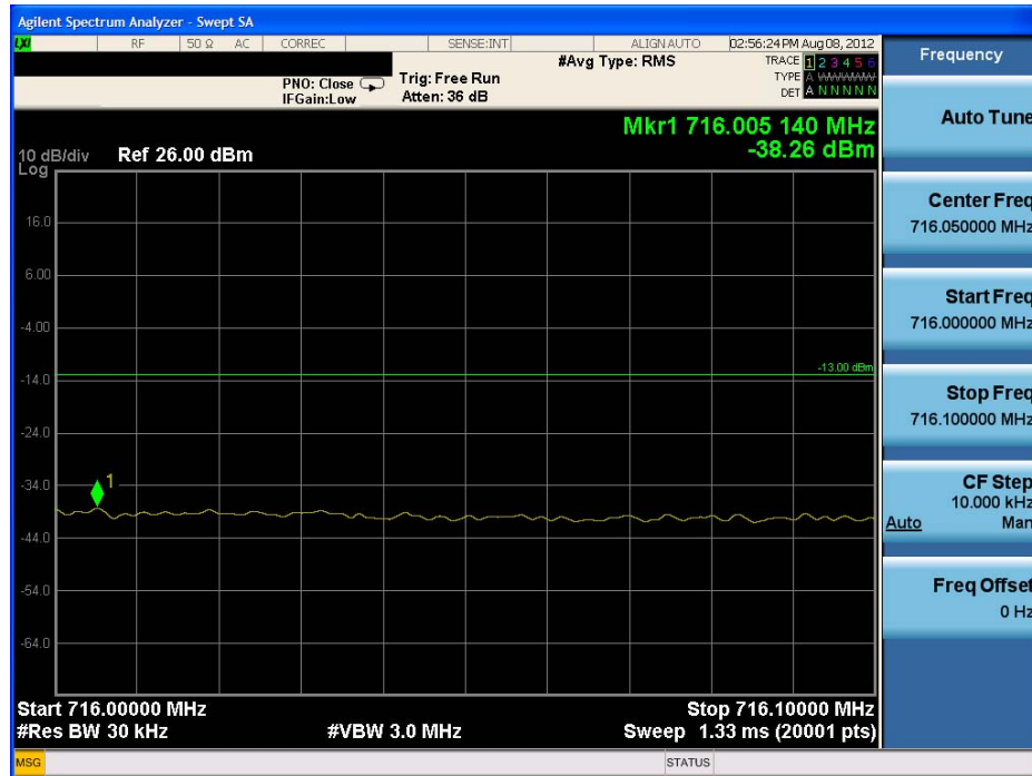
Plot 7-23. Upper Band Edge Plot (QPSK – RB Size 1, Offset 0)
