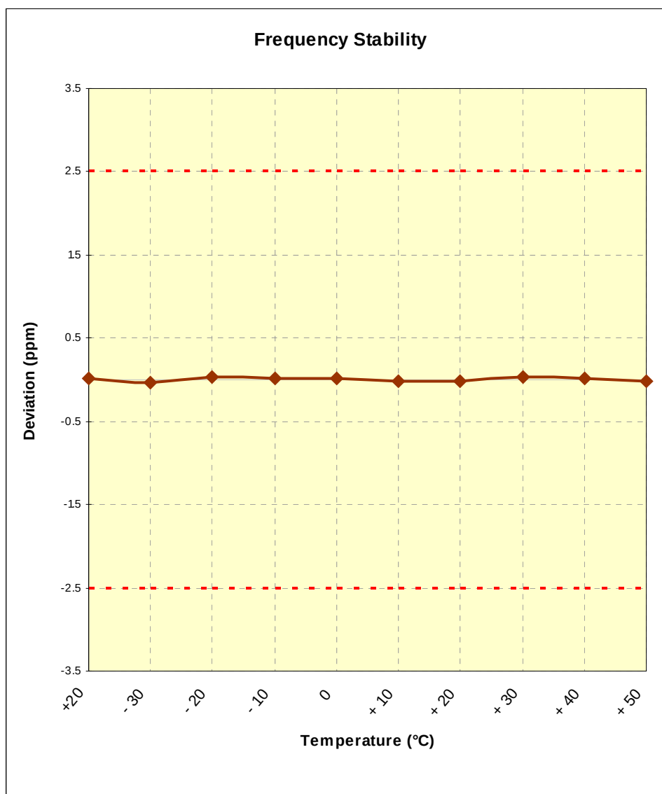
Figure 6-2. Frequency Stability Graph (Band 5)
