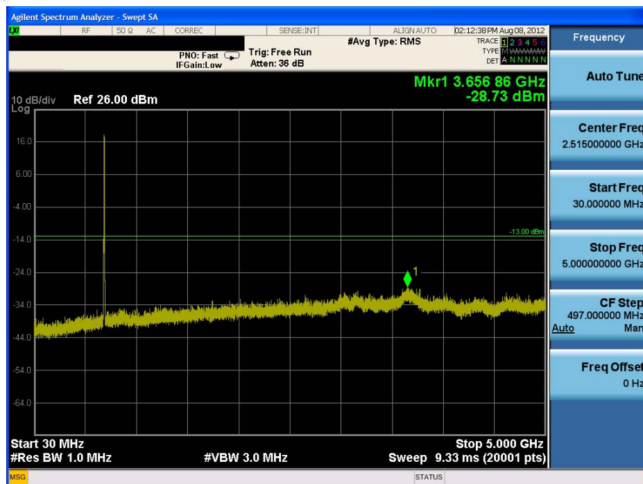
Plot 7-7. Conducted Spurious Plot (16QAM – RB Size 1, RB Offset 0 – Mid Channel)
