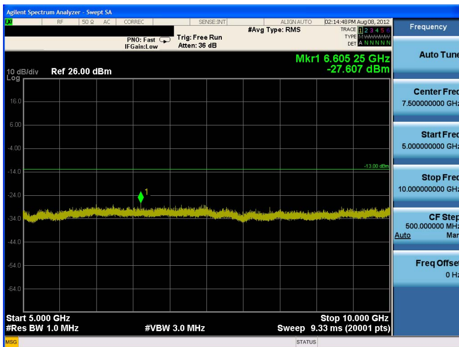
Plot 7-8. Conducted Spurious Plot (16 QAM– RB Size 1, RB Offset 0 – Mid Channel)
