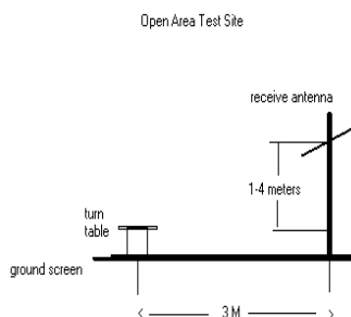
Figure 3-2. Diagram of 3-meter outdoor test range
