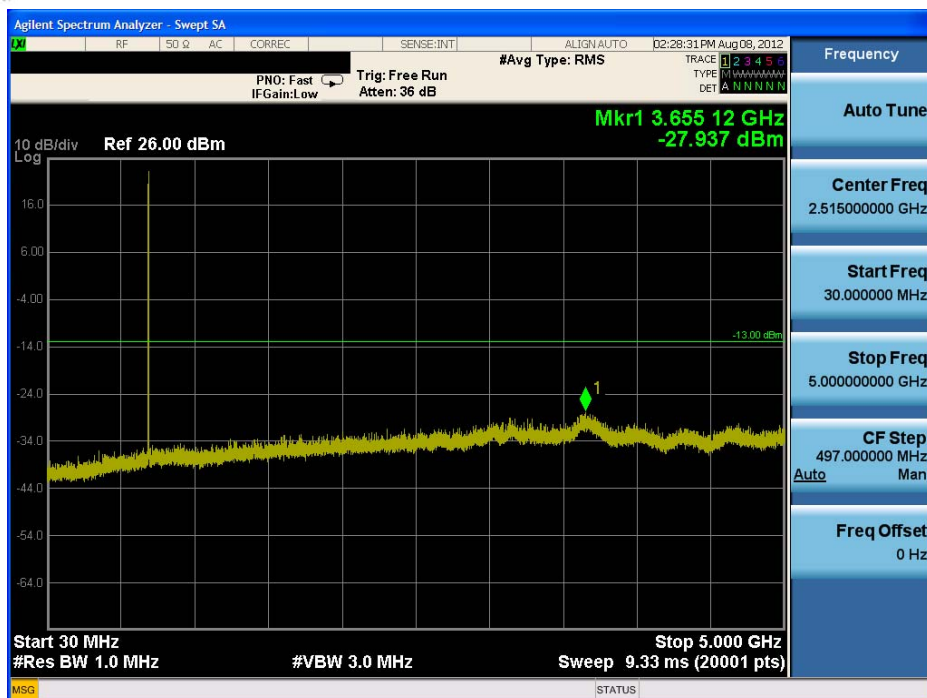
Plot 7-9. Conducted Spurious Plot (16QAM – RB Size 1, RB Offset 0 – High Channel)
