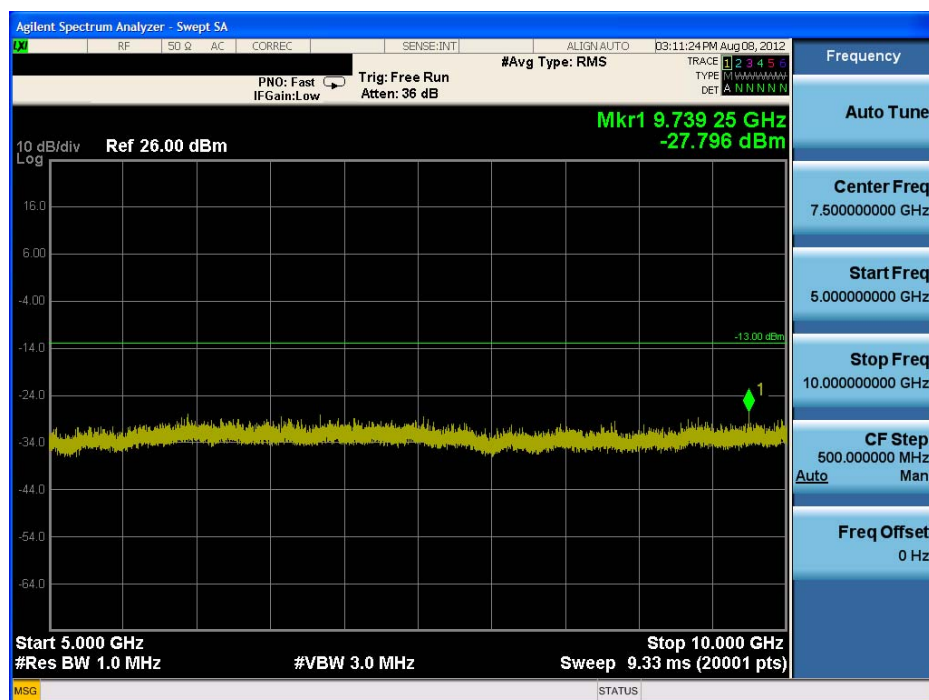
Plot 7-18. Conducted Spurious Plot (QPSK – RB Size 50, Offset 0 – Low Channel)
