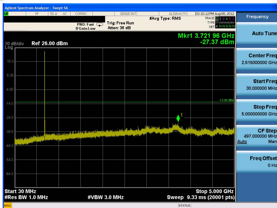
Plot 7-17. Conducted Spurious Plot (QPSK – RB Size 50, Offset 0 – Low Channel)
