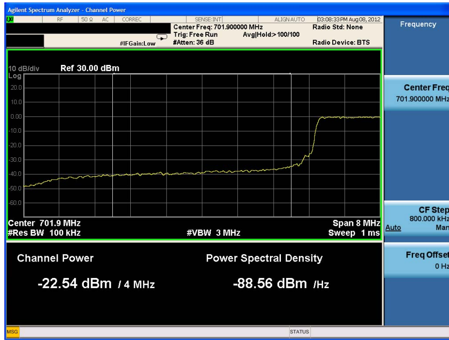
Plot 7-13. Lower Band Edge Plot (QPSK – RB Size 25, Offset 0)
