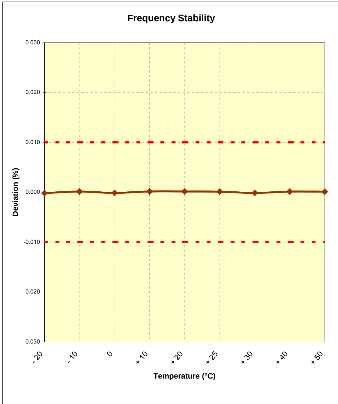
Figure 8-3. Frequency Stability Plot
