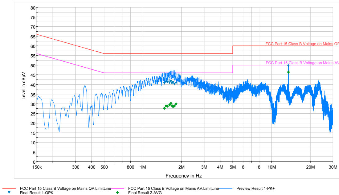
Plot 8-2. Line-Conducted Test Plot (N)
