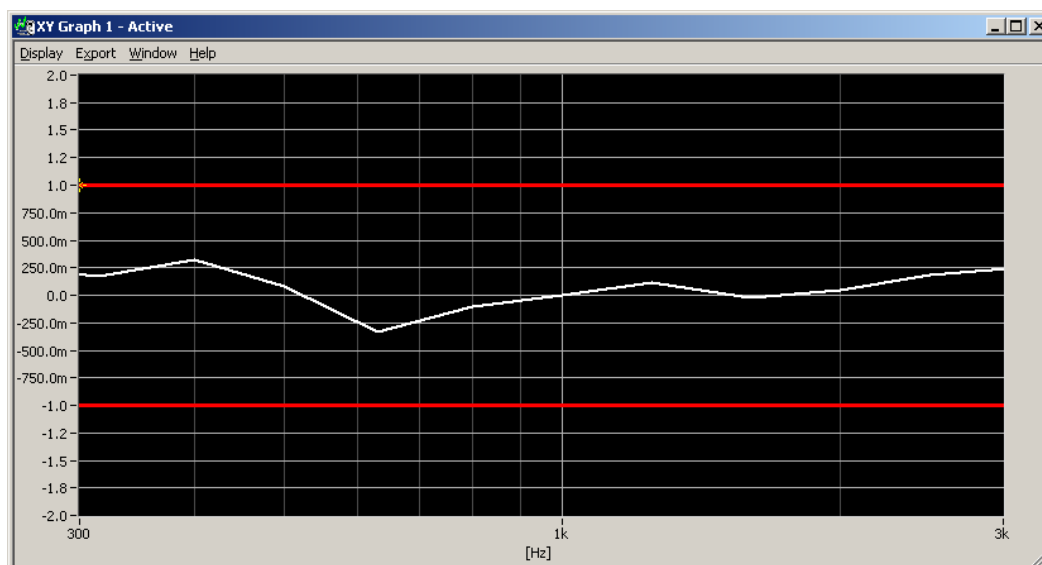
Figure 7-3 Helmholtz Coil Validation for Frequency Response
