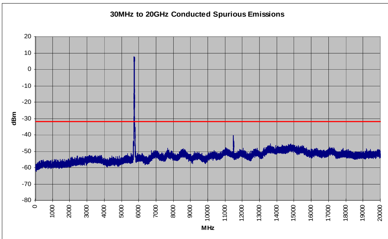
Plot 6-53. Conducted Spurious Plot (802.11a – Ch. 149)
