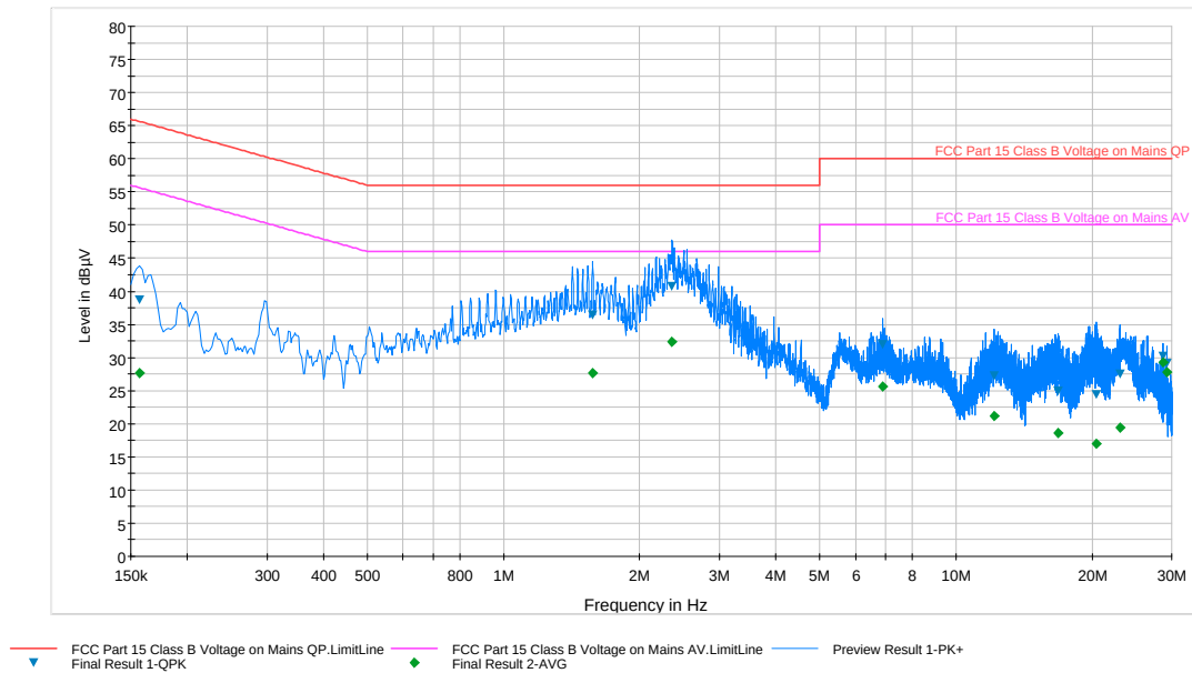
Plot 6-59. Line Conducted Plot with 802.11b (L1)
