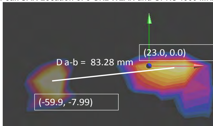
Figure 11-7 Peak SAR Location of 5 GHz WLAN and GPRS 1900 MHz
