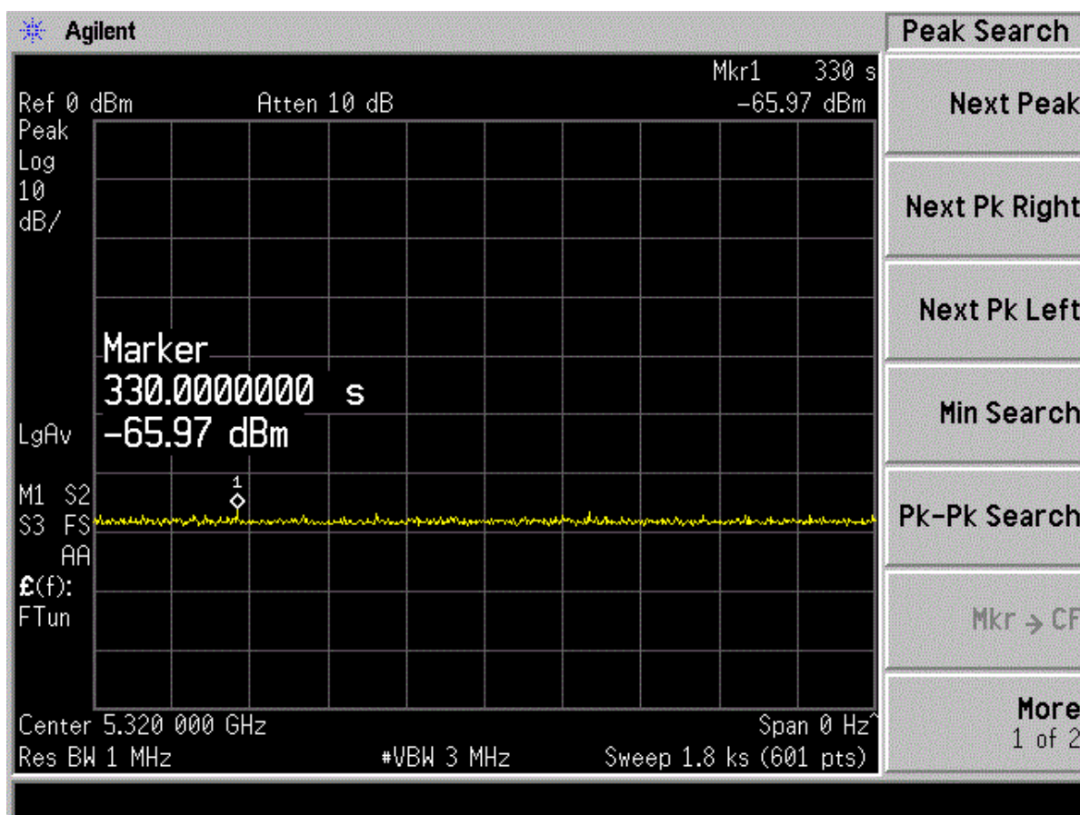
Figure 5-6. Aggregate Time using Pulse Table Capability
