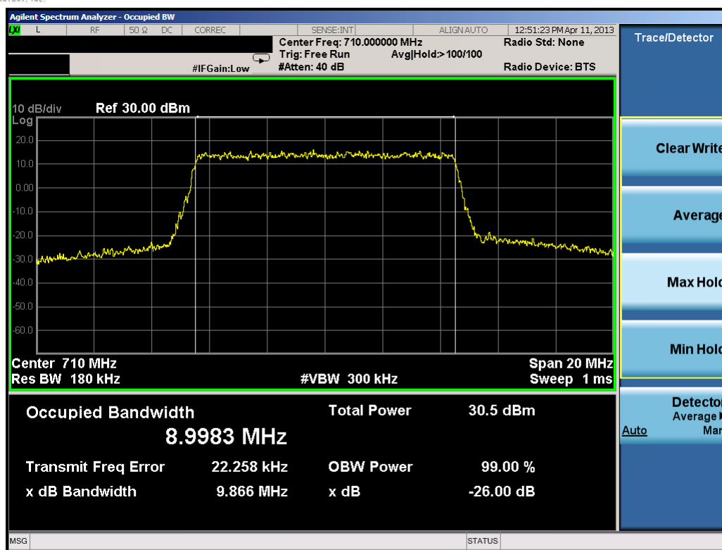
Plot 7-12. Occupied Bandwidth Plot (10.0MHz QPSK – RB Size 50)
