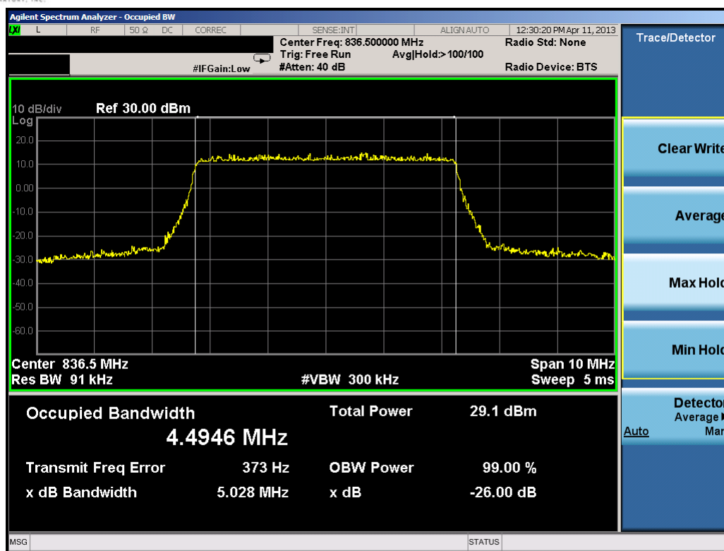
Plot 8-2. Occupied Bandwidth Plot (5.0MHz QPSK – RB Size 25)
