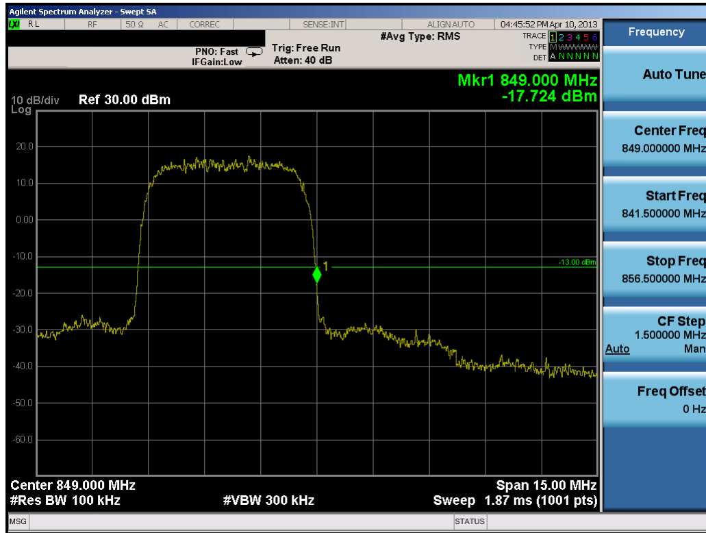
Plot 7-34. Band Edge Plot (Cellular WCDMA Mode – Ch. 4233)
