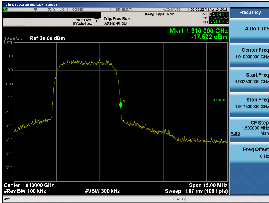
Plot 7-45. Band Edge Plot (PCS WCDMA Mode – Ch. 9538)
