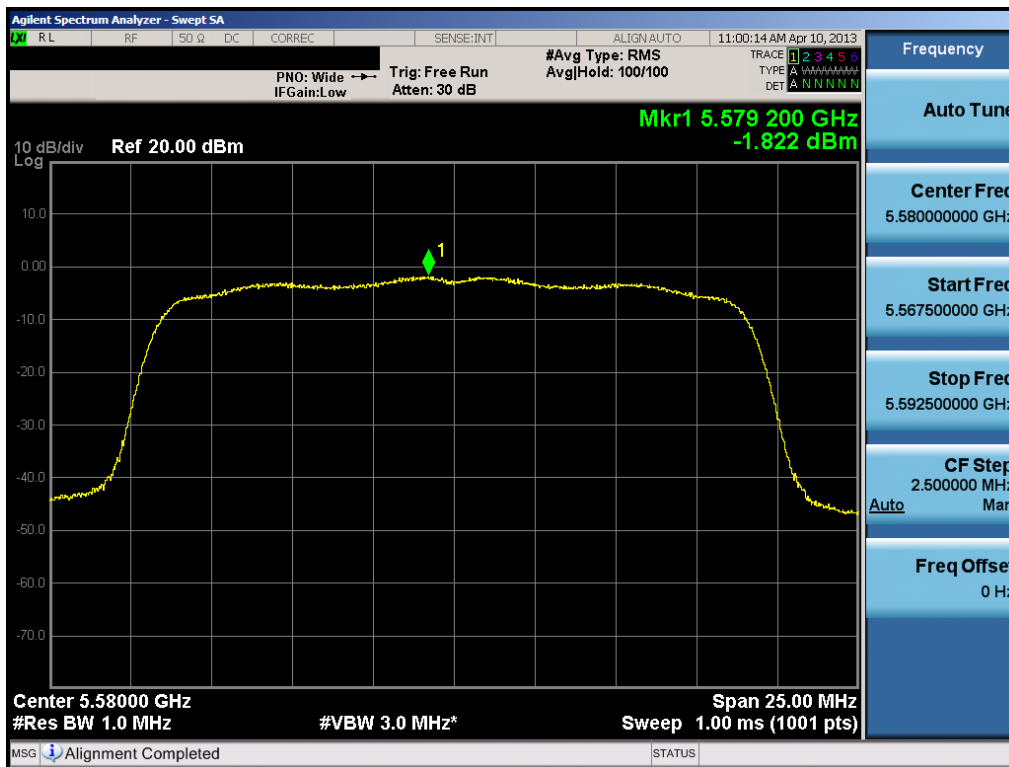
Plot 6-47. Peak Power Spectral Density Plot (20MHz BW 802.11n (UNII Band 3) – Ch. 116)
