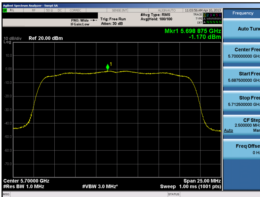
Plot 6-48. Peak Power Spectral Density Plot (20MHz BW 802.11a/n (UNII Band 3) – Ch. 140)
