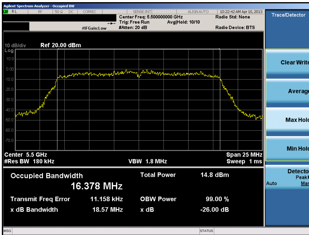
Plot 6-17. 26dB Bandwidth Plot (802.11a (UNII Band 3) – Ch. 100)
