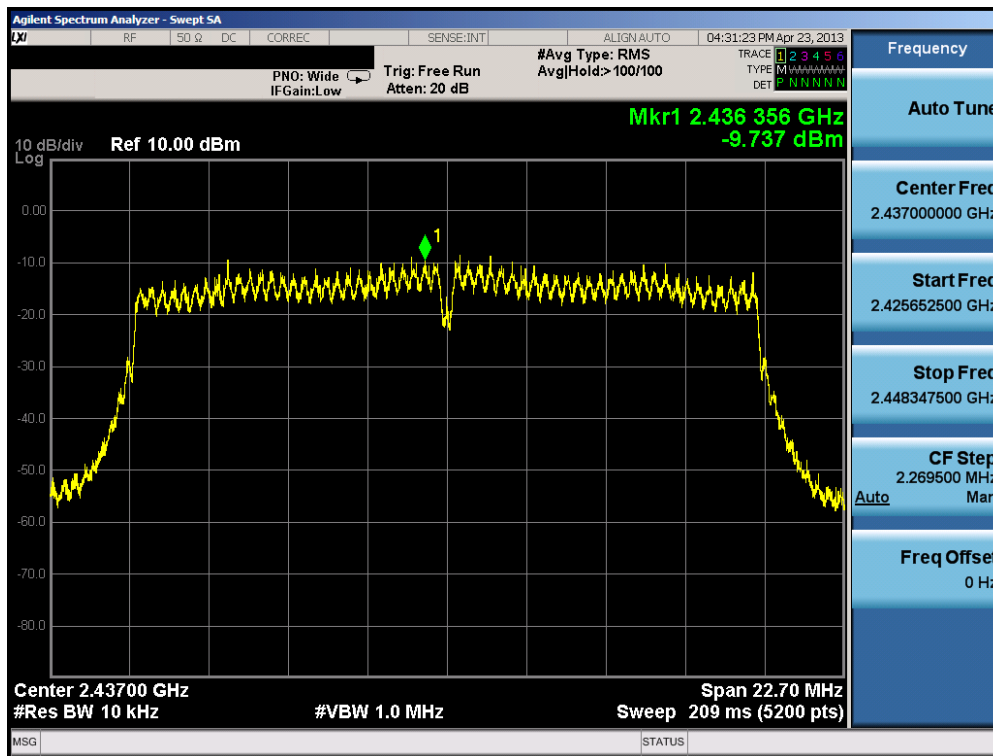
Plot 6-25. Power Spectral Density Plot (802.11n (2.4GHz) – Ch. 6)
