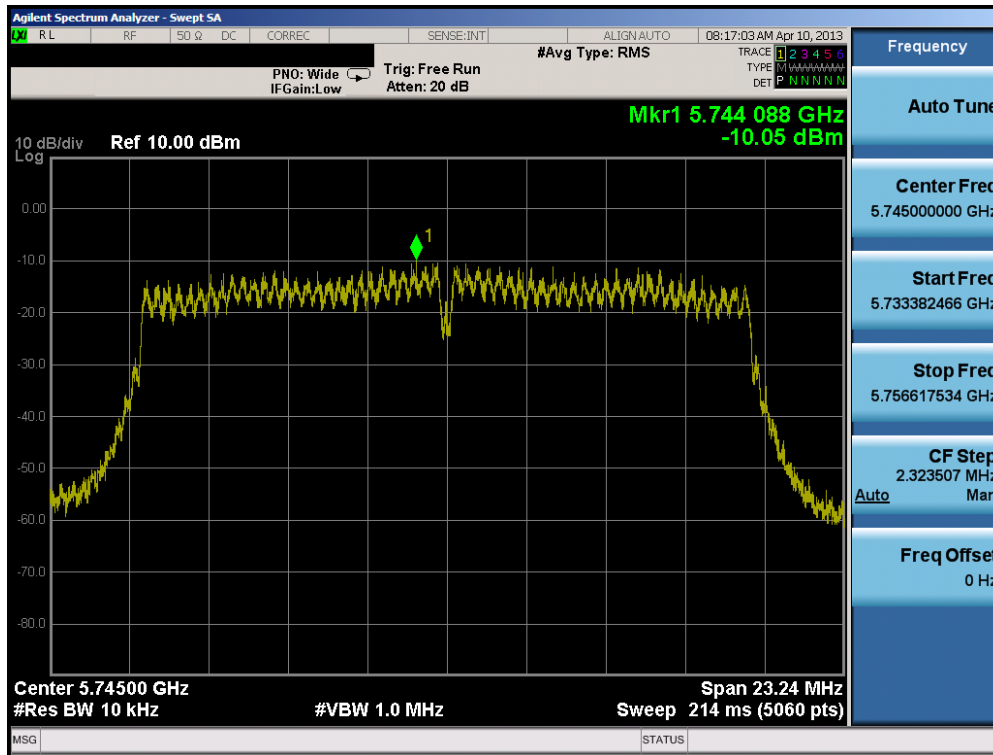
Plot 6-30. Power Spectral Density Plot (20MHz BW 802.11n (5.8GHz) – Ch. 149)
