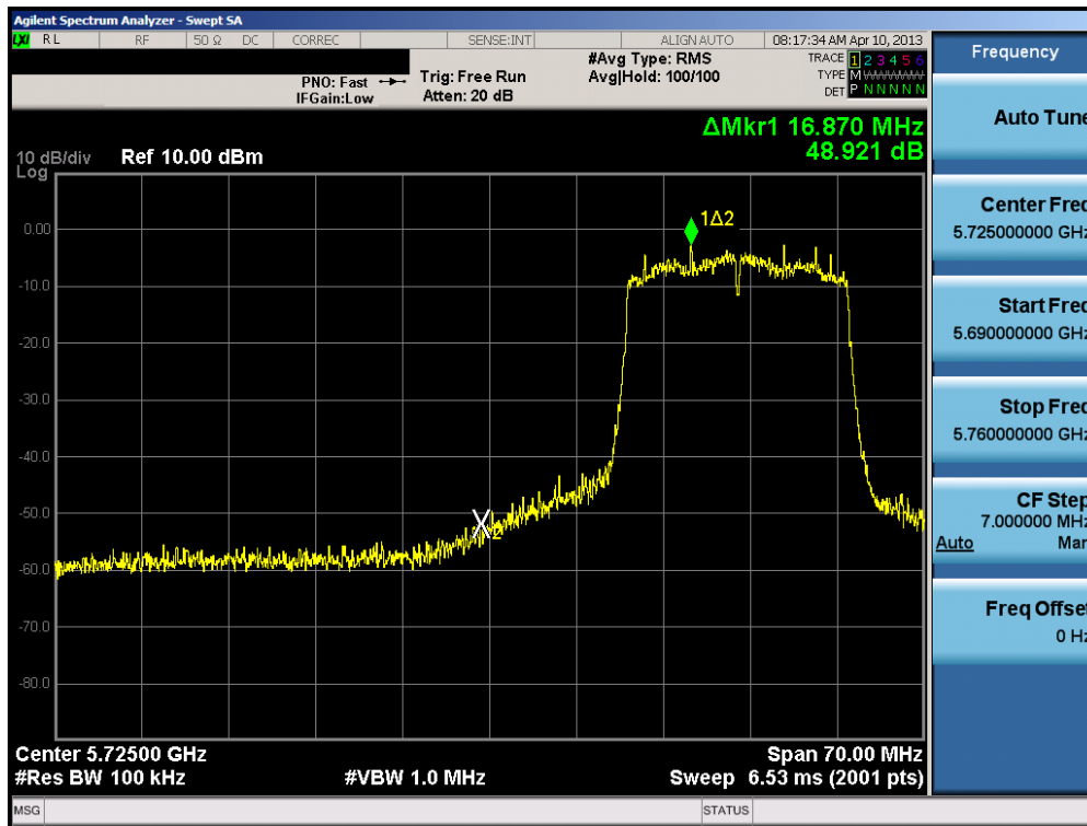
Plot 6-43. Band Edge Plot (20MHz BW 802.11n (5.8GHz) – Ch. 149)
