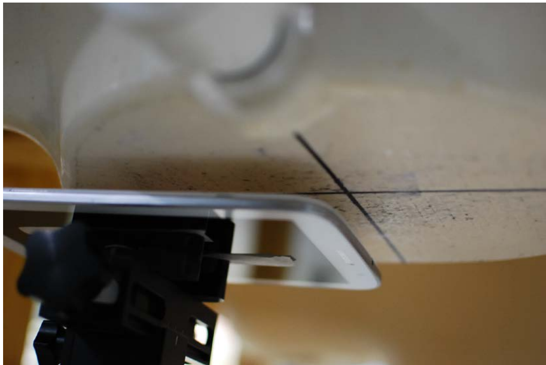
SAR Test Setup Photo 2: Back at 15 mm
