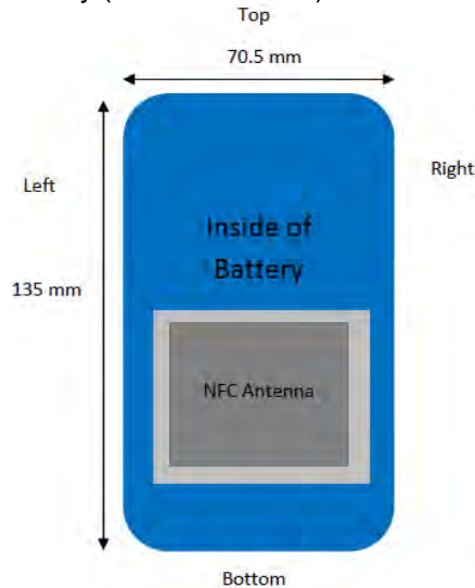
Figure 1-2 NFC Antenna Locations
