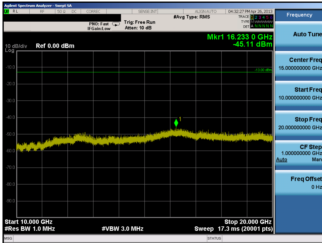
Plot 9-30. Conducted Spurious Plot (20.0MHz QPSK – RB Size 1, RB Offset 0 – Low Channel)
