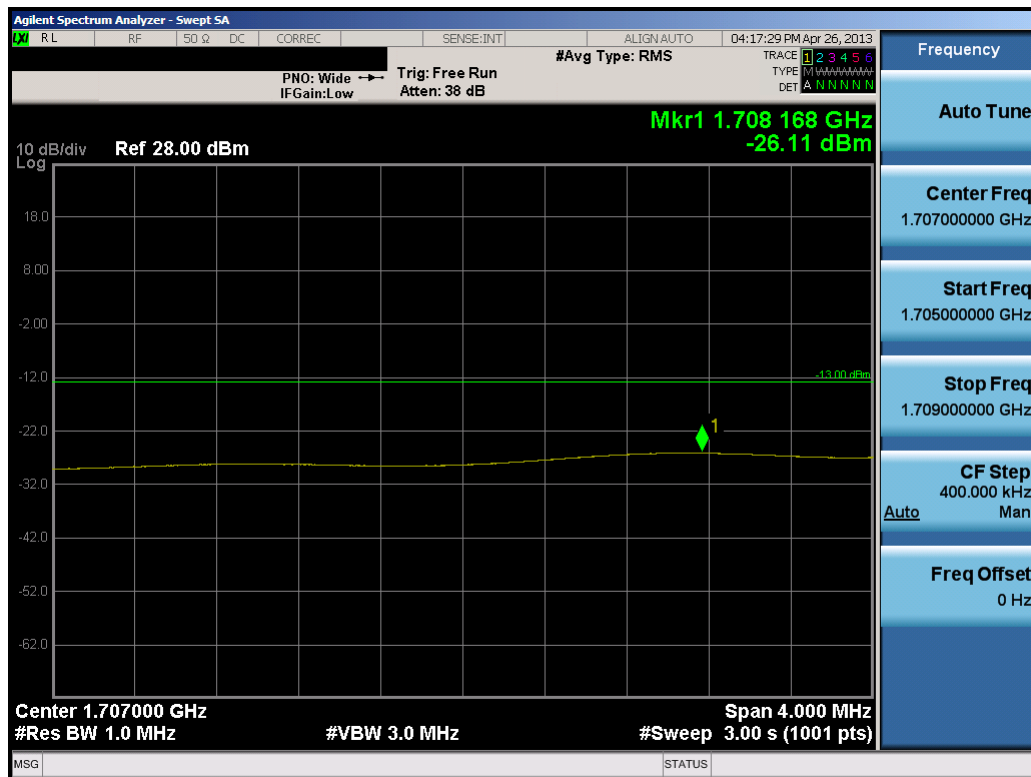
Plot 9-18. Lower Extended Band Edge Plot (15.0MHz QPSK – RB Size 75)
