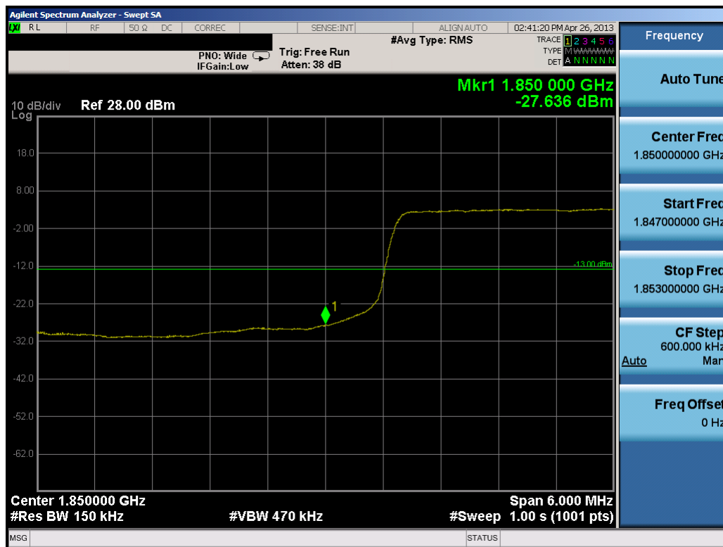
Plot 10-23. Lower Band Edge Plot (15.0MHz QPSK – RB Size 75)
