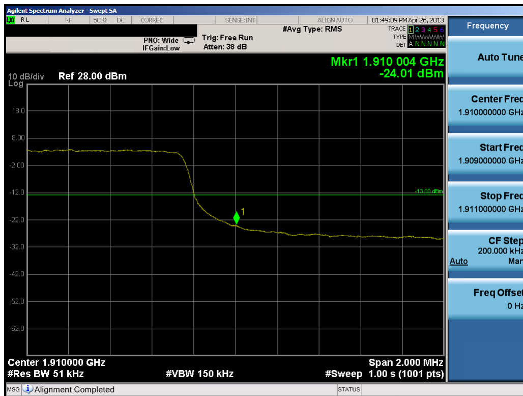
Plot 10-11. Upper Band Edge Plot (5.0MHz QPSK – RB Size 25)
