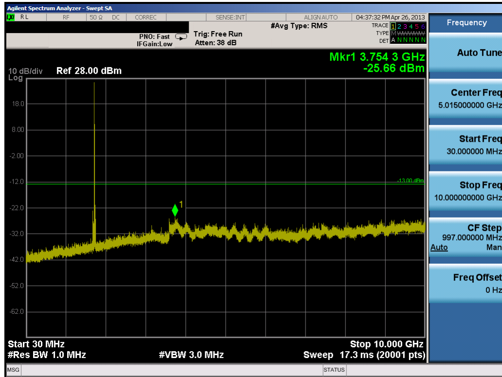
Plot 9-33. Conducted Spurious Plot (20.0MHz QPSK – RB Size 1, RB Offset 0 – High Channel)
