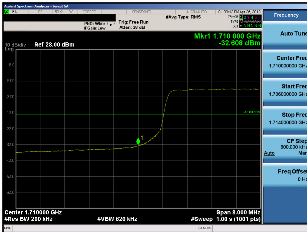
Plot 9-25. Lower Band Edge Plot (20.0MHz QPSK – RB Size 100)
