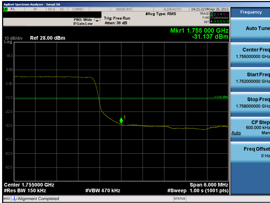
Plot 9-21. Upper Band Edge Plot (15.0MHz QPSK – RB Size 75)
