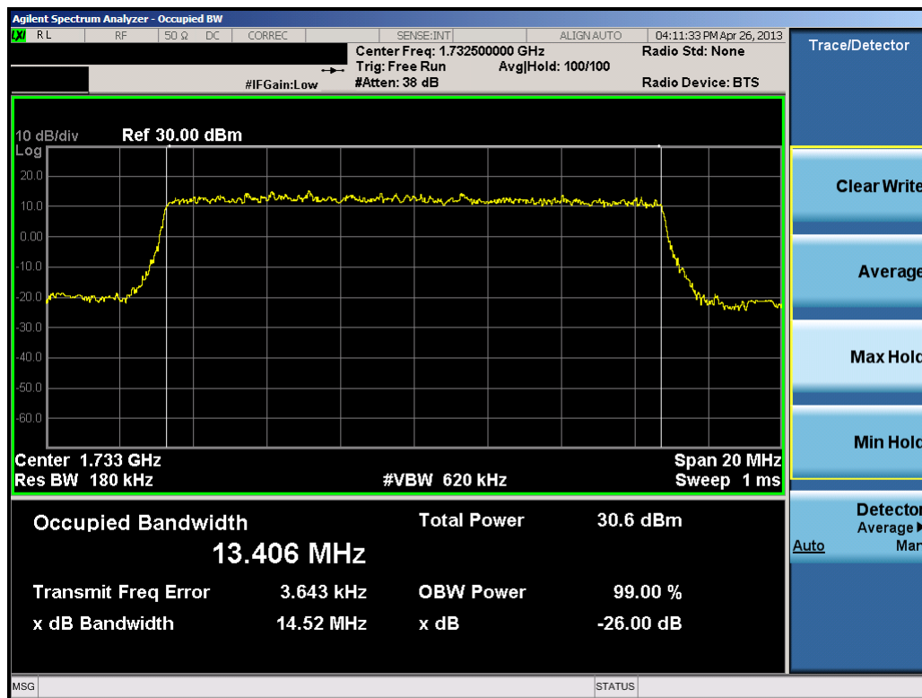
Plot 9-19. Occupied Bandwidth Plot (15.0MHz QPSK – RB Size 75)
