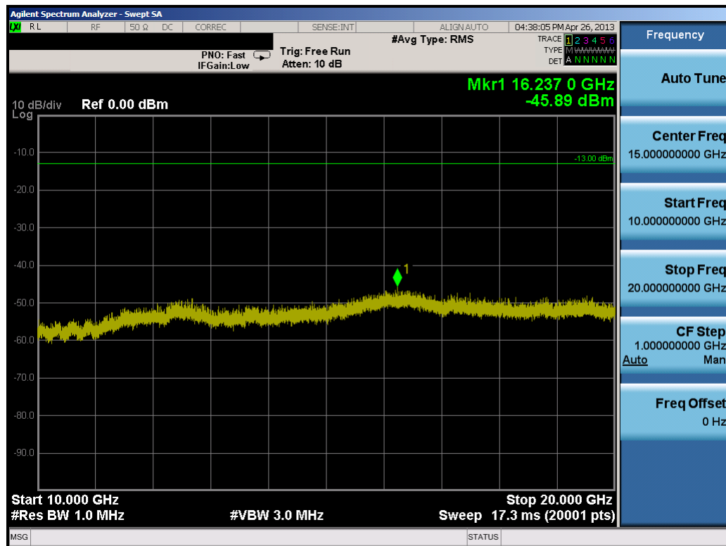
Plot 9-34. Conducted Spurious Plot (20.0MHz QPSK – RB Size 1, RB Offset 0 – High Channel)
