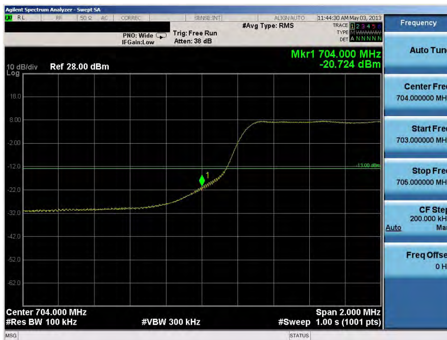
Plot 7-1. Lower Band Edge Plot (5.0MHz QPSK - RB Size 25)
