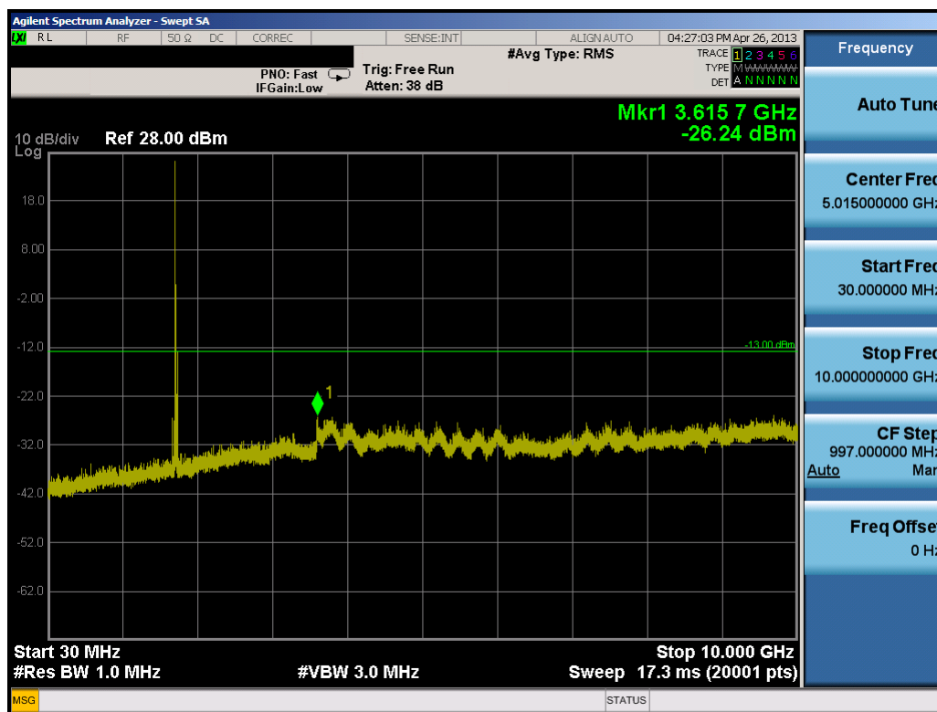
Plot 9-31. Conducted Spurious Plot (20.0MHz QPSK – RB Size 1, RB Offset 0 – Mid Channel)
