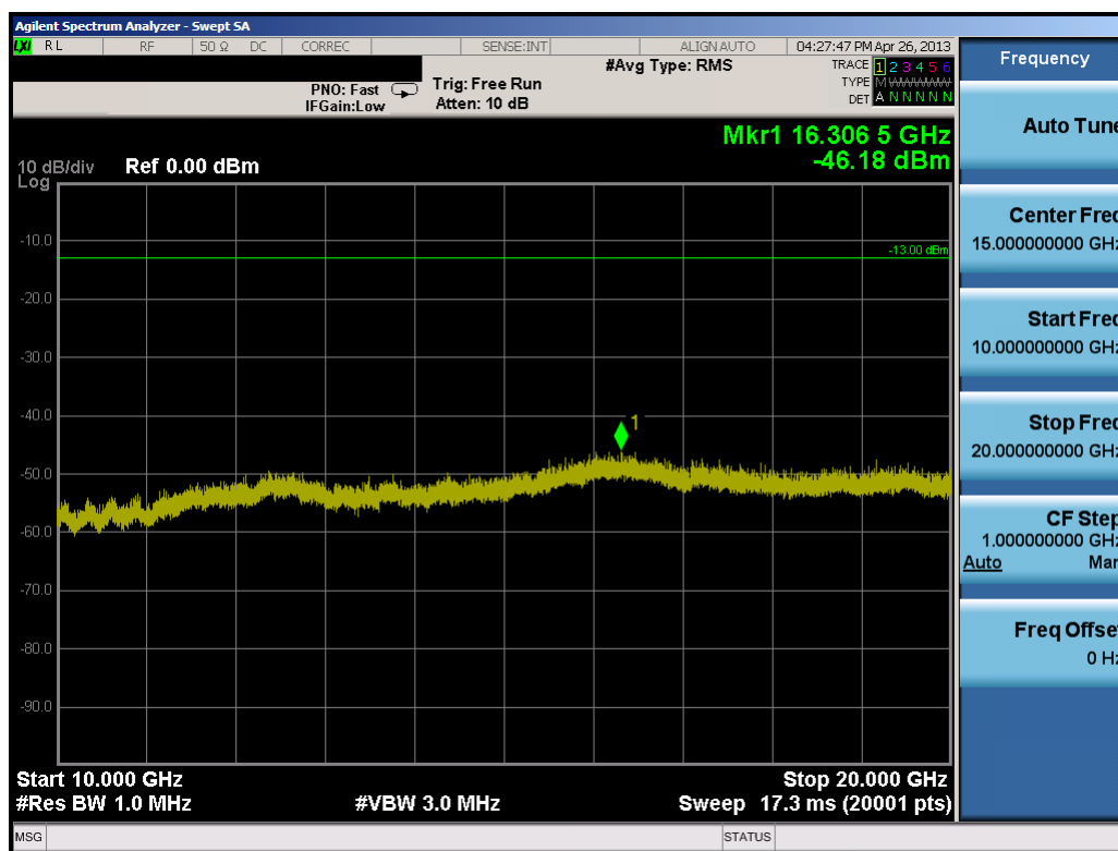
Plot 9-32. Conducted Spurious Plot (20.0MHz QPSK – RB Size 1, RB Offset 0 – Mid Channel)
