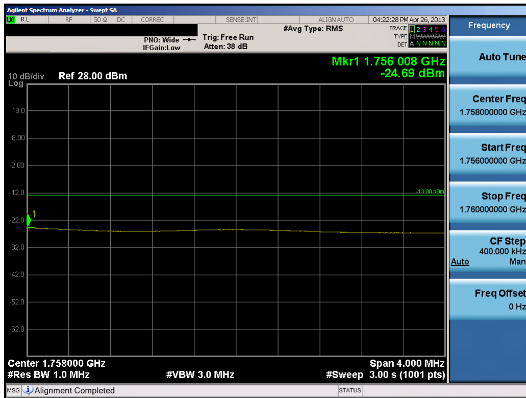
Plot 9-22. Upper Extended Band Edge Plot (15.0MHz QPSK – RB Size 75)
