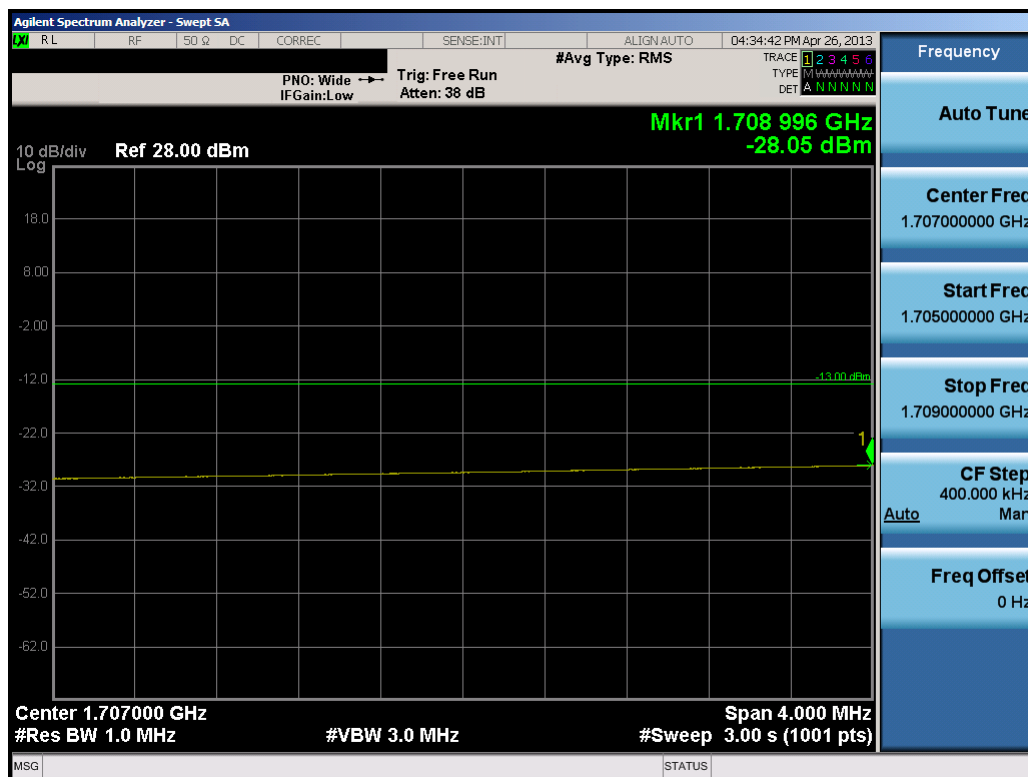
Plot 9-26. Lower Extended Band Edge Plot (20.0MHz QPSK – RB Size 100)
