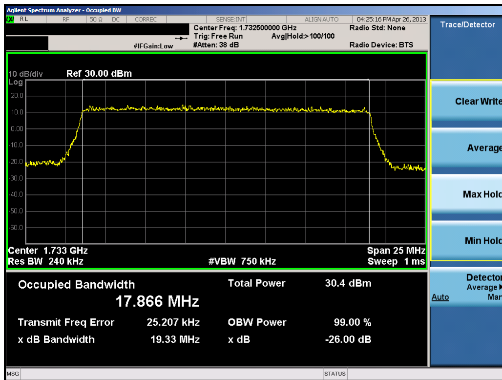
Plot 9-27. Occupied Bandwidth Plot (20.0MHz QPSK – RB Size 100)
