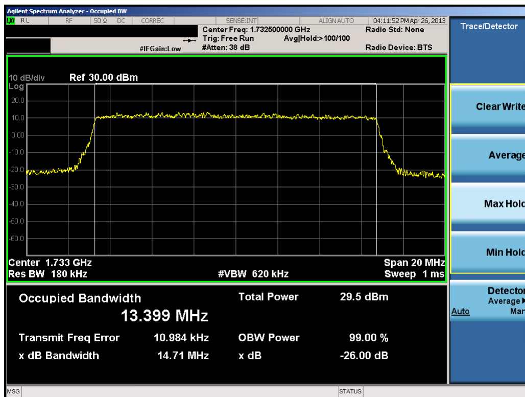
Plot 9-20. Occupied Bandwidth Plot (15.0MHz 16-QAM – RB Size 75)
