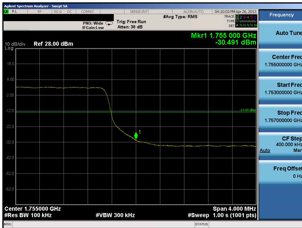
Plot 9-13. Upper Band Edge Plot (10.0MHz QPSK – RB Size 50)
