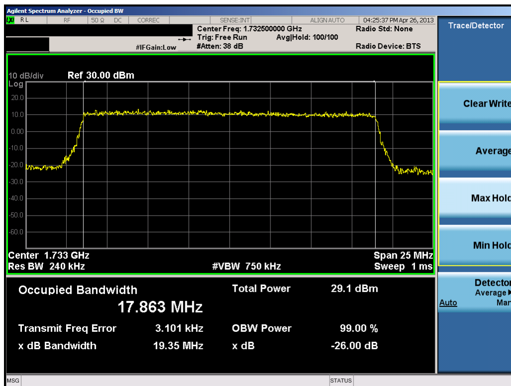
Plot 9-28. Occupied Bandwidth Plot (20.0MHz 16-QAM – RB Size 100)
