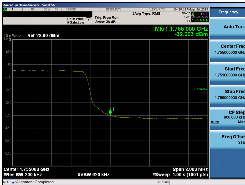
Plot 9-35. Upper Band Edge Plot (20.0MHz QPSK – RB Size 100)
