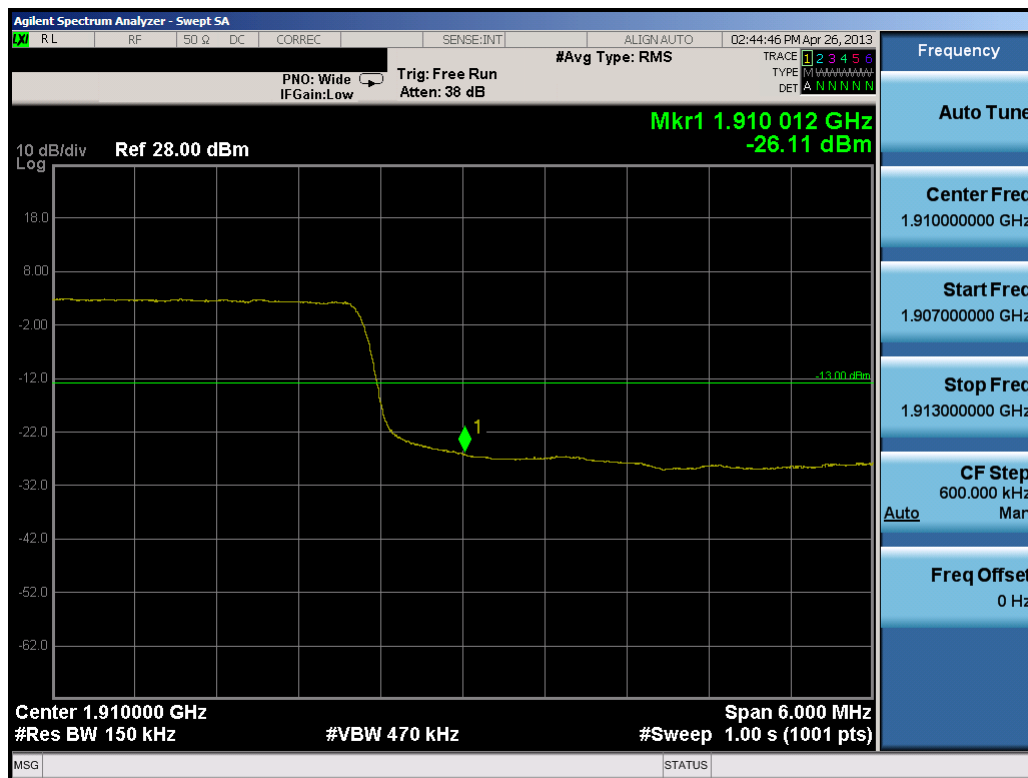
Plot 10-27. Upper Band Edge Plot (15.0MHz QPSK – RB Size 75)
