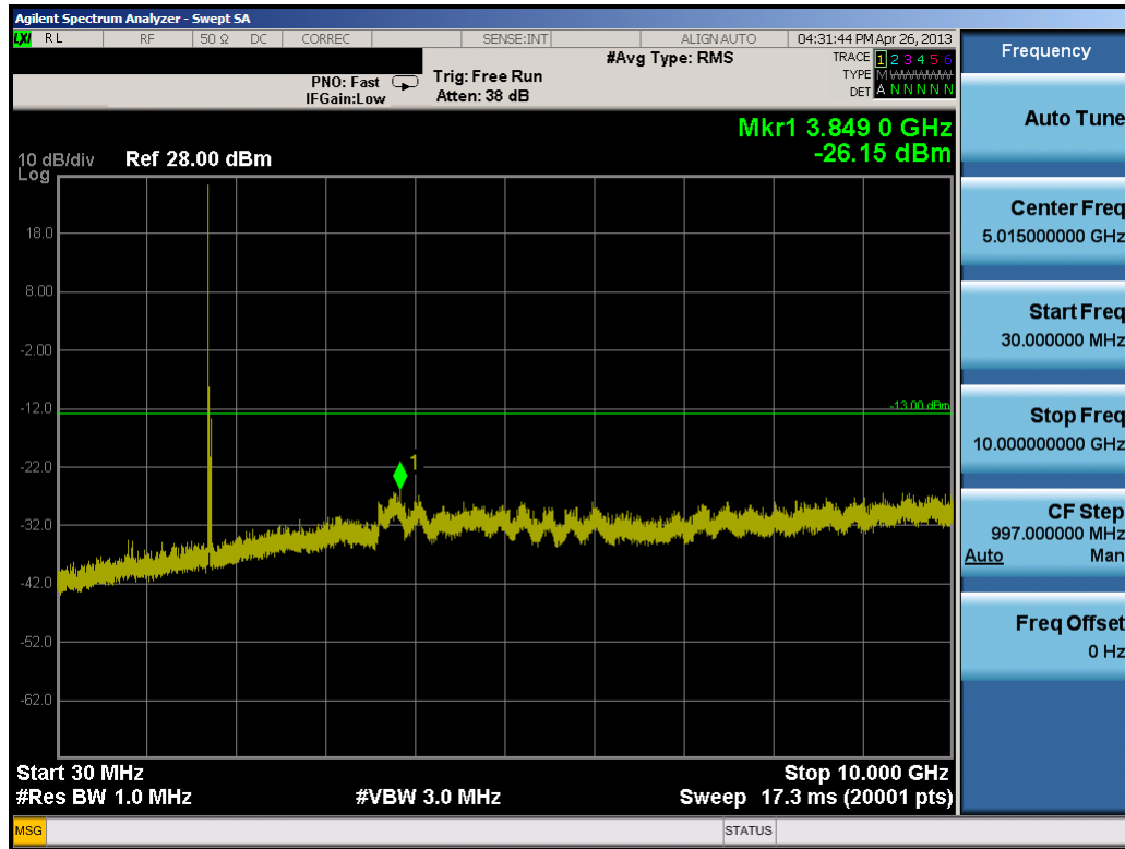
Plot 9-29. Conducted Spurious Plot (20.0MHz QPSK – RB Size 1, RB Offset 0– Low Channel)
