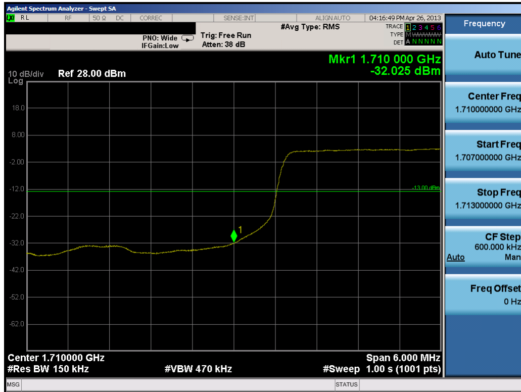
Plot 9-17. Lower Band Edge Plot (15.0MHz QPSK – RB Size 75)
