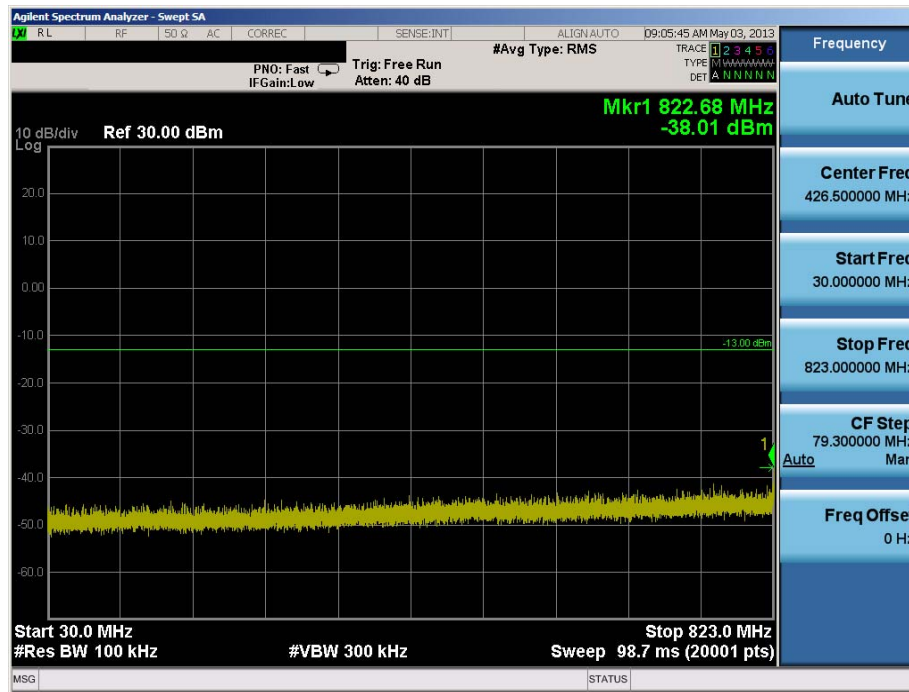
Plot 7-1. Conducted Spurious Plot (Cellular GSM Mode – Ch. 128)
