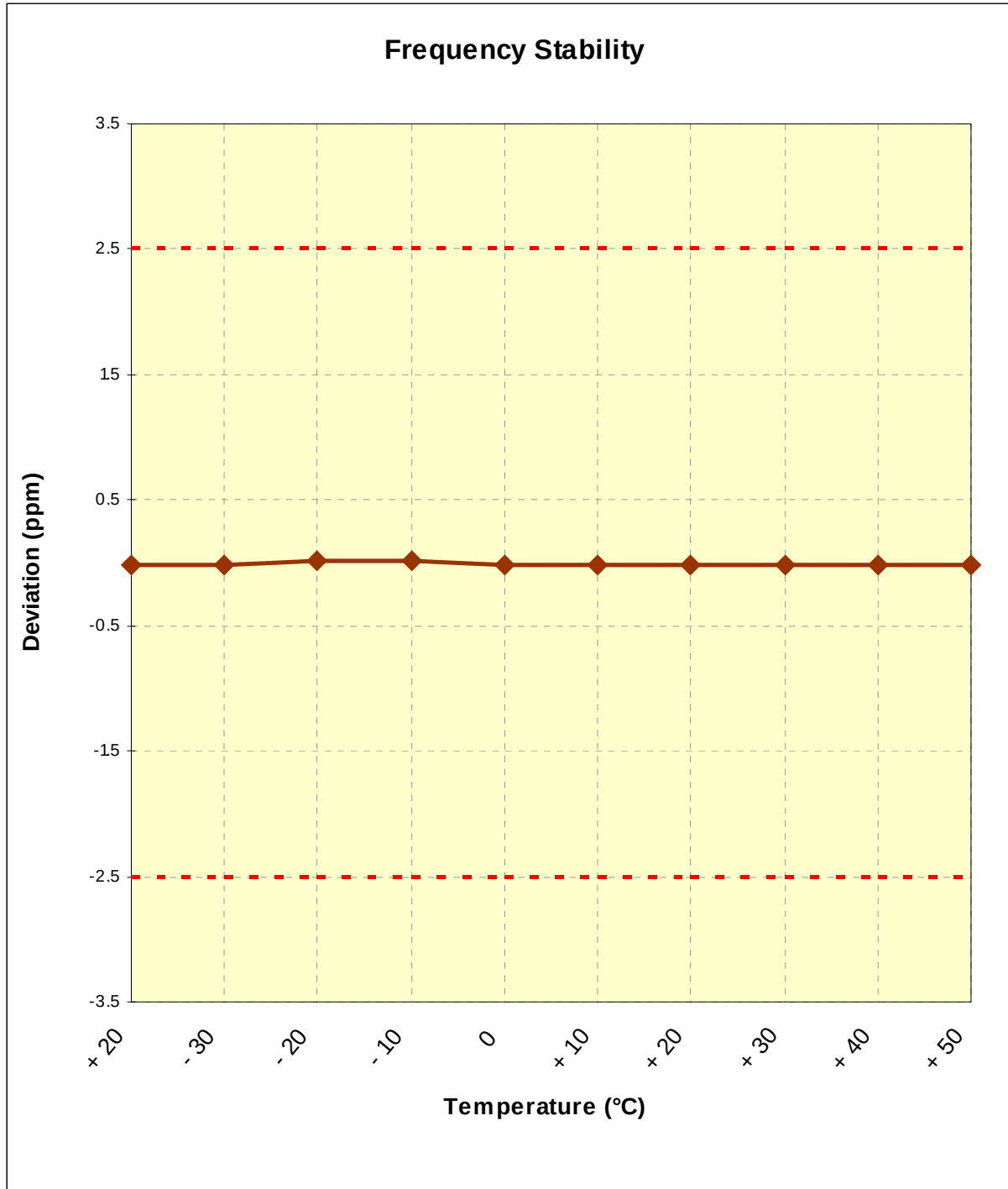
Figure 6-2. Frequency Stability Graph (Cellular WCDMA Mode – Ch. 4183)
