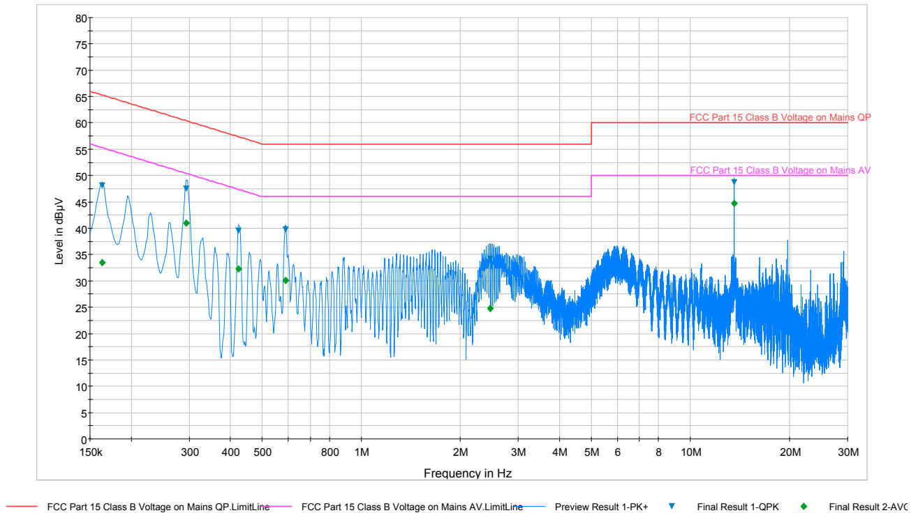
Plot 8-1. Line-Conducted Test Plot (L1)
