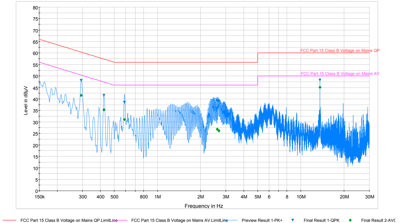
Plot 8-2. Line-Conducted Test Plot (N)
