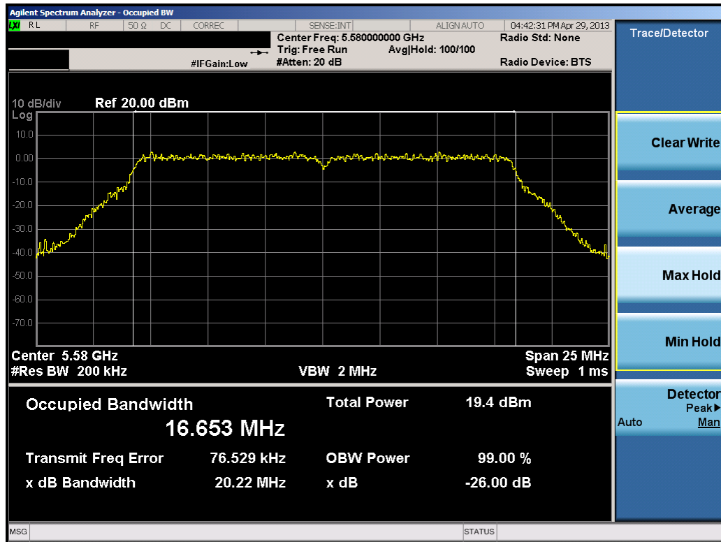
Plot 6-21. 26dB Bandwidth Plot (802.11a (UNII Band 3) – Ch. 116)
