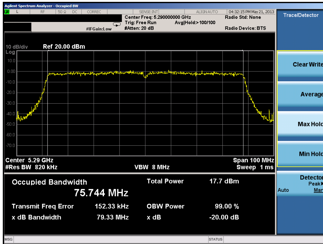
Plot 6-19. 20dB Bandwidth Plot (80MHz BW 802.11ac (UNII Band 2) – Ch. 58)
