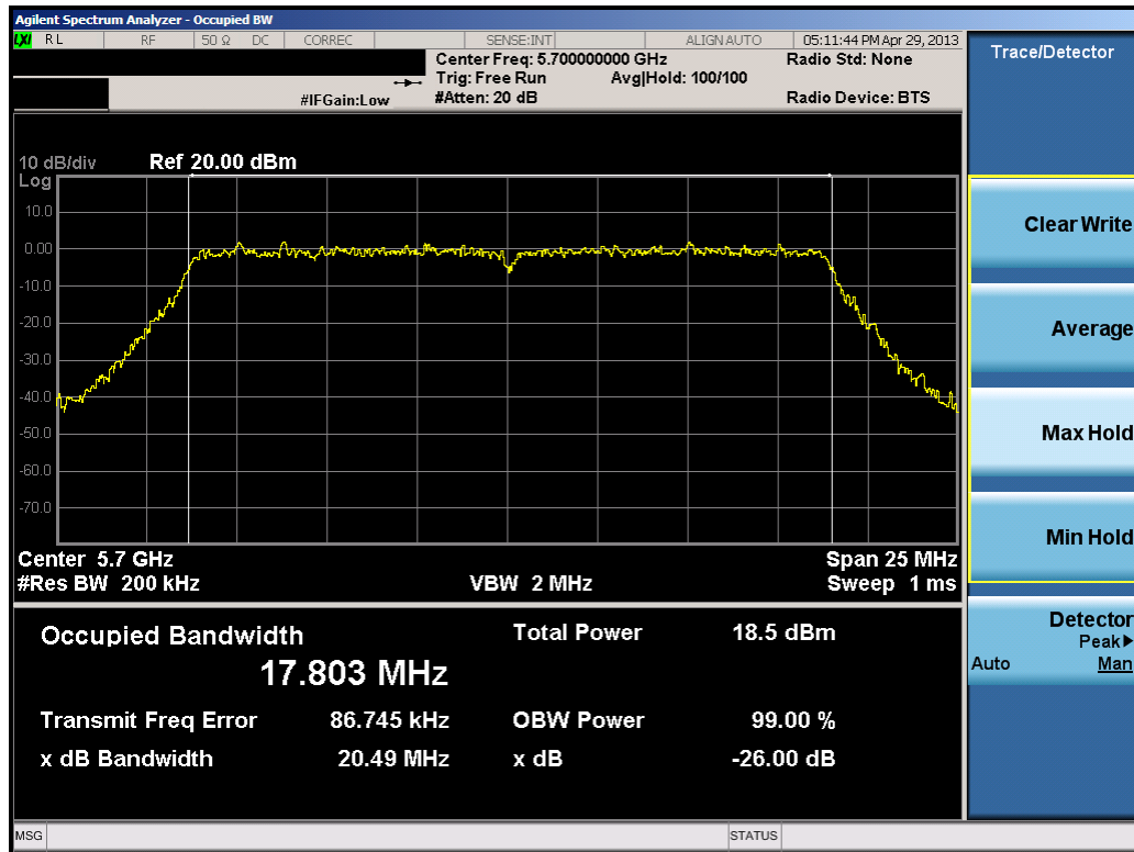
Plot 6-25. 26dB Bandwidth Plot (20MHz BW 802.11n (UNII Band 3) – Ch. 140)
