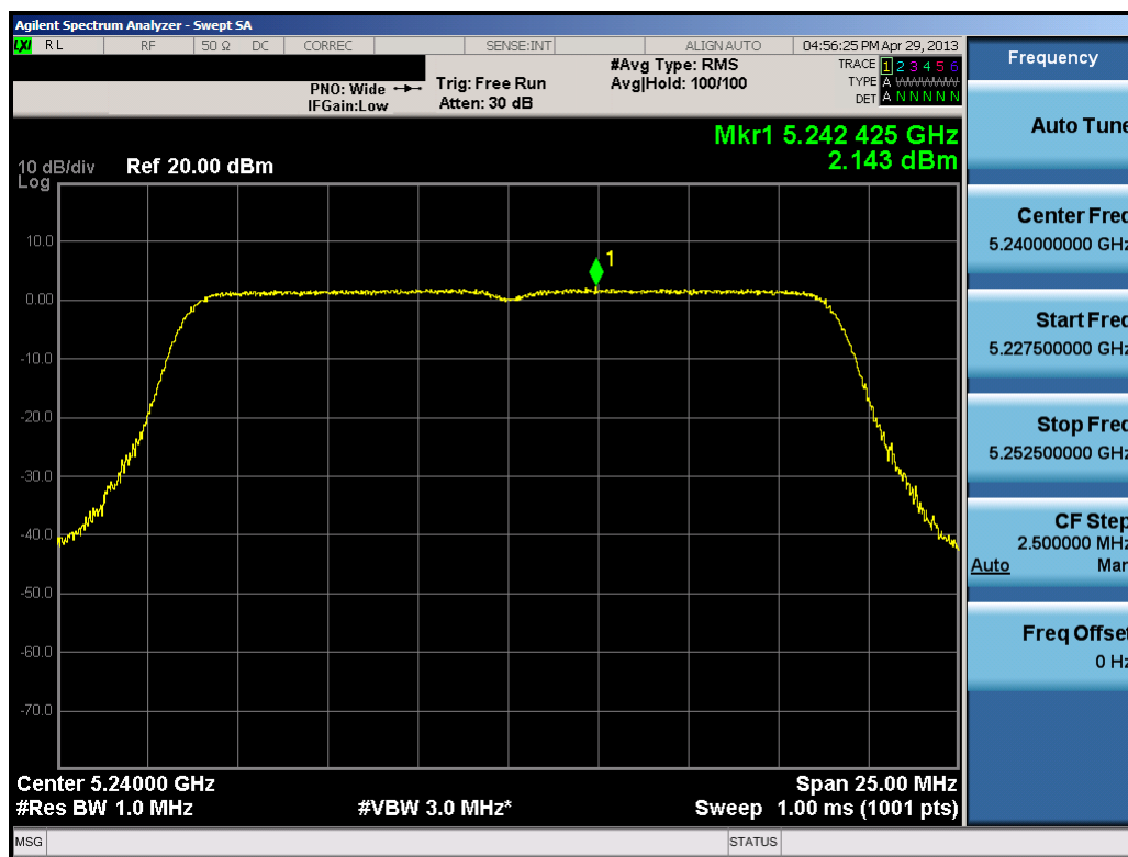
Plot 6-35. Peak Power Spectral Density Plot (20MHz BW 802.11n (UNII Band 1) – Ch. 48)
