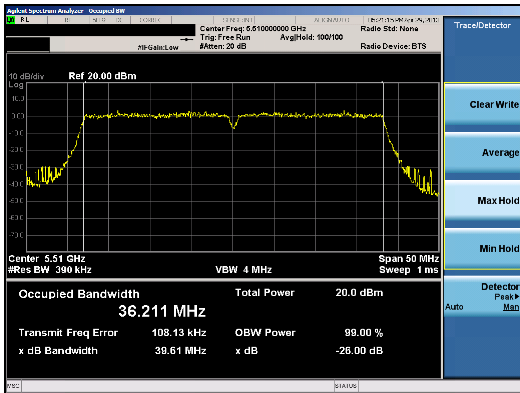
Plot 6-26. 26dB Bandwidth Plot (40MHz BW 802.11n (UNII Band 3) – Ch. 102)
