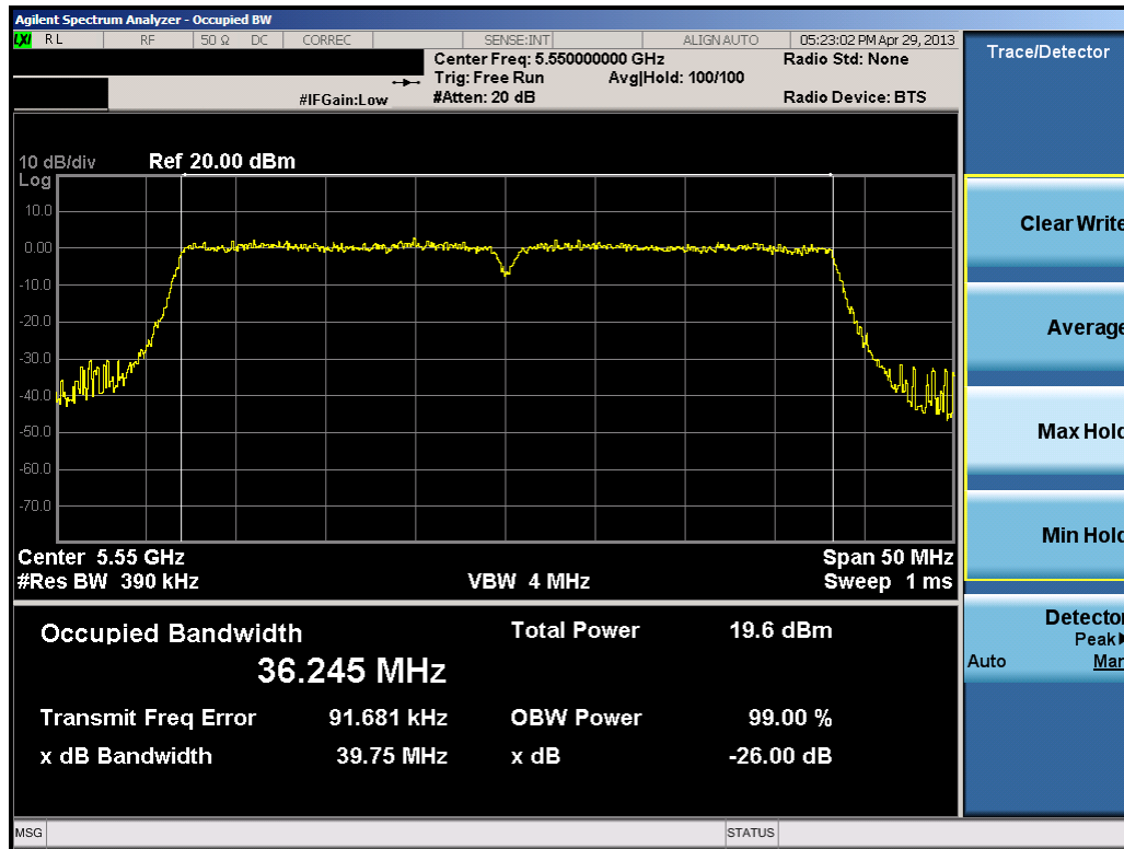
Plot 6-27. 26dB Bandwidth Plot (40MHz BW 802.11n (UNII Band 3) – Ch. 110)
