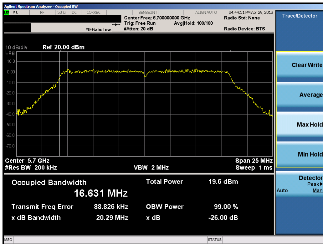
Plot 6-22. 26dB Bandwidth Plot (802.11a (UNII Band 3) – Ch. 140)
