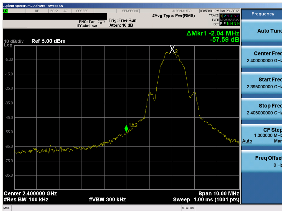
Plot 6-7. Band Edge Plot (Bluetooth (LE) – Ch. 0)
