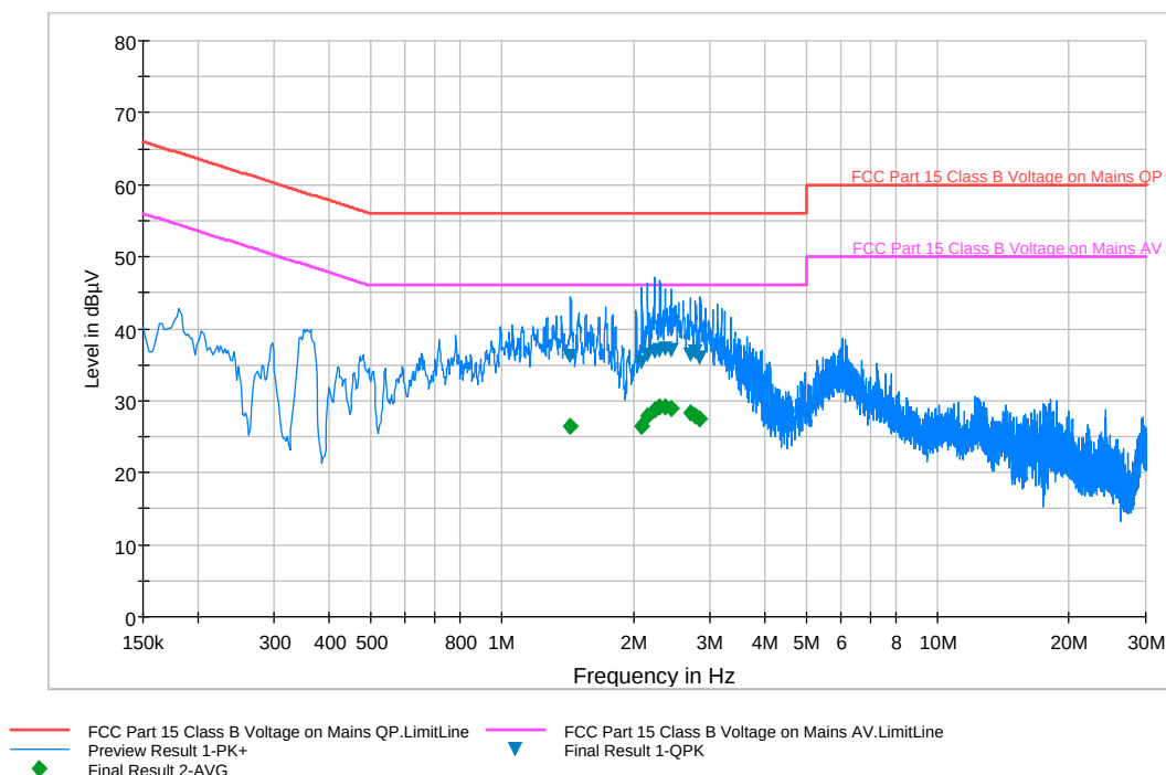
Plot 6-15. Line Conducted Plot with Bluetooth LE (L1)
