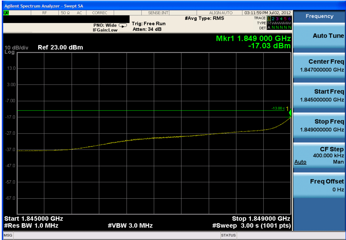
Plot 7-37. Extended Band Edge Span Plot (PCS WCDMA Mode – Ch. 9262)
