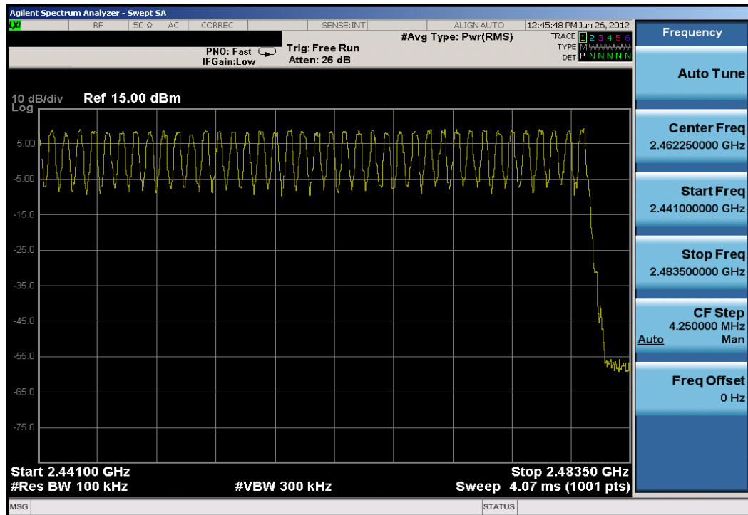
Plot 6-17. High End Spectrum Channel Hopping Plot (Bluetooth)
