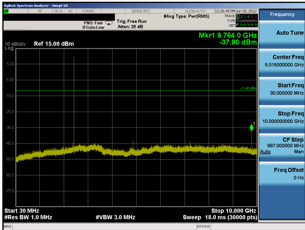
Plot 6-20. Conducted Spurious Plot (Bluetooth, 3Mbps – Ch. 39)
