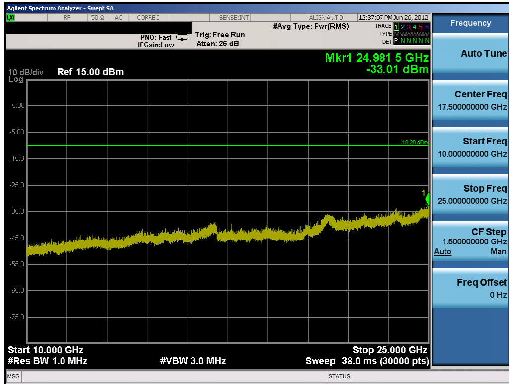
Plot 6-19. Conducted Spurious Plot (Bluetooth, 3Mbps – Ch. 0)
