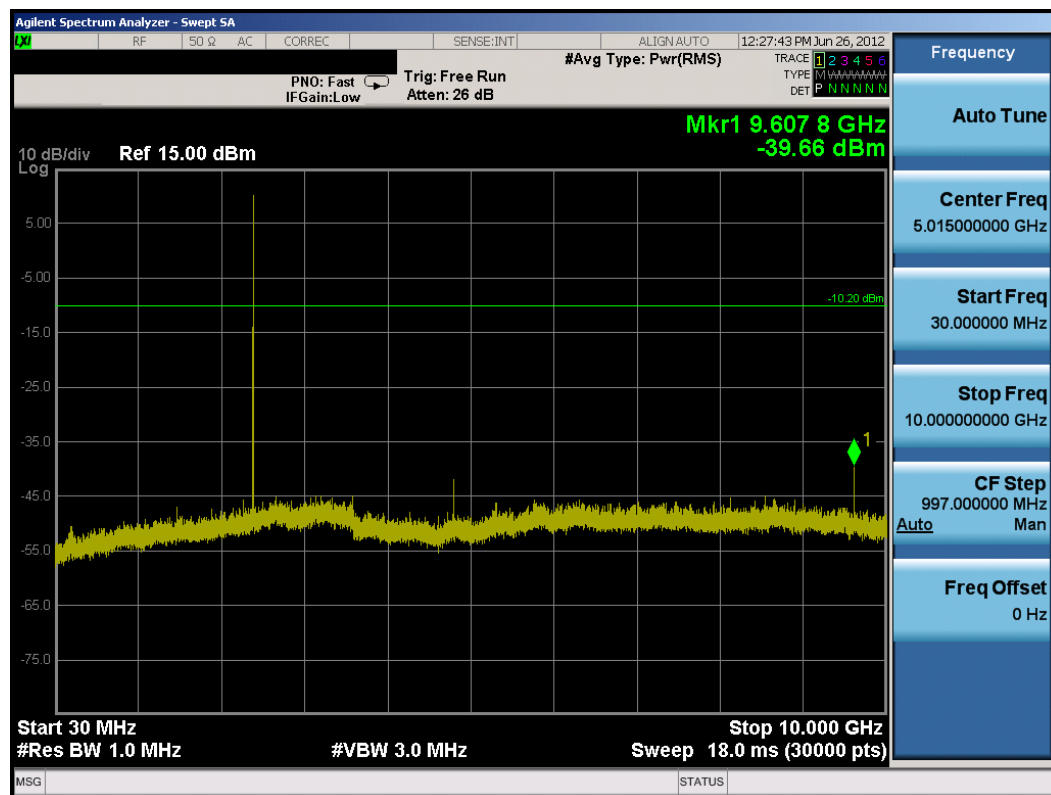
Plot 6-18. Conducted Spurious Plot (Bluetooth, 3Mbps – Ch. 0)
