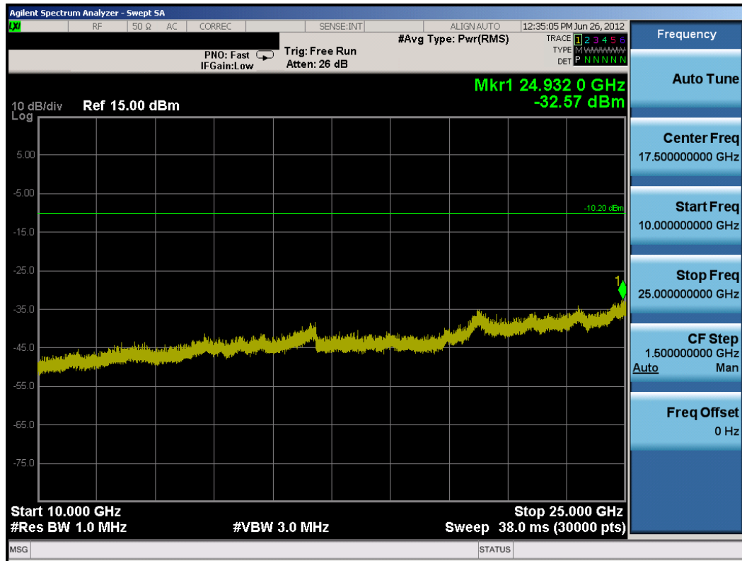
Plot 6-23. Conducted Spurious Plot (Bluetooth, 3Mbps – Ch. 78)
