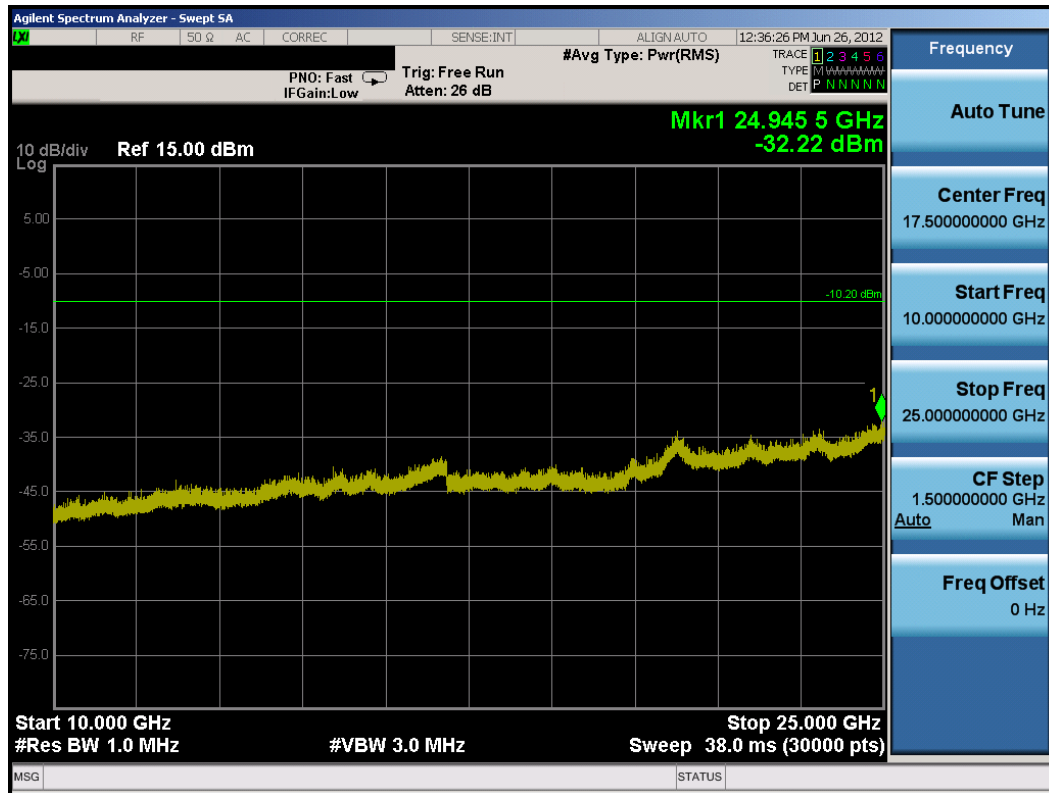
Plot 6-21. Conducted Spurious Plot (Bluetooth, 3Mbps – Ch. 39)
