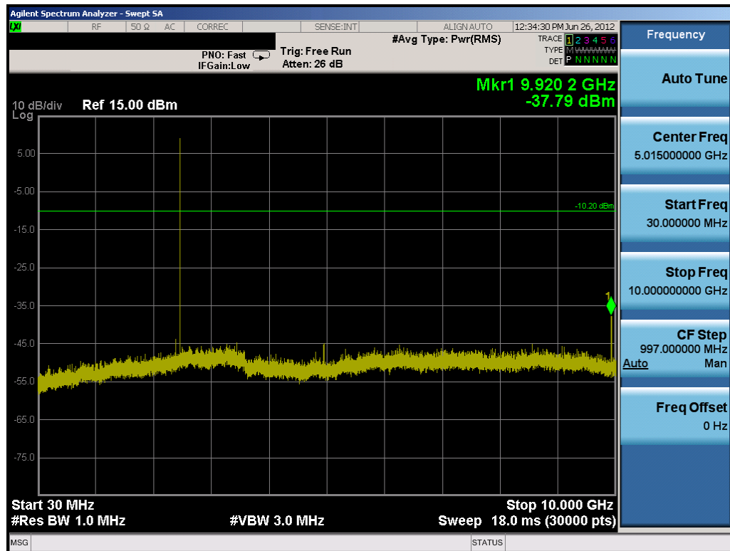
Plot 6-22. Conducted Spurious Plot (Bluetooth, 3Mbps – Ch. 78)
