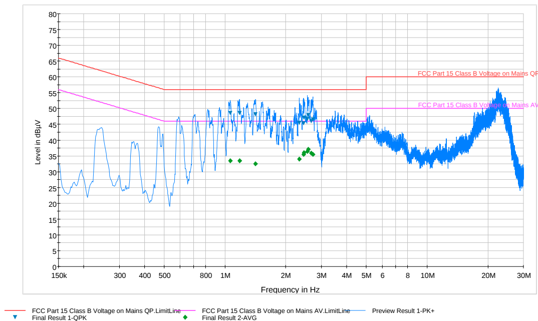
Plot 6-32. Line Conducted Plot with 802.11b (N)
