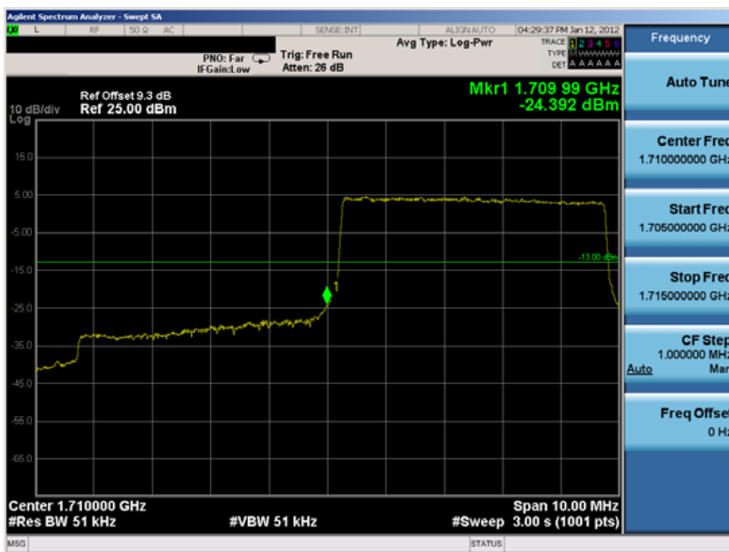
Plot 8-9. Band Edge Plot (5MHz BW, QPSK RB Size = 25 Offset = 0, Low Channel)
