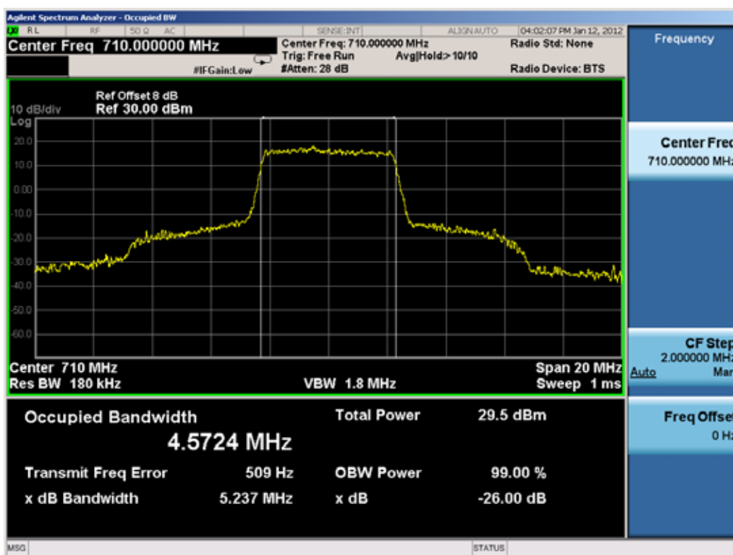
Plot 7-9. Occupied Bandwidth Plot (5MHz BW, QPSK RB Size = 25, Offset = 0)
