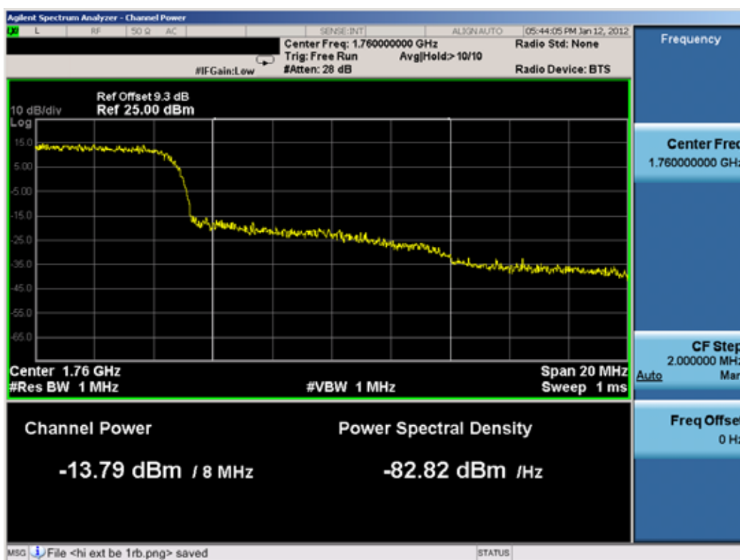
Plot 8-27. Extended Band Edge Plot (10MHz BW, QPSK RB Size = 50 Offset = 0, High Channel)
