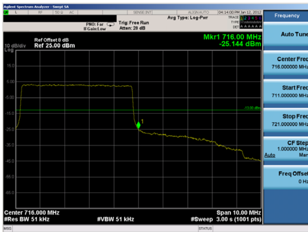
Plot 7-13. Upper Band Edge Plot (5MHz BW, QPSK RB Size = 25, Offset = 0)
