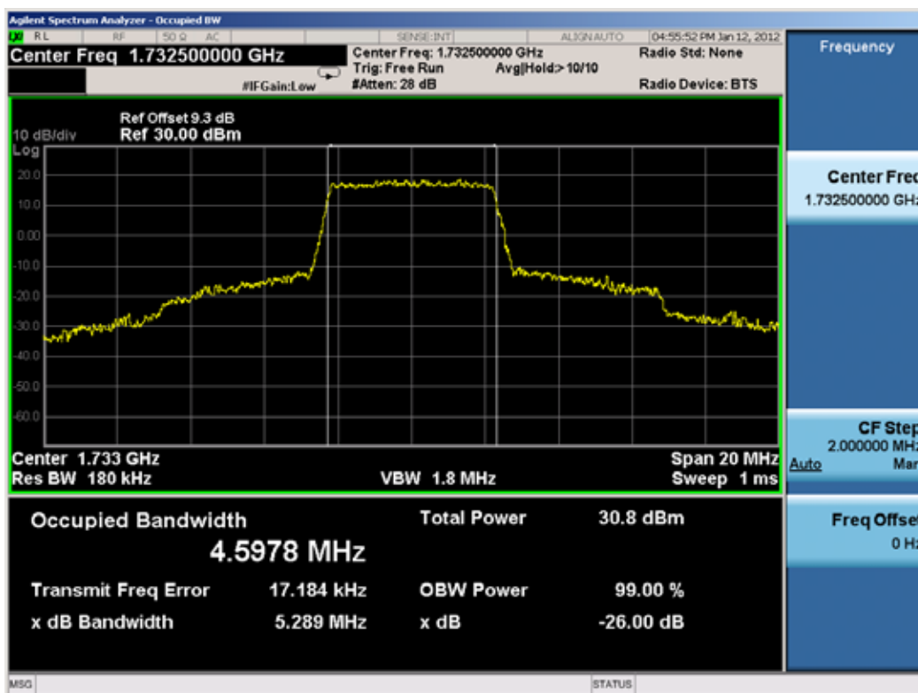
Plot 8-17. Occupied Bandwidth Plot (5MHz BW, QPSK RB Size = 25 Offset = 0)
