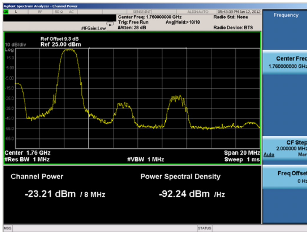
Plot 8-28. Extended Band Edge Plot (10MHz BW, QPSK RB Size = 1 Offset = 49, High Channel)
