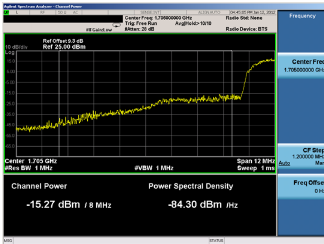
Plot 8-14. Extended Band Edge Plot (5MHz BW, QPSK RB Size = 25 Offset = 0)
