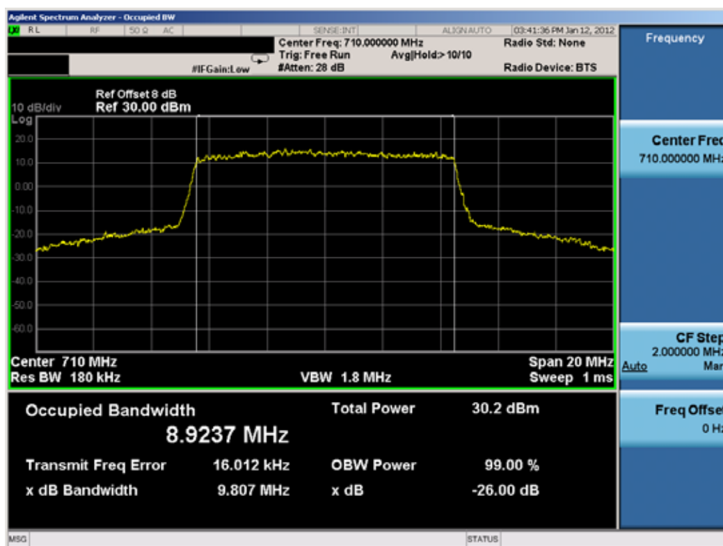
Plot 7-7. Occupied Bandwidth Plot (10MHz BW, QPSK RB Size = 50, Offset = 0)
