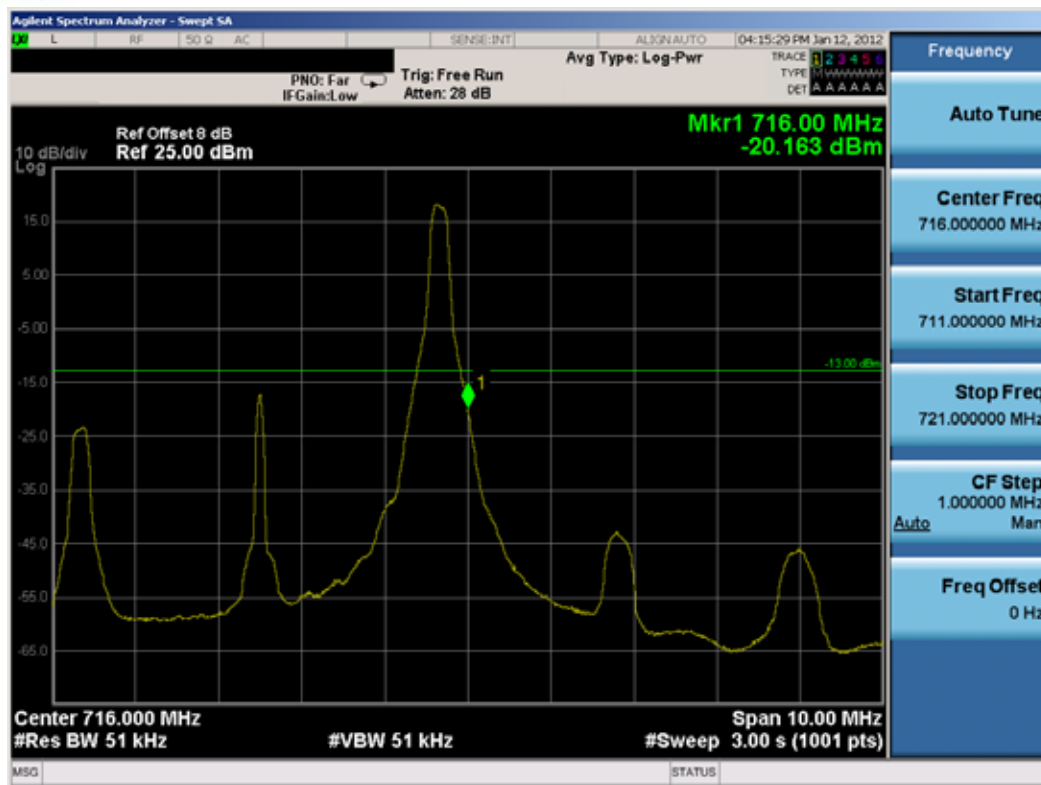
Plot 7-14. Upper Band Edge Plot (5MHz BW, QPSK RB Size = 1, Offset = 24)
