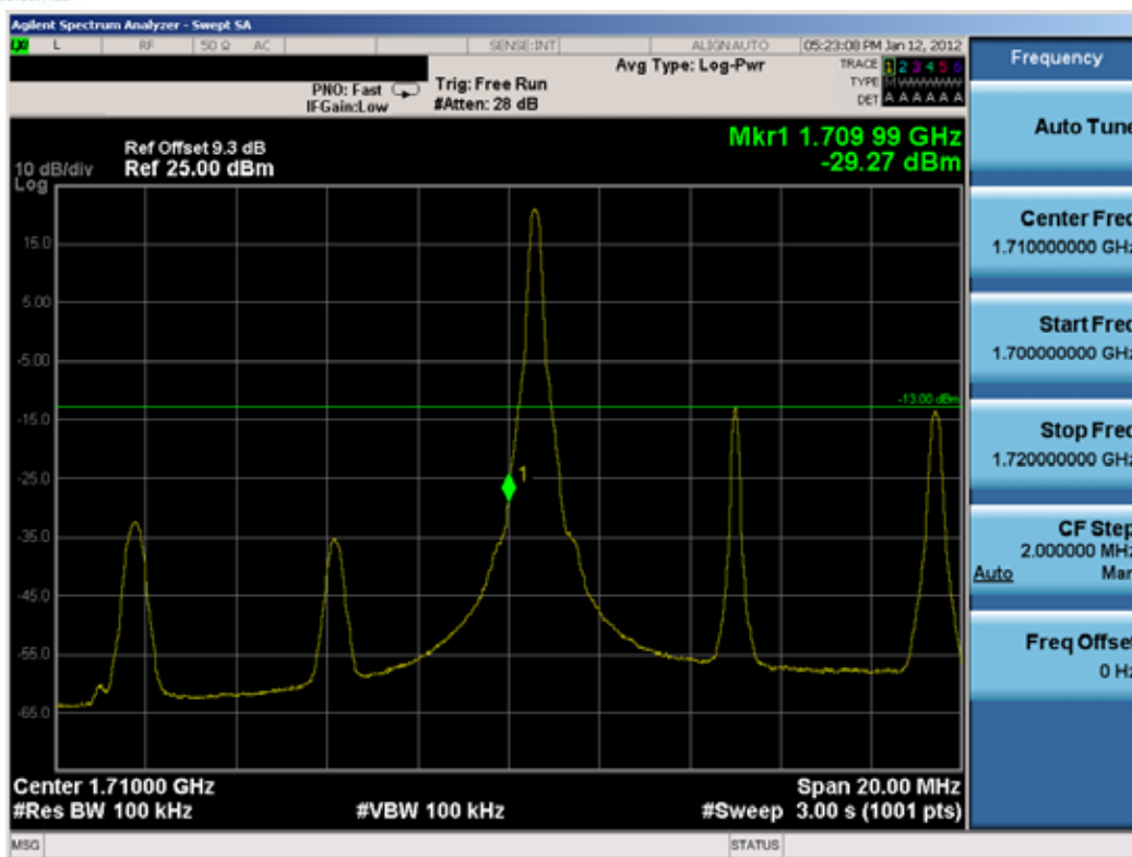
Plot 8-8. Band Edge Plot (10MHz BW, QPSK RB Size = 1 Offset = 0, Low Channel)
