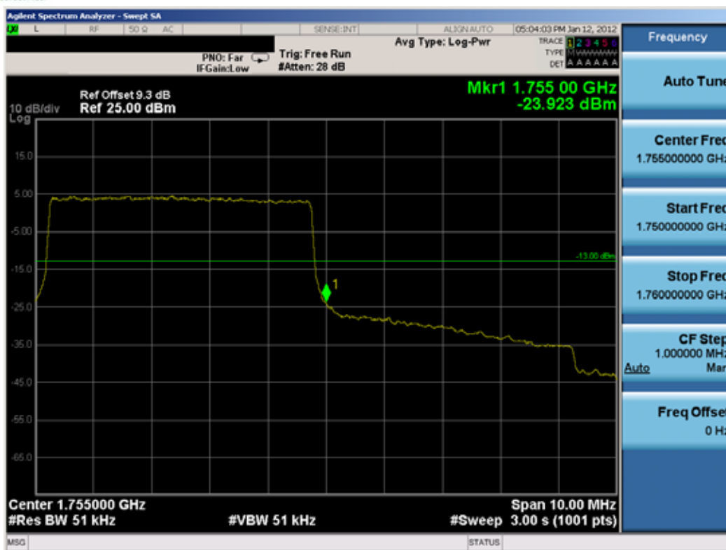
Plot 8-26. Band Edge Plot (5MHz BW, QPSK RB Size = 25 Offset = 0, High Channel)
