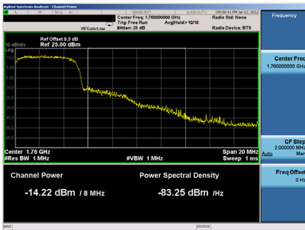
Plot 8-29. Extended Band Edge Plot (5MHz BW, QPSK RB Size = 25 Offset = 0, High Channel)
