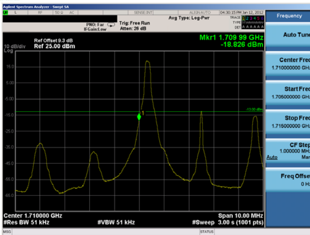
Plot 8-10. Band Edge Plot (5MHz BW, QPSK RB Size = 1 Offset = 0, Low Channel)
