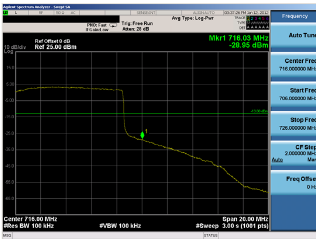
Plot 7-11. Upper Band Edge Plot (10 MHz BW, QPSK RB Size = 50, Offset = 0)
