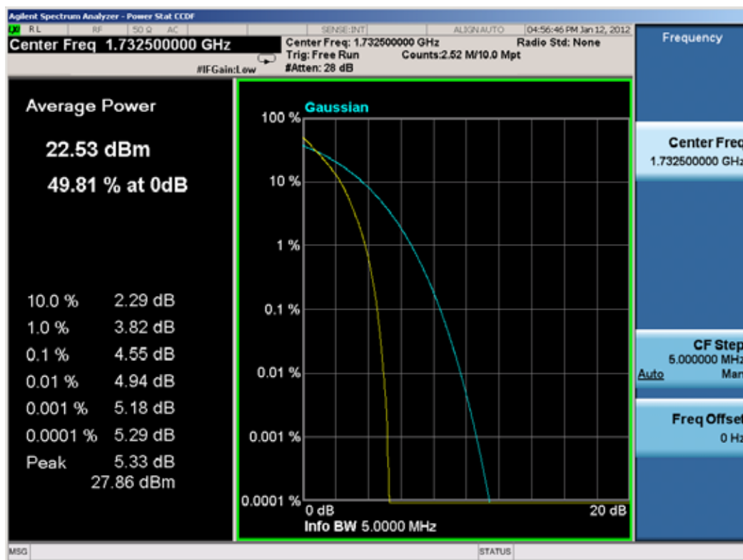
Plot 8-21. Peak-Average Ratio Plot (5MHz BW, QPSK RB Size = 25 RB Offset = 0)
