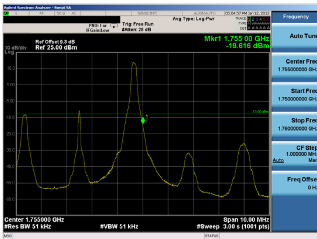
Plot 8-25. Band Edge Plot (5MHz BW, QPSK RB Size = 1 Offset = 24, High Channel)
