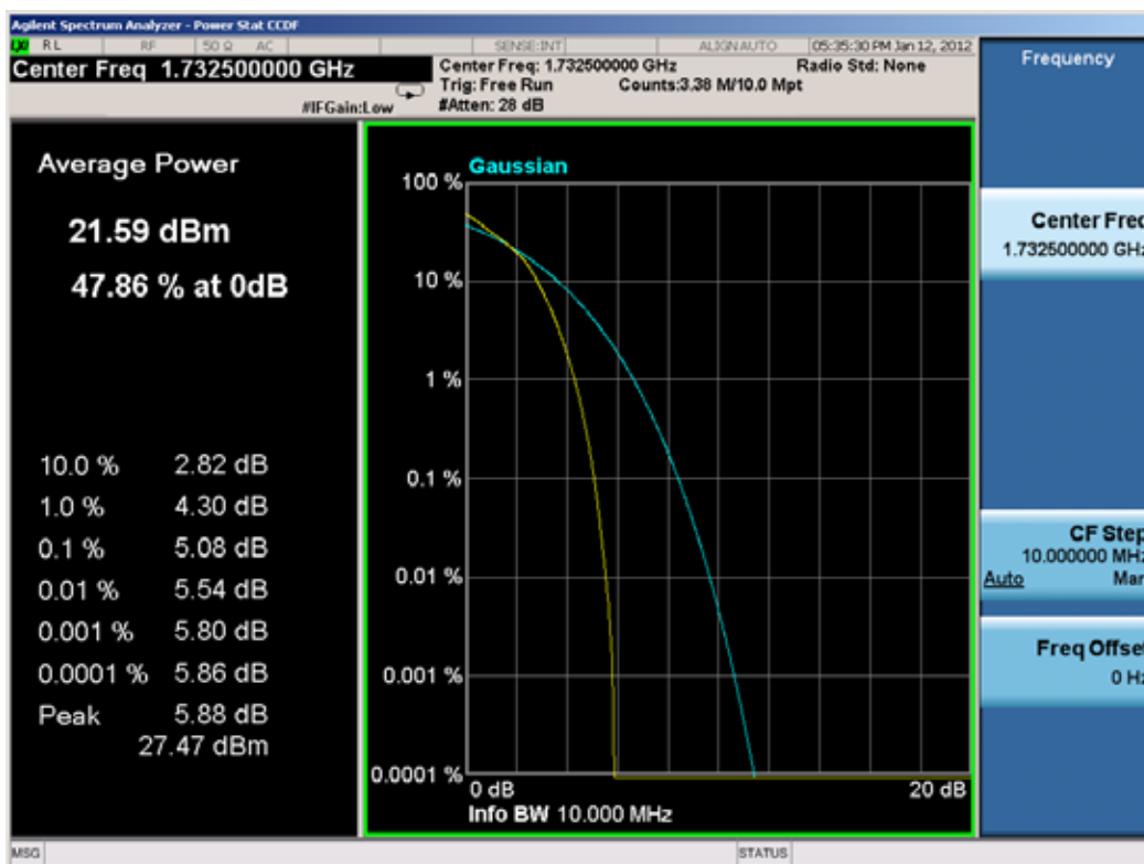
Plot 8-19. Peak-Average Ratio Plot (10MHz BW, QPSK RB Size = 50 RB Offset = 0)
