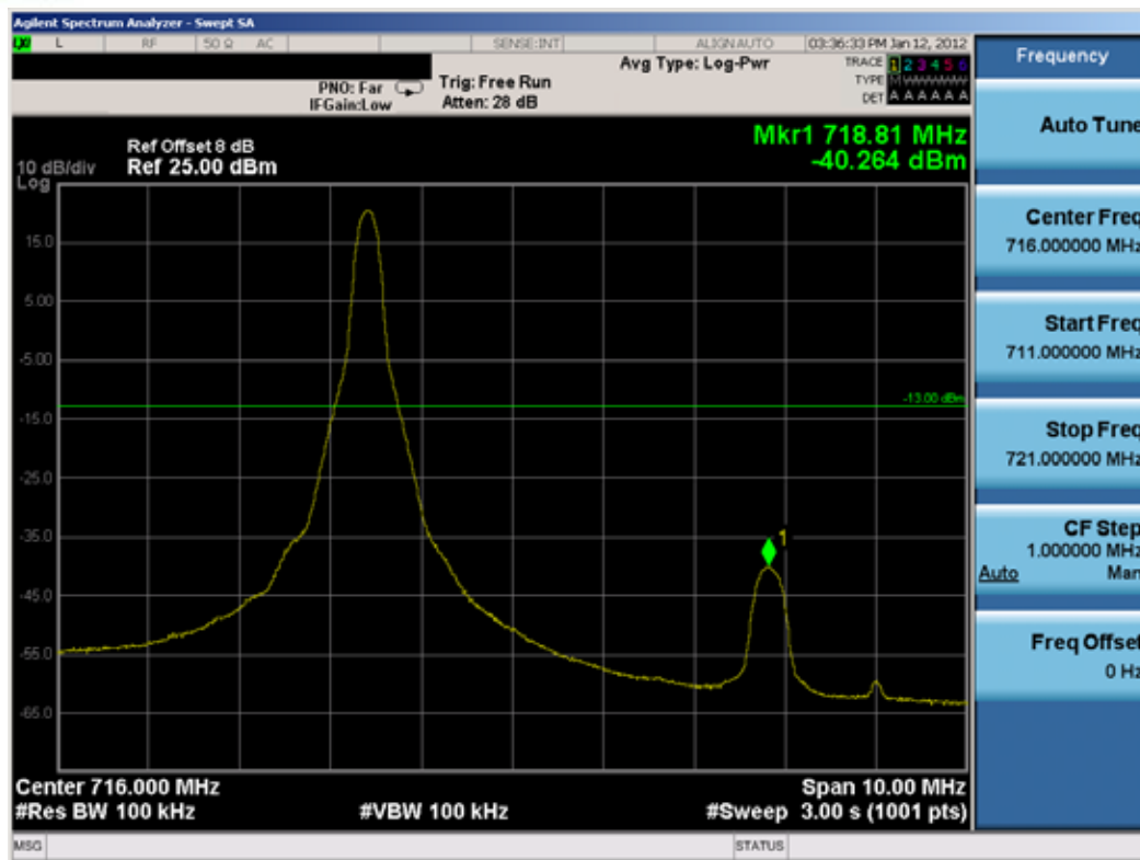
Plot 7-12. Upper Band Edge Plot (10MHz BW, QPSK RB Size = 1, Offset = 49)
