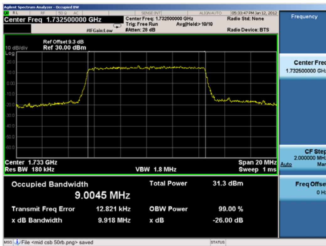
Plot 8-15. Occupied Bandwidth Plot (10MHz BW, QPSK RB Size = 50 Offset = 0)
