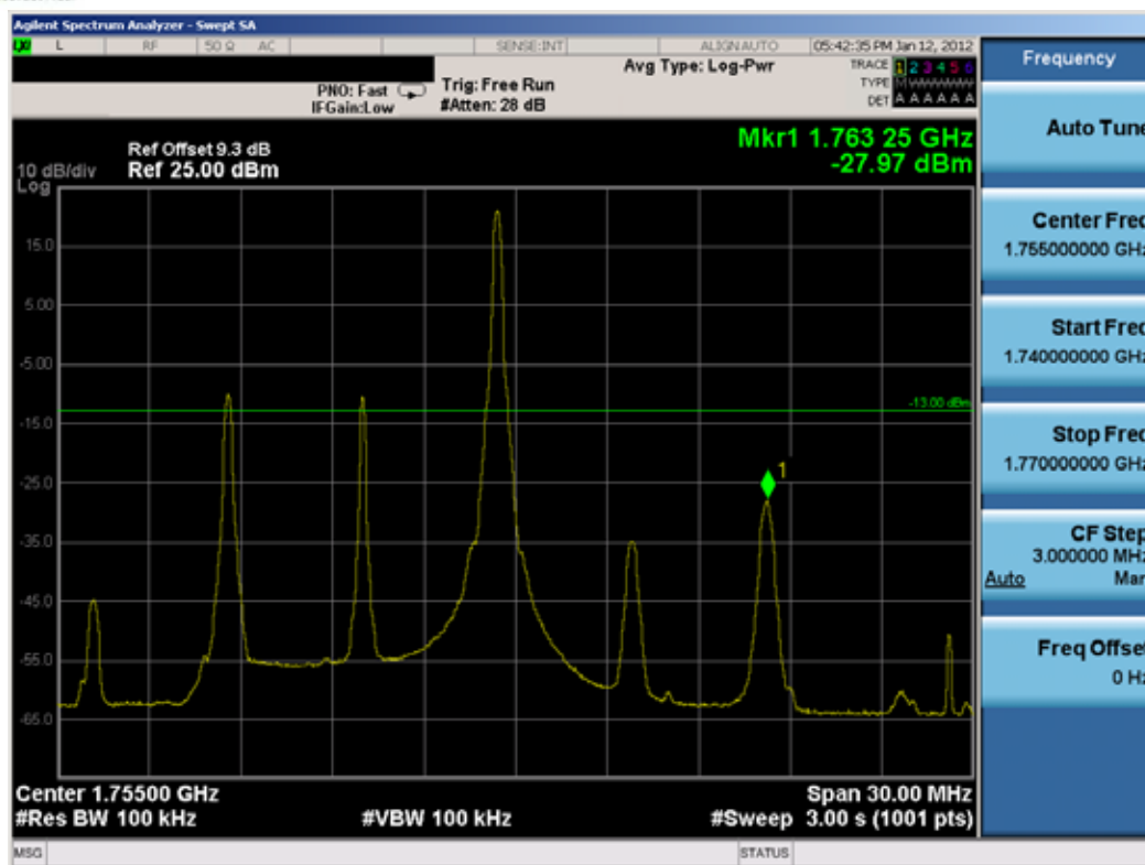
Plot 8-24. Band Edge Plot (10MHz BW, QPSK RB Size = 1 Offset = 49, High Channel)
