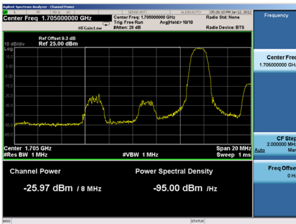
Plot 8-11. Extended Band Edge Plot (10MHz BW, QPSK RB Size = 1 Offset = 0, Low Channel)
