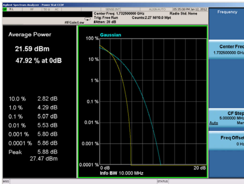
Plot 8-20. Peak-Average Ratio Plot (10MHz BW, 16QAM RB Size = 50 RB Offset = 0)
