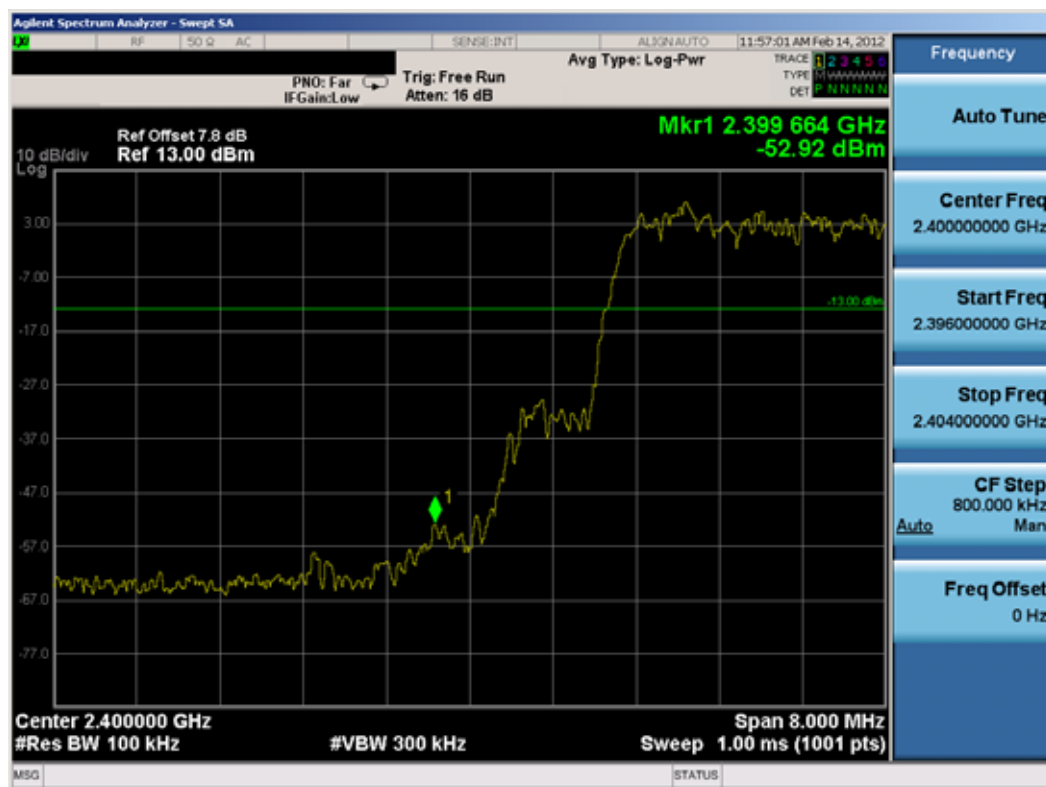
Plot 6-12. Lower Band Edge Plot (Bluetooth, 3Mbps, Hopping)
