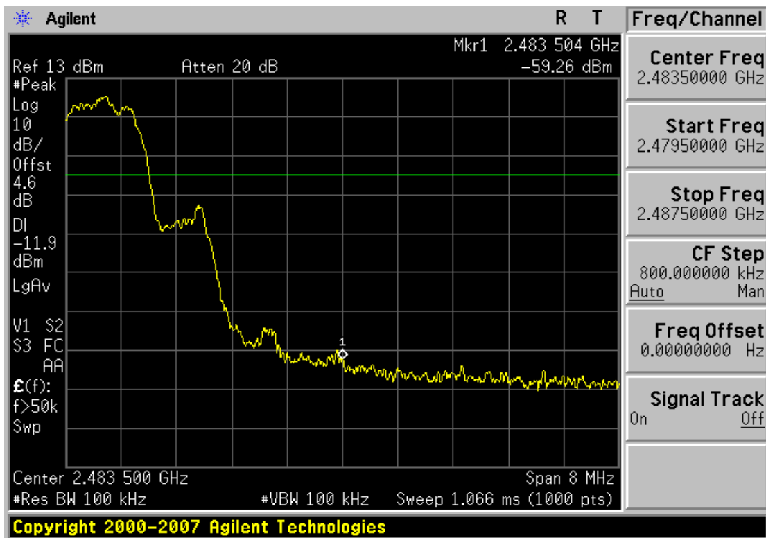
Plot 6-11. Band Edge Plot (Bluetooth, 3Mbps – Ch. 78)
