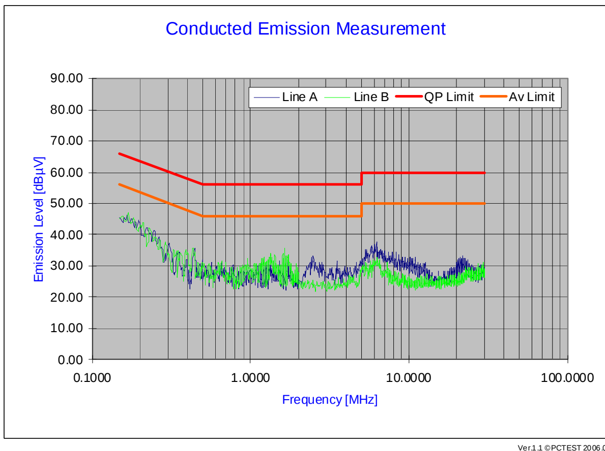
Plot 6-24. Line Conducted Plot with Bluetooth
