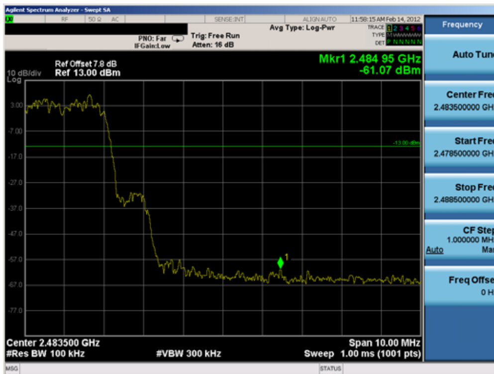
Plot 6-13. Upper Band Edge Plot (Bluetooth, 3Mbps, Hopping)
