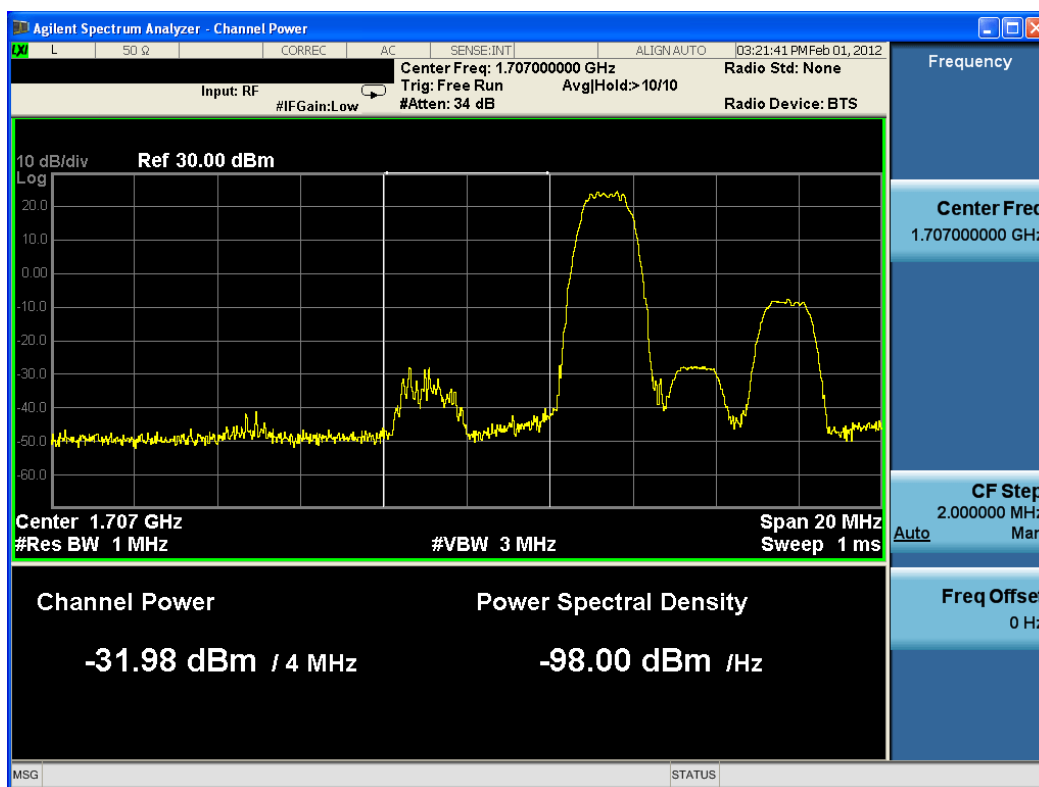
Plot 8-13. Extended Band Edge Plot (5MHz BW, QPSK RB Size = 1 Offset = 0)
