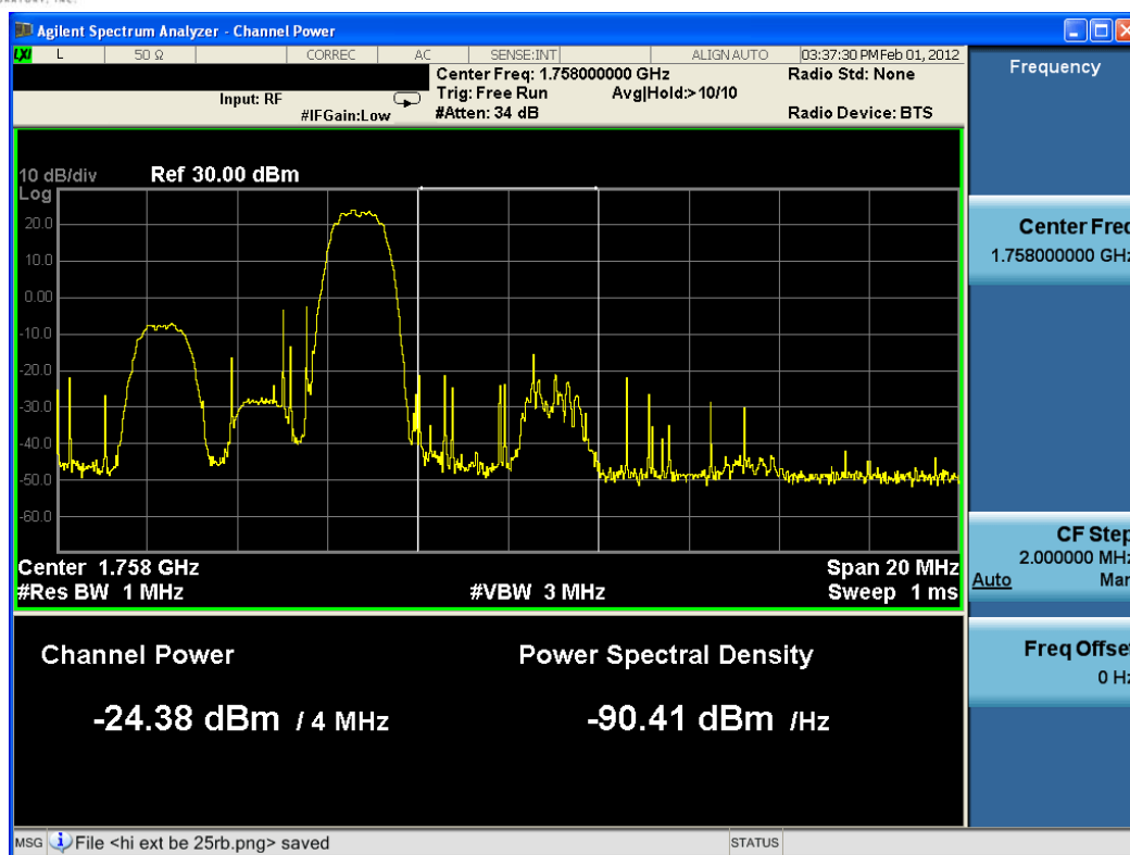
Plot 8-30. Extended Band Edge Plot (5MHz BW, QPSK RB Size = 1 Offset = 24, High Channel)
