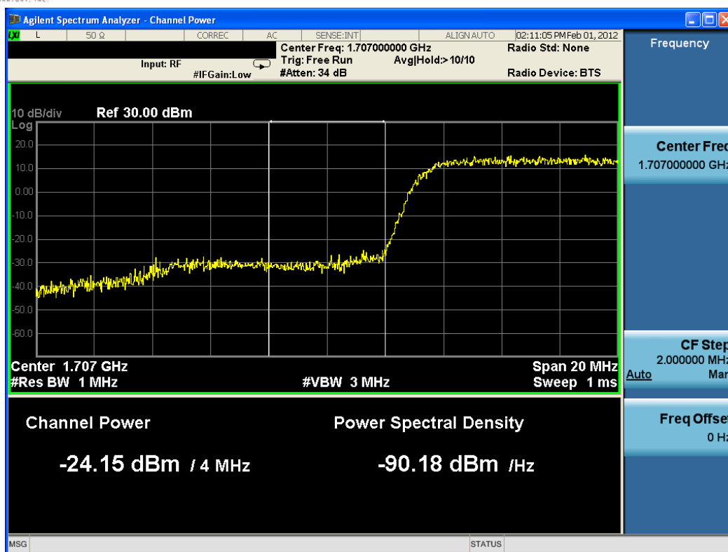
Plot 8-12. Extended Band Edge Plot (10MHz BW, QPSK RB Size = 50 Offset = 0)
