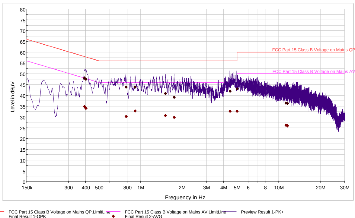
Plot 6-31. Line Conducted Plot with 802.11b (L1)
