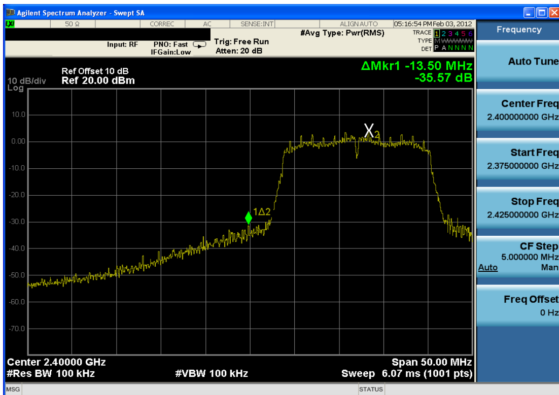
Plot 6-21. Band Edge Plot (802.11g – Ch. 1)
