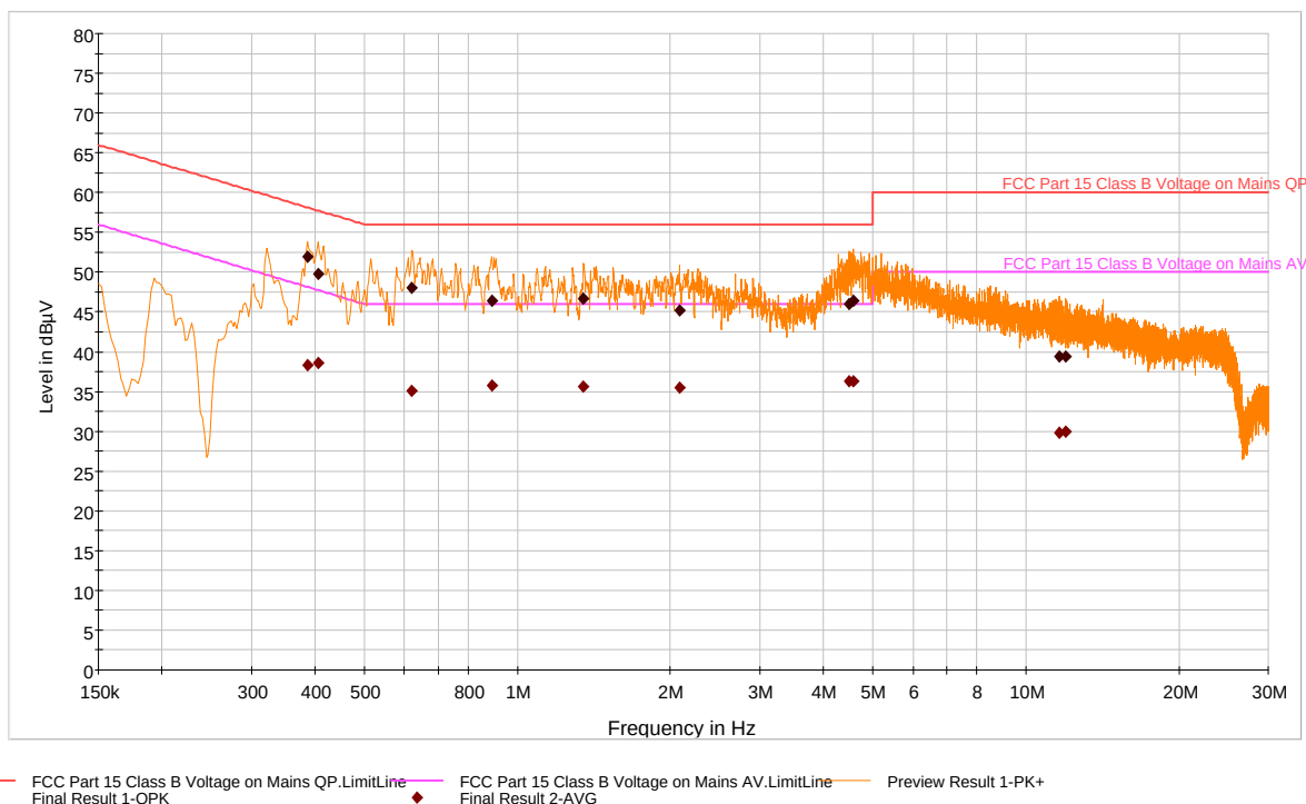
Plot 6-32. Line Conducted Plot with 802.11b (LN)
