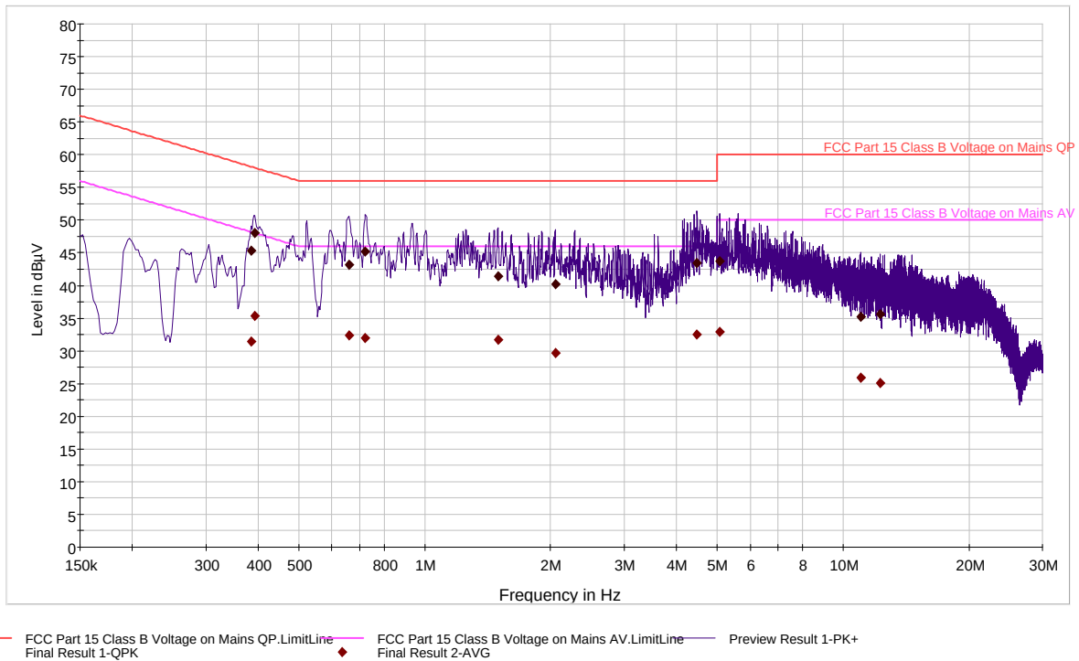
Plot 6-24. Line Conducted Plot with Bluetooth (Line 1)
