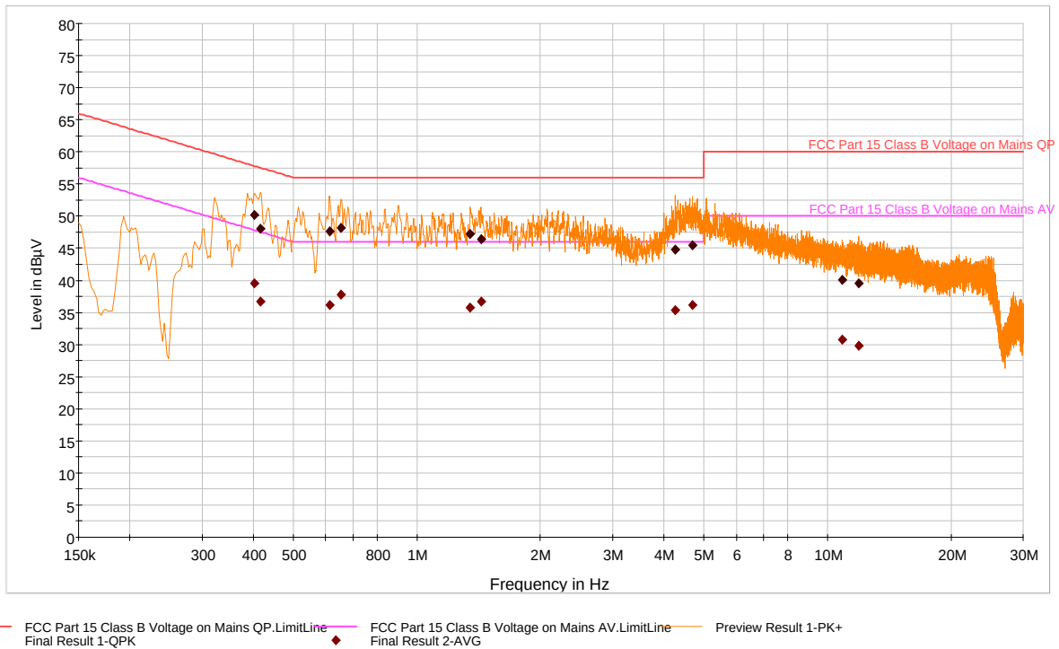
Plot 6-25. Line Conducted Plot with Bluetooth (Line N)
