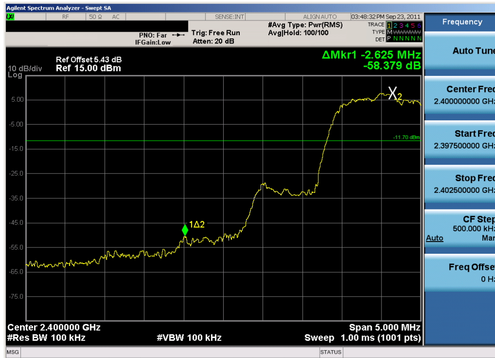
Plot 6-10. Band Edge Plot (Bluetooth, 3Mbps - Ch. 0)
