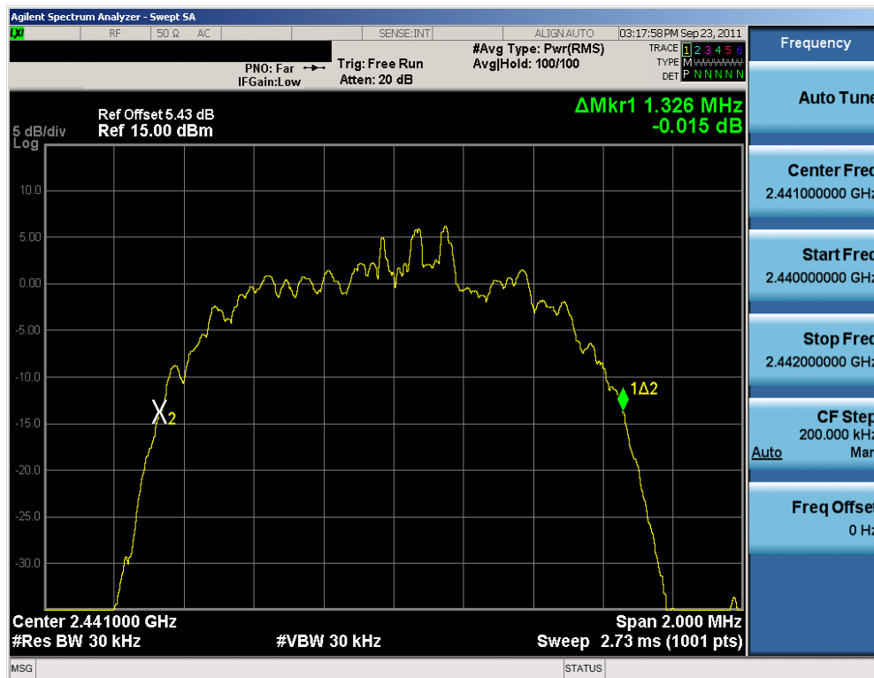
Plot 6-8. 20dB Bandwidth Plot (Bluetooth, 3Mbps – Ch. 39)
