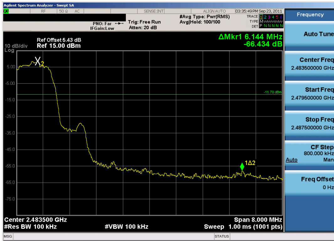
Plot 6-11. Band Edge Plot (Bluetooth, 3Mbps – Ch. 78)
