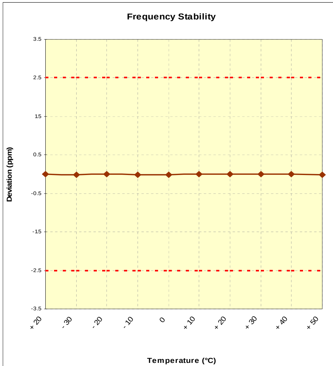
Figure 6-3. Frequency Stability Graph (PCS GSM Mode – Ch. 661)
