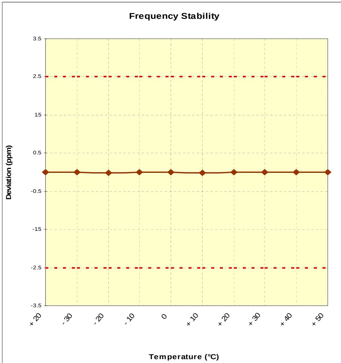
Figure 6-4. Frequency Stability Graph (PCS WCDMA Mode – Ch. 9400)
