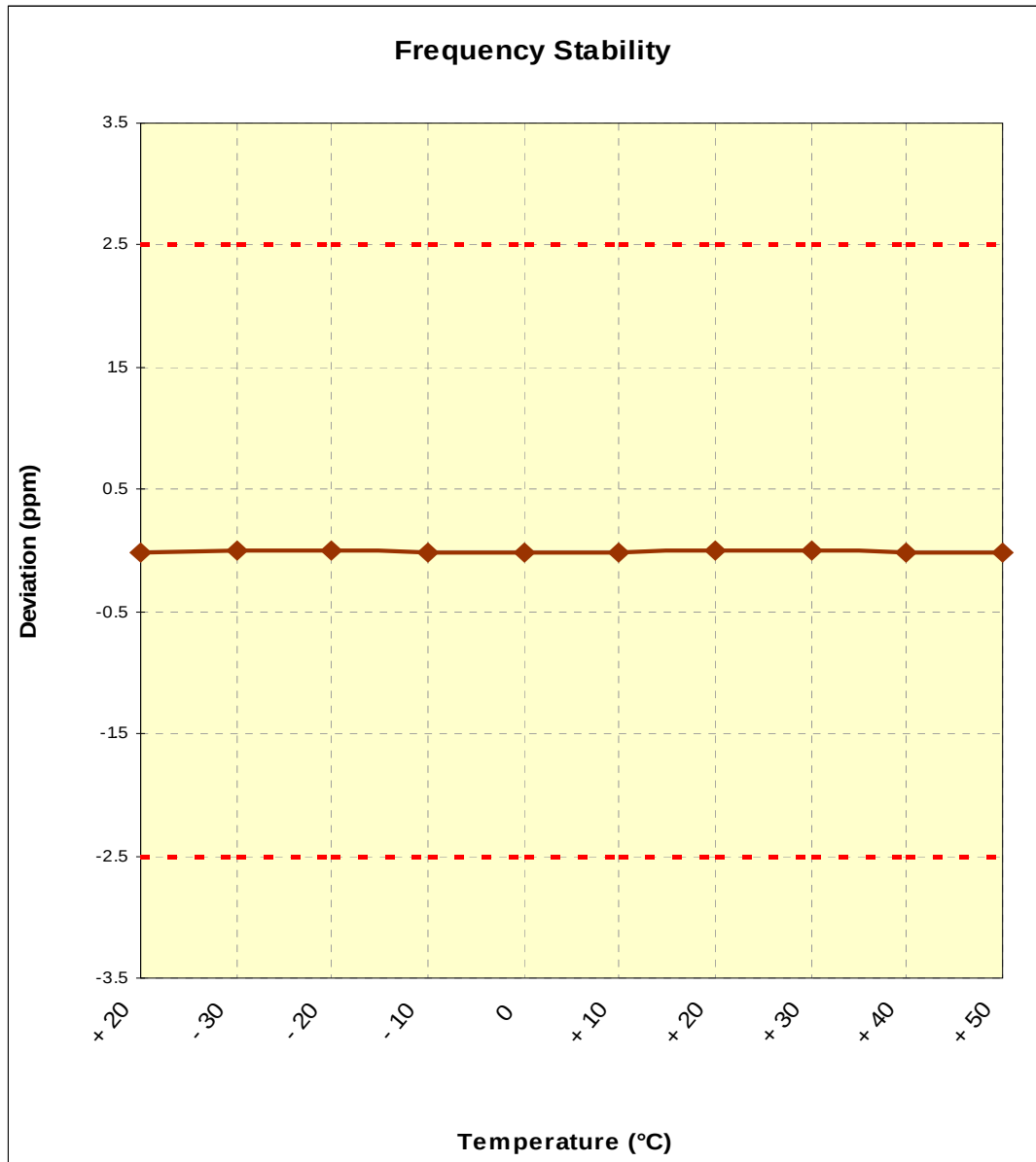
Figure 6-1. Frequency Stability Graph (Cellular GSM Mode – Ch. 190)
