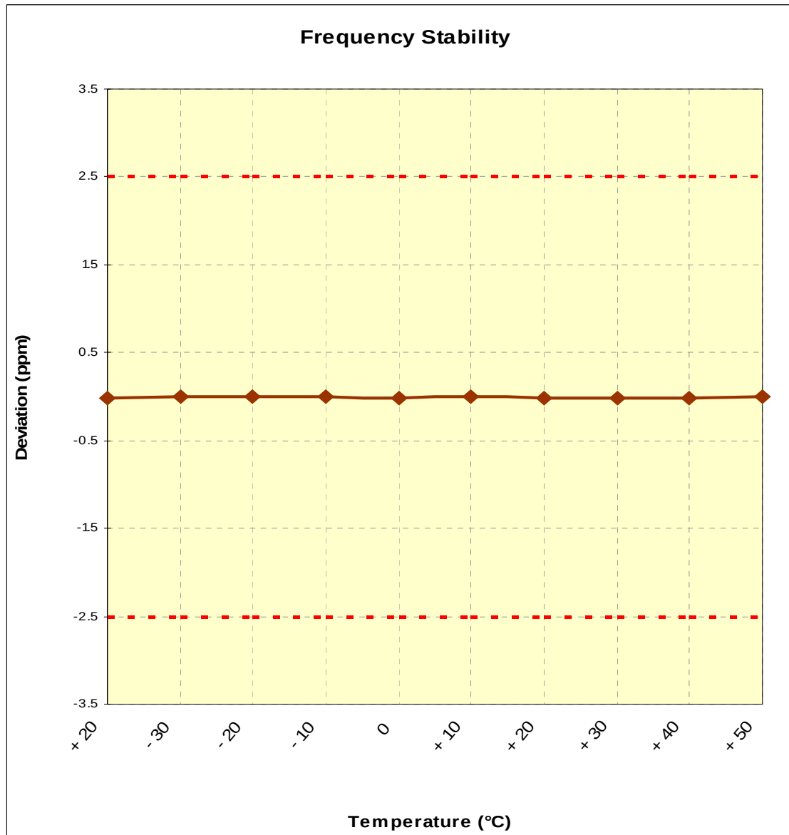
Figure 6-2. Frequency Stability Graph (Cellular WCDMA Mode – Ch. 4183)
