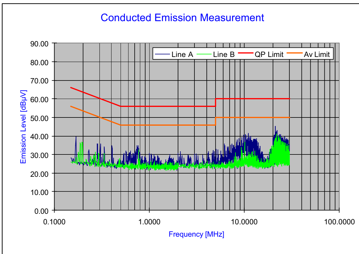
Plot 6-25. Line Conducted Plot with 802.11n
