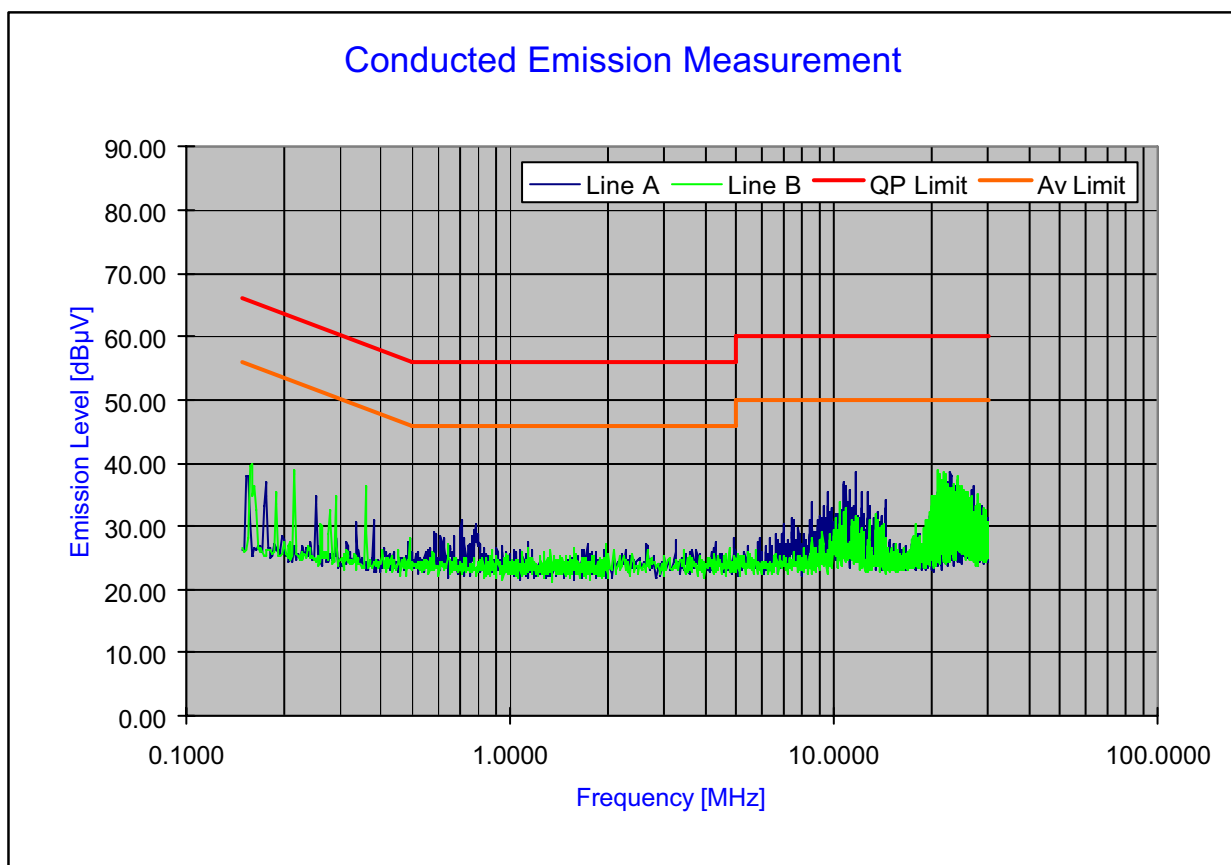
Plot 6-8. Line Conducted Plot with 802.11g
