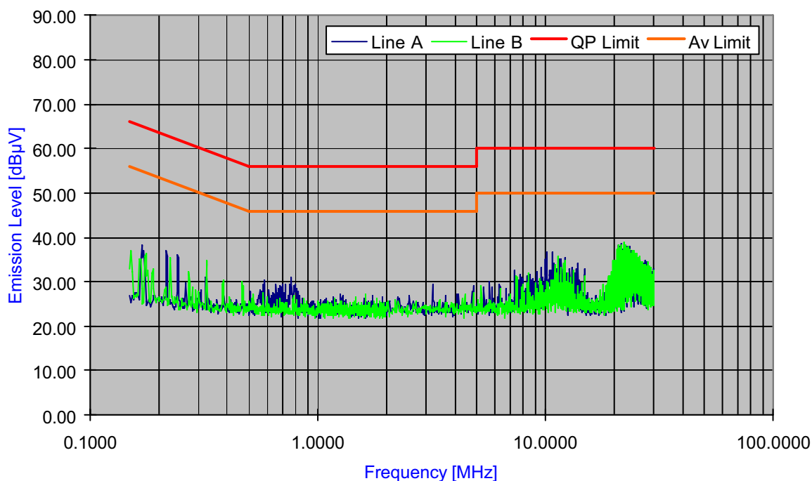
Plot 6-7. Line Conducted Plot with 802.11b
