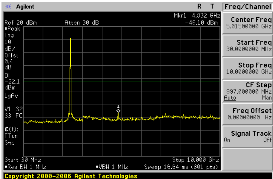
Plot 6-25. Conducted Spurious Plot (802.11b – Ch. 1)
