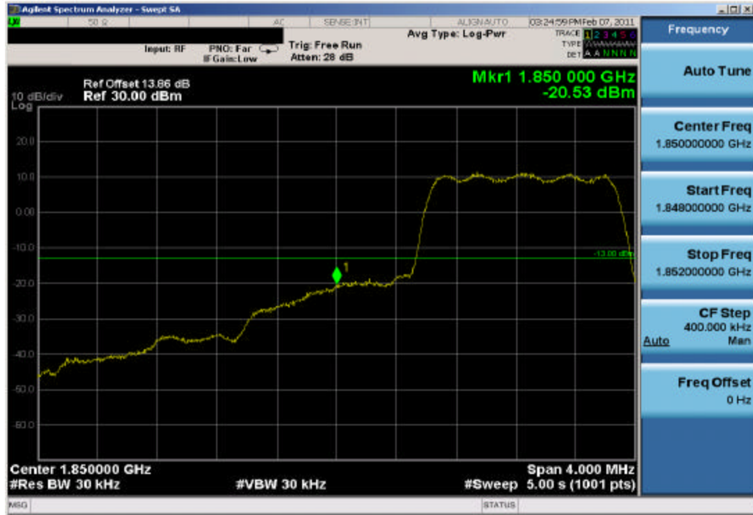
Plot 7-59. Band Edge Plot (PCS CDMA Mode – Ch. 25)
