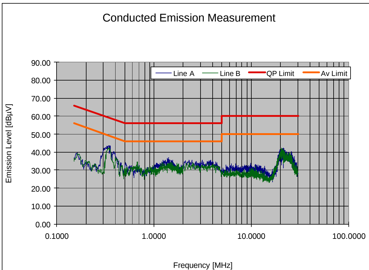
Plot 6-32. Line Conducted Plot with 802.11g
